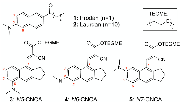
Figure 1. Chemical structures of Prodan (1), Laurdan (2), and cyclopenta[ b ]naphthalene cyanoacrylate (CNCA) dyes (3-5).
