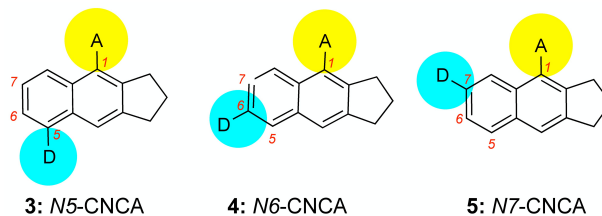
Figure 4: Comparison of the relative position of donor (D, Me 2 N) and acceptor (A, CH=C(CN)CO 2 TEGME) substituents in CNCA dyes. Placing the D and A groups in close proximity decreases their rotational ability thereby allowing emission from the planar excited state.
