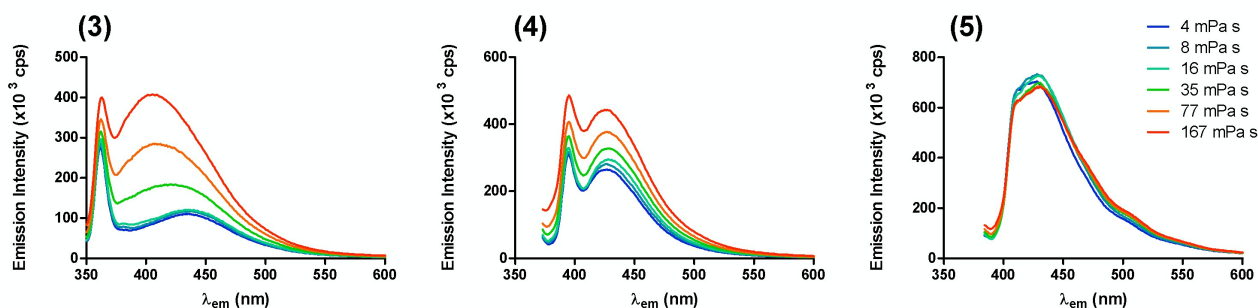
Figure 2: Emission spectra of 3 , 4 , and 5 in alcohol mixtures of different viscosity. While 5 shows no major change in the different alcohol mixtures, 4 and notably 3 exhibit increased peak emission from the red-shifted band in alcohols with higher viscosity.
