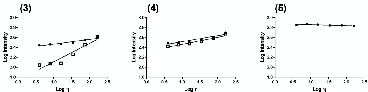
Figure 3: Peak emission intensity plotted over solvent viscosity in a double-logarithmic scale. Compounds 3 and 4 have significantly positive slopes, and the slope can be used as an indication of the sensitivity towards viscosity. The slope of 5 is not significantly different from zero. Circles indicate the blue-shifted band (and the single emission of 5 ) and open squares indicate the red-shifted band.
