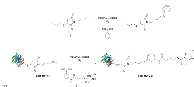
Scheme 1. Oxidative Heck reactions between terminal alkenes and arylboronic acids.
