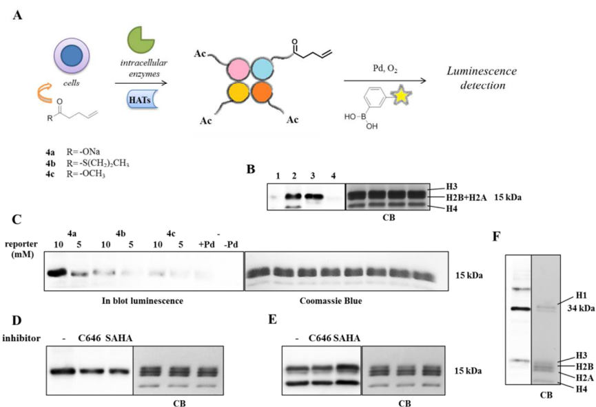
Fig. 2. A) Schematic procedure of alkene metabolic labeling and subsequent detection of histones via the oxidative Heck reaction using 3-(biotinylamino)phenylboronic acid 1 . B) On blot luminescence imaging and Coomassie Blue staining of biotinylated alkyne-labeled and alkene-labeled histones (7.0 \mu g) via 2) 'click' and 3) oxidative Heck reaction accordingly. Reactions 1) and 4) negative controls for 'click' and oxidative Heck reaction accordingly. C) On blot luminescence imaging and Coomassie Blue staining of histones (5.5 \mu g) after 6 h incubation with 5 and 10 mM of 4a sodium pent-4-enoate, 4b S -propyl pent-4-enthioate and 4c methyl 4-pentenoate. D) On blot luminescence imaging and Coomassie Blue staining of alkenylated histones (4.0 \mu g) after 14 h incubation with 30 \mu M of C646 and 0.41 \mu M of SAHA followed by treatment with 10 mM of the reporter 4a . E) On blot luminescence detection and Coomassie Blue staining of acetylated histones (3.0 \mu g) after 20 h incubation with 30 \mu M of C646 and 0.41 \mu M of SAHA using the Anti-Acetyl lysine antibody. F) On blot luminescence imaging and Coomassie Blue staining of alkenylated histones H1 and H3 (1.0 \mu g) after separation on 15% SDS-PAGE.
