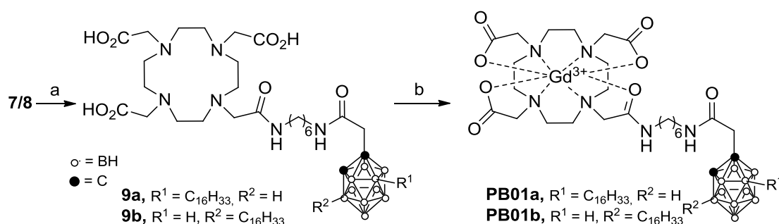
Scheme 3 Synthesis of \text{Gd}^{3+} - \text{C}-[(\text{COOH})_3\text{DOTAMA}-\text{C}_6] -acetamido- \text{C}'\text{-H-4} -(hexadecyl)- ortho -carborane ( PB01a ) and \text{Gd}^{3+} - \text{C}-[(\text{COOH})_3\text{DOTAMA}-\text{C}_6] -acetamido- \text{C}'\text{-H-9} -(hexadecyl)- ortho -carborane ( PB01b ). Reaction conditions and yields: a) \text{CF}_3\text{COOH} , \text{CH}_2\text{Cl}_2 , r. t., (>99% for both 9a and 9b ); or \text{H}_2 , Pd/C, EtOH, \text{CH}_2\text{Cl}_2 , rt (>99% for both 9a and 9b ); b) \text{GdCl}_3 , \text{H}_2\text{O} (>99% for both PB01a and PB01b ).
