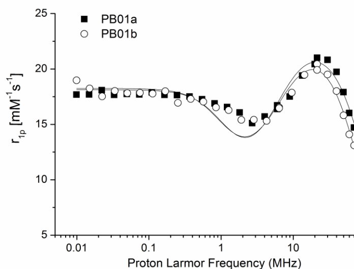
Figure 3 Nuclear Magnetic Relaxometric Dispersion (NMRD) profiles (0.01–70 MHz; pH 7, 25°C) of PB01a and PB01b derivatives. The solid curves through the data points are calculated with the parameters reported in the Table 1.
