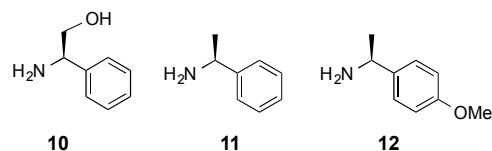
Figure 1 The chiral auxiliaries amine reagents used in the Strecker synthesis strategy.
