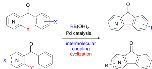
Scheme 1 Possible syntheses of substituted azafluorenones using palladium-catalyzed tandem reactions.
