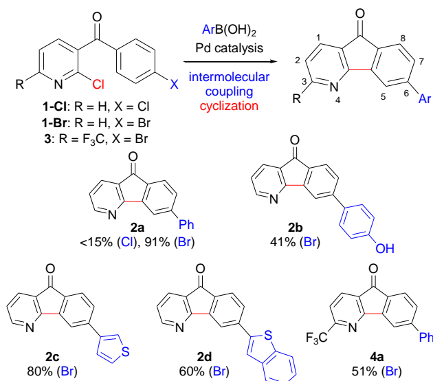
Scheme 2 Palladium-catalyzed Suzuki coupling-intramolecular arylation from the dihalides 1 and 3 . Reaction conditions: Pd(OAc) 2 (5 mol %), Cy 3 P·HBF 4 (10 mol %), K 2 CO 3 (2 equiv), DMF, 130 °C, 24 h.
