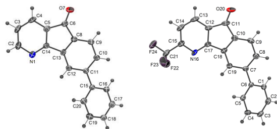
Figure 1 ORTEP diagrams (50% probability) of 2a and 4a .
