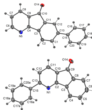
Figure 2 ORTEP diagrams (50% probability) of 6a and 9a .
