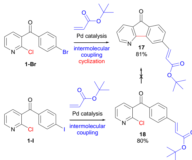
Scheme 6 Palladium-catalyzed Heck coupling-intramolecular arylation attempted from the dihalides 1-Br and 1-I . Reaction conditions: Pd(OAc) 2 (5 mol %), Cy 3 P·HBF 4 (10 mol %), K 2 CO 3 (2 equiv), DMF, 130 °C, 24 h.
