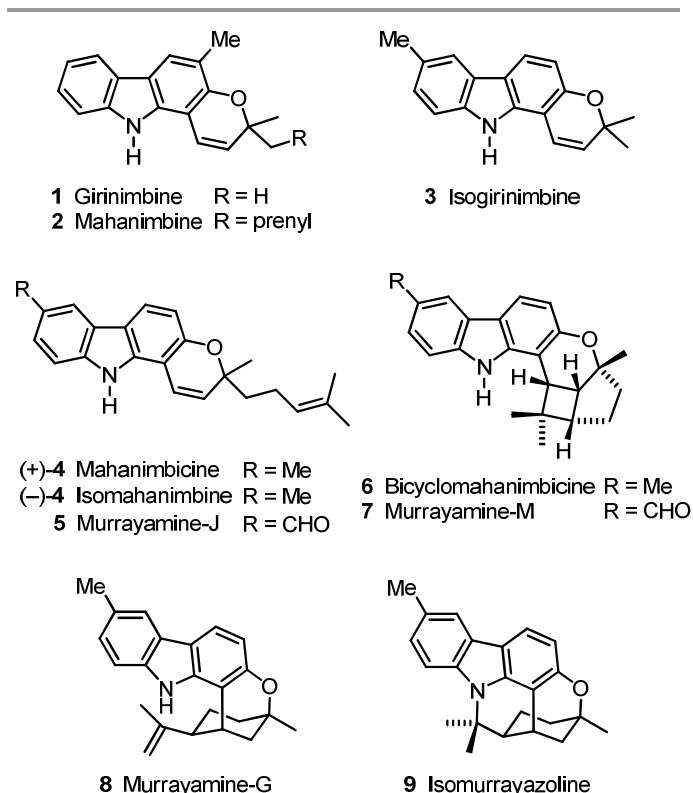
Fig. 1 Naturally occurring pyrano[3,2- a ]carbazole alkaloids 1–9.
