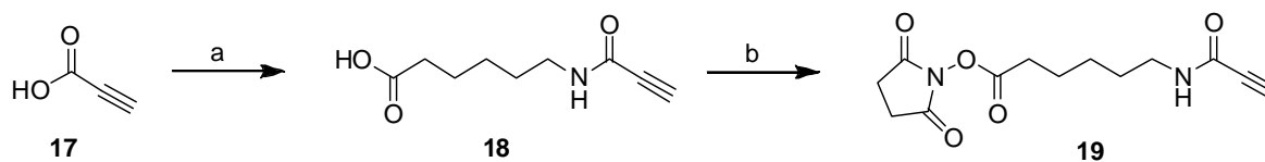
Scheme 6. Synthesis of the alkyne carboxylic acid succinimidyl ester 19 . a: 6-aminocaproic
