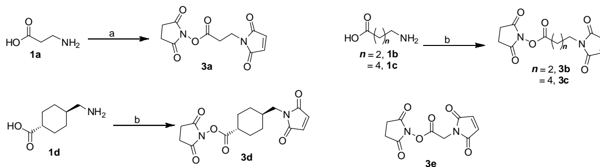
Scheme 1. Synthesis of the N -maleoyl amino acid succinimidyl esters ( 3 ). Synthesis of 3e
