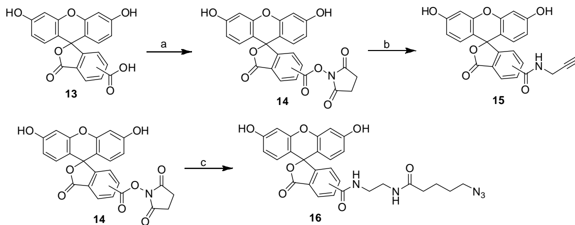
Scheme 5. Synthesis of the alkyne ( 15 ) and azido ( 16 ) derivatives of fluorescein. a: NHS,
