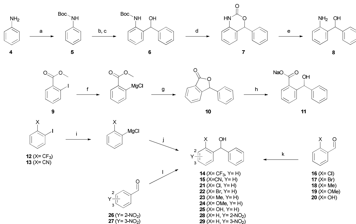
Scheme 1 Synthesis of compounds 8 , 11 , 14-15 , 21-25 and 28-29 . Reagents and conditions: (a) Boc 2 O, THF, reflux, 38%; (b) t BuLi, THF, -60°C; (c) benzaldehyde, THF, -20°C, 35% (2 steps); (d) TFA, DCM, 0°C - room temp, 78%; (e) KOH, MeOH/H 2 O, reflux, 17%; (f) i PrMgCl, THF, -40°C; (g) benzaldehyde, THF, -40°C, 63% (2 steps); (h) NaOH, MeOH/H 2 O, 50°C, 39%; (i) i PrMgCl, THF, -40°C; (j) benzaldehyde, THF, -40°C, 47-71% (2 steps); (k) PhMgCl, THF, 0-50°C, 36-92%; (l) PhMgCl, THF, -40°C, 7-12%.
