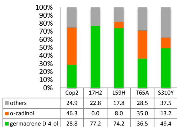
Figure 1 Product distribution in % of Cop2, the triple mutant 17H2 and the single mutants L59H, T65A and S310Y analyzed by GC.
