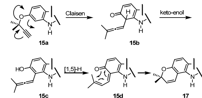
Scheme 4 Mechanism for annulation of the pyran ring. 19
