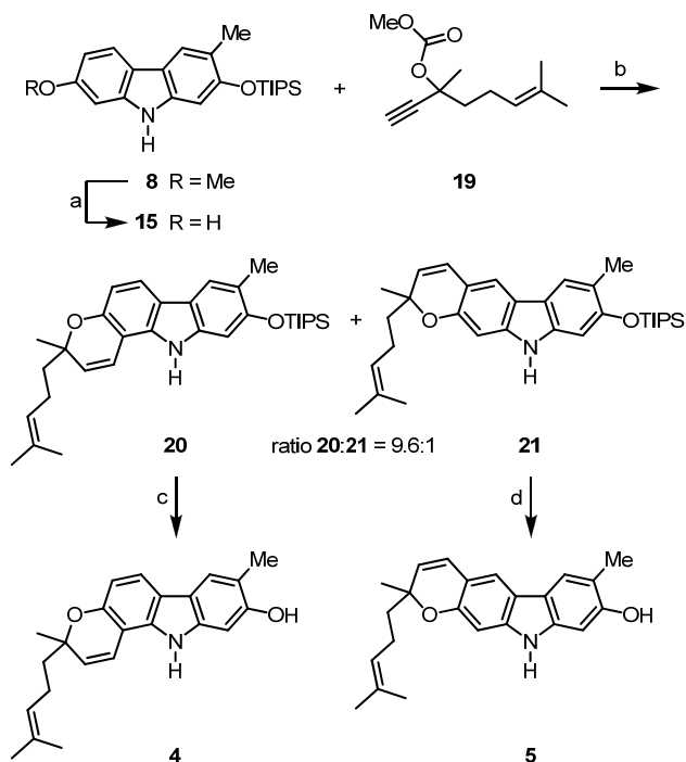
Scheme 5 Synthesis of pyrayafoline D ( 4 ) and E ( 5 ). Reagents and conditions: (a) 2.0 equiv. \text{BBr}_3 , \text{CH}_2\text{Cl}_2 , -78^\circ\text{C} to rt; (b) 1. 2.0 equiv. 19 , 2.0 equiv. DBU, 0.5 mol% \text{CuCl}_2 \cdot 2\text{H}_2\text{O} , MeCN, rt; 2. PhMe, reflux, 49% 20 and 4% 21 (three steps); (c) 1.5 equiv. TBAF, DMF, -5^\circ\text{C} , 100%; (d) 1.5 equiv. TBAF, DMF, -12^\circ\text{C} , 83%.
