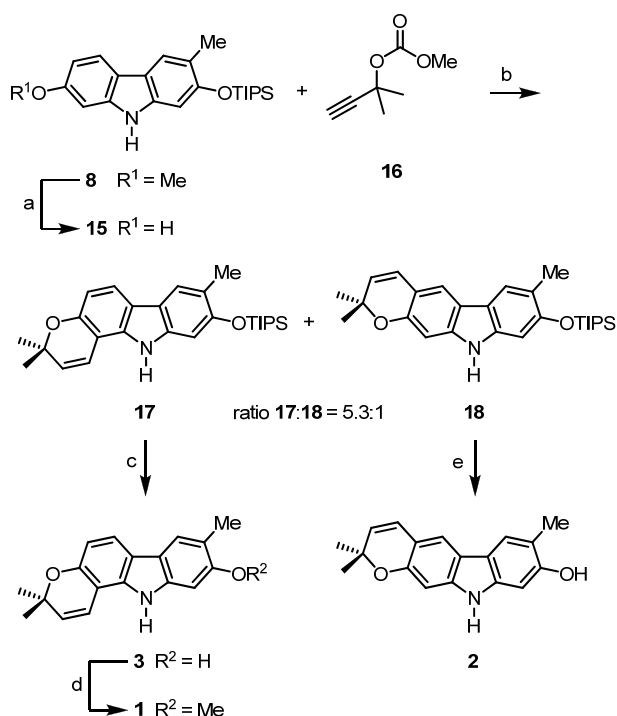
Scheme 4 Mechanism for annulation of the pyran ring. 19
