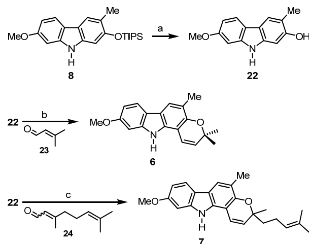
Scheme 6 Synthesis of O -methylmurrayamine A ( 6 ) and O -methylmahanine ( 7 ). Reagents and conditions: (a) 1.5 equiv. TBAF, DMF, -10^\circ\text{C} to rt, 100%; (b) 2.0 equiv. prenal ( 23 ), 4.0 equiv. \text{Ti}(\text{OiPr})_4 , PhMe, -78^\circ\text{C} to rt, 88%; (c) 2.0 equiv. citral ( 24 ), 4.0 equiv. \text{Ti}(\text{OiPr})_4 , PhMe, -78^\circ\text{C} to rt, 75%.
