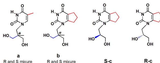
Fig. 2 Acyclic nucleosides mimicking thymine residue. The pro-chiral carbon of a and b is labelled with #.
