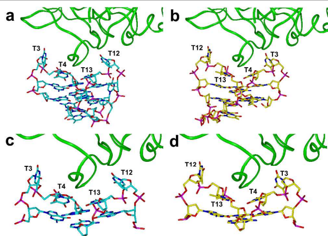
Fig. 8 X-ray structures of the complex between TBA and human \alpha -thrombin presenting aptamer TT loops interacting with thrombin ABE I. (a) and (c): binding mode III; PDB structure 1HAO (TBA carbons = cyan). (b) and (d): binding mode IV; PDB structure 4DIH (TBA carbons = yellow). Heteroatoms are coloured as follows: O = red; N = blue; P = magenta. Thrombin ABE I is shown as green ribbon.
