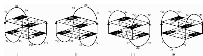
Fig. 3 Schematic representation of the four possible orientations of TBA with respect to thrombin assuming the same strand polarity of the X-ray complex. White and black rectangles indicate G bases in anti and syn conformation, respectively.
