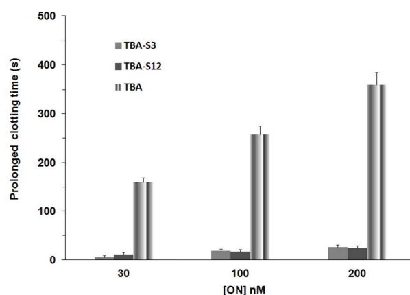
Fig. 7 Prolonged fibrinogen clotting time (s) in presence of TBA, TBA-S 3 , or TBA-S 12 at different concentrations (30-200 nM). The graphics were drawn from scattering curves data.
