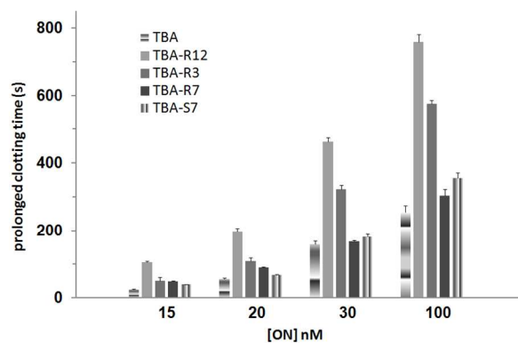
Fig. 6 Prolonged fibrinogen clotting time (s) in presence of TBA or each active aptamer at different concentrations (15-100 nM). The graphics were drawn from scattering curves data.
