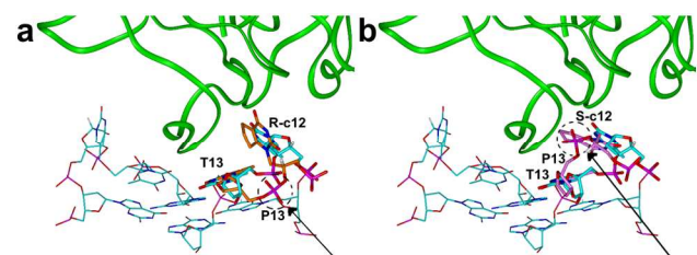
Fig. 9 (a) TBA-R 12 (carbons = orange) and (b) TBA-S 12 (carbons = pink) superimposed on the bioactive conformation of TBA in complex with thrombin (carbons = cyan; PDB ID: 1HAO). Heteroatoms are coloured as follows: O = red; N = blue; P = magenta. Thrombin ABE I is shown as green ribbon. Hydrogens are omitted with the exception of those present on the modified residue chiral carbon (R-c12 and S-c12) and on TBA T12 C4'. The position of P13 is highlighted by a dashed circle and an arrow.
