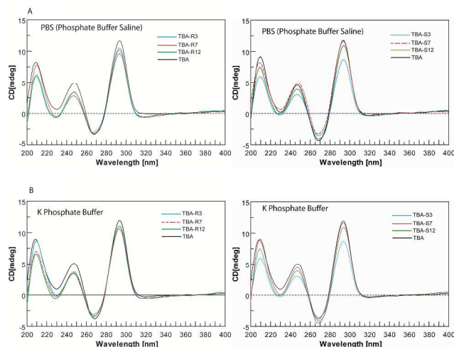
Fig. 5 CD spectra of TBA and modified ONs in PBS (A) and K + phosphate buffer (B).
