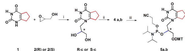
Scheme 1 Synthesis of monomers 5a,b . i) 1 1.0 g (6.6 mmol), 2 (pure enantiomer R or S ) 0.490 g (6.6 mmol), potassium carbonate 0.152 g (1.1 mmol), dry DMF (24 mL), 12–18 h, 80 °C, yields R-c 60% and S-c 45%; ii) R-c or S-c 560 mg (2.5 mmol), 4,4'-dimethoxytrytylchloride 850 mg (2.5 mmol), 4-dimethylaminopyridine 15 mg (0.12 mmol), pyridine (20 mL), 2.0 h, r.t., yields 85%; iii) 4a,b 859 mg, (1.6 mmol), 2-cyanoethyl-diisopropylchlorophosphoramidite 536 \mu\text{L} (2.4 mmol), DIPEA 1.7 mL (10 mmol), DCM (9 mL), 40 min, r.t., yields 90%.
