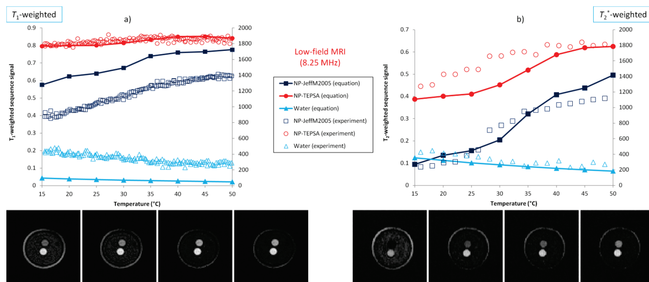
Fig. 7 Images taken on the low-field MRI scanner (8.25 MHz, 0.194 T) at increasing temperatures from 15 to 50°C with a) the T_1 -weighted sequence ( TR=100\text{ms} TE=2.8\text{ms} flip angle = 70^\circ ) and b) the T_2^* -weighted sequence ( TR=300\text{ms} TE=12\text{ms} ), 160\times 160\text{ mm}^2 field of view, 128\times 128 matrix, 7 mm slice thickness. The external light grey circle was ascribed to a perfusion MRI contrast of the water circulating in the double-wall of the glass chamber (diameter 50 mm) as compared to water at rest inside the chamber (dark grey). The tube at the upper position was filled with Jeffamine ® M-2005 grafted USPIOs (1.1 \text{mM}_{\text{Fe}} ) and the tube at the bottom position with the TEPSA-coated control (0.8 \text{mM}_{\text{Fe}} ). The USPIOs exhibited a positive contrast (signal above the level of pure water) on all MR images except with the T_2^* -weighting (b) for the USPIOs grafted with the chains below their LCST (15–25°C). The open markers show experimental signals. The closed markers and the solid lines represent theoretical predictions using Eq. (5) with the experimental values of T_1 , T_2^* , TE and TR . In the case of the Jeffamine ® M-2005 grafted USPIOs, a linear regression of the experimental signal (normalised to the initial value at 15°C) versus temperature leads to slopes of +1.9%/°C and +16.6%/°C respectively for the T_1 - and the T_2^* -weighted sequences, with correlation coefficients R=0.98 and R=0.97 , respectively. MRI cross-sections at the bottom line illustrate the variations of the signal plotted on the curves.
