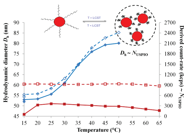
Fig. 4 Intensity-average hydrodynamic diameter D_h (nm, filled markers, solid lines) and derived count-rate in DLS (empty markers, dotted lines) vs. temperature for USPIOs grafted with Jeffamine ® M-2005 (blue) and M-2070 (red). The measurements were performed at 1 mM Fe in water.
