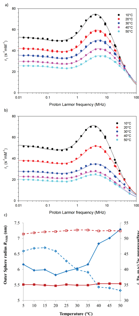
Fig. 5 NMRD profiles of the longitudinal relaxivity vs. Larmor frequency for a) TEPSA-coated USPIOs, and b) USPIOs grafted with Jeffamine ® M-2005 ; c) relaxometric radius R_{\text{NMR}} (nm, filled markers, solid lines) and saturation magnetisation M_S (empty markers, dotted lines) vs. temperature for USPIOs coated by Jeffamine ® M-2005 (blue) and TEPSA only (red).
