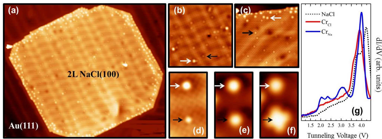
Figure 1. (a) 53 \times 44 \text{ nm}^2 STM topography image ( V = 1 \text{ V} , I = 0.05 \text{ nA} ) of Cr atoms on 2L NaCl/Au(111). (b) 15 \times 15 \text{ nm}^2 STM topography image ( V = 1 \text{ V} , I = 0.05 \text{ nA} ) taken in the center of the NaCl island in (a). (c) 15 \times 15 \text{ nm}^2 atomic-resolution STM topography image ( V = 1 \text{ V} , I = 0.05 \text{ nA} ) taken near the edge of another 2L NaCl island. The obviously brighter protrusions indicated by white arrows are \text{Cr}_{\text{Cl}} atoms, while the weaker protrusions indicated by black arrows are \text{Cr}_{\text{Na}} atoms. (d)-(f) 2.8 \times 4.8 \text{ nm}^2 STM topography images of a \text{Cr}_{\text{Cl}} atom and a \text{Cr}_{\text{Na}} atom taken at +2.0 \text{ V} , +2.4 \text{ V} , and +3.1 \text{ V} , respectively. (g) dI/dV spectra recorded at \text{Cr}_{\text{Cl}} , \text{Cr}_{\text{Na}} and the surrounding NaCl.
