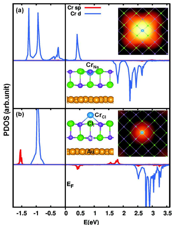
Figure 2. Projected density of states (PDOS) of 2L NaCl/Au(111) films with Cr substituting Na (a) and Cl (b), respectively. See Fig. S4 and S5 in SI for the decomposition of Cr 3d and 4sp orbitals. Structures and simulated STM images are presented in the insets.
