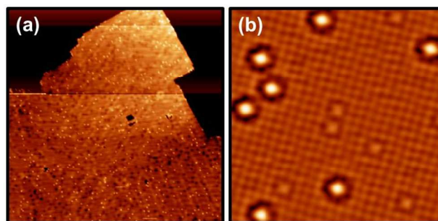
Figure 4. (a) 100 \times 100 nm 2 STM topography image ( V = 1 V, I = 0.02 nA) of Cr atoms on 3L NaCl/Au(111). Cr doping concentration is around 1%. (b) 10 \times 10 nm 2 Fourier-filtered STM topography image ( V = 1 V, I = 0.05 nA) taken in the middle of a 3L NaCl island.
