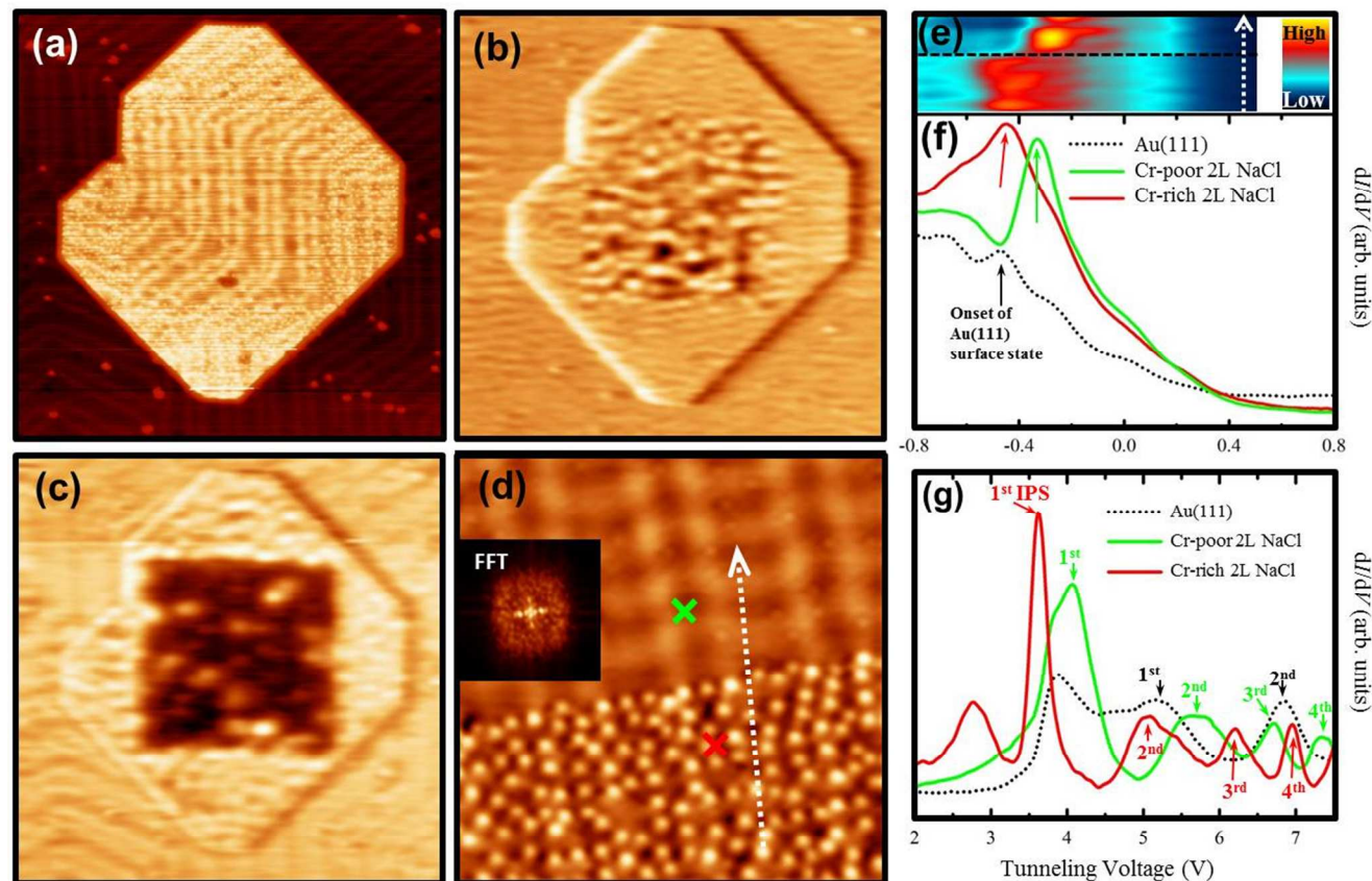
Figure 3. (a) 80 \times 80 \text{ nm}^2 STM topography image of Cr atoms on 2L NaCl/Au(111) and the corresponding LDOS maps taken at (b) V = -0.2 \text{ V} , I = 0.05 \text{ nA} and (c) V = -0.4 \text{ V} , I = 0.1 \text{ nA} . (d) 21 \times 21 \text{ nm}^2 STM topography image ( V = 0.6 \text{ V} , I = 0.1 \text{ nA} ) taken near the edge of another 2L NaCl island. The inset is a 4 \text{ nm}^{-1} \times 4 \text{ nm}^{-1} fast Fourier transform (FFT) pattern of the Cr-rich region. (e) 1.3 \text{ V} \times 12 \text{ nm} color visualization of (dI/dV)(V) spectra taken along the dotted white arrow indicated in (d). The horizontal black dashed line in (e) indicates the boundary between the Cr-rich and Cr-poor region. (f) and (g) dI/dV spectra taken on the clean Au(111) surface, the Cr-rich region [near the red cross in (d)], and the Cr-poor region [near the green cross in (d)] of the 2L NaCl island in the -0.8 to 0.8 \text{ eV} and 2 to 7 \text{ eV} ranges, respectively. The arrows in (f) mark the onset of the interface state for Cr-poor and Cr-rich regions. The arrows in (g) mark the positions of the image-potential states (IPSS).
