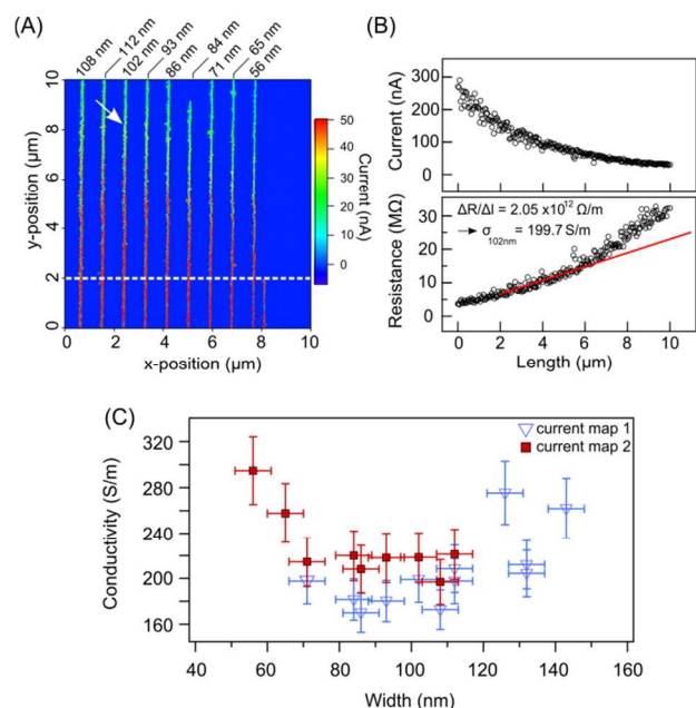
Fig. 2 (A) Typical conductivity map ( 10 \times 10 \mu\text{m}^2 ) of Ppy belts on a \text{SiO}_2 substrate (bias voltage of 1 V). The measured width of the nanobelts decreases from 112 nm to 56 nm as indicated. All belts have an average height of 25 nm. (B) Local current, I , (top) and resistance, R , (bottom) vs. length of a single nanobelt. The local resistance was determined from the measured current data via Ohm's law. The line shows a linear fit to the resistance values in the range from 2 \mu\text{m} to 5 \mu\text{m} . The slope was used to determine the conductivity of the corresponding belt. (C) Calculated conductivities for polymer belts of different width. The data were derived from two different adjoining current maps which show an overlap for the belts ranging from 71 nm to 112 nm. Current map 1 (blue open triangles): belt widths ranging from 71 nm to 143 nm; current map 2 (red closed squares): belt widths ranging from 56 nm to 112 nm).
