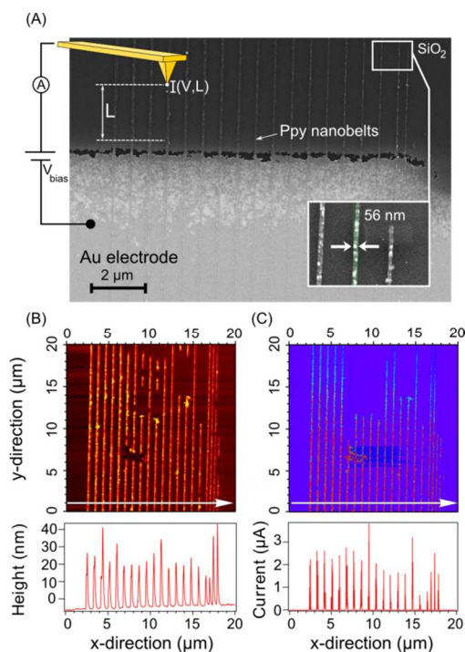
Fig. 1 Schematic setup of the electrical circuit used in the experiments. (A) SEM image of polymer nanobelts (vertical line structure) written on an insulating substrate of SiO 2 and electrically connected to a gold electrode (bottom, bright part). The white box displays the position of the enlarged section of the polymer belts which are used to determine the width of the belts. The schematic
