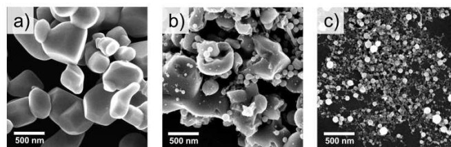
Fig. 2 SEM images of a) the source titania powder b) laser ablated material from titania powder and c) laser ablated material from solid titanium target.
