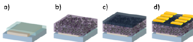
Fig. 3 Built-up of inverted solar cells: a) glass substrate with FTO top layer partially etched away and added compact titania blocking layer; b) adding the active layer consisting of laser ablated titania and P3P6T; c) adding an electron blocking layer; d) evaporation of gold contacts.
