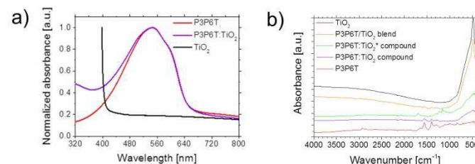
Fig. 5 a) Absorption spectra normalized to maximum absorbance of laser ablated TiO 2 (black curve), pure P3P6T (red curve), and the P3P6T:TiO 2 compound (purple curve). b) Infrared spectra of P3P6T and laser ablated TiO 2 . The red curve represents pure P3P6T and the black one pure TiO 2 by laser ablation from titania powder. A blend of TiO 2 laser-ablated from suspension and P3P6T powder (orange), and the corresponding compound of P3P6T:TiO 2 (purple) are shown. Additionally the compound with TiO 2 ablated from a titanium target, denoted P3P6T:TiO 2 * (green) is shown. Data are shifted along the y-axis for clarity.
