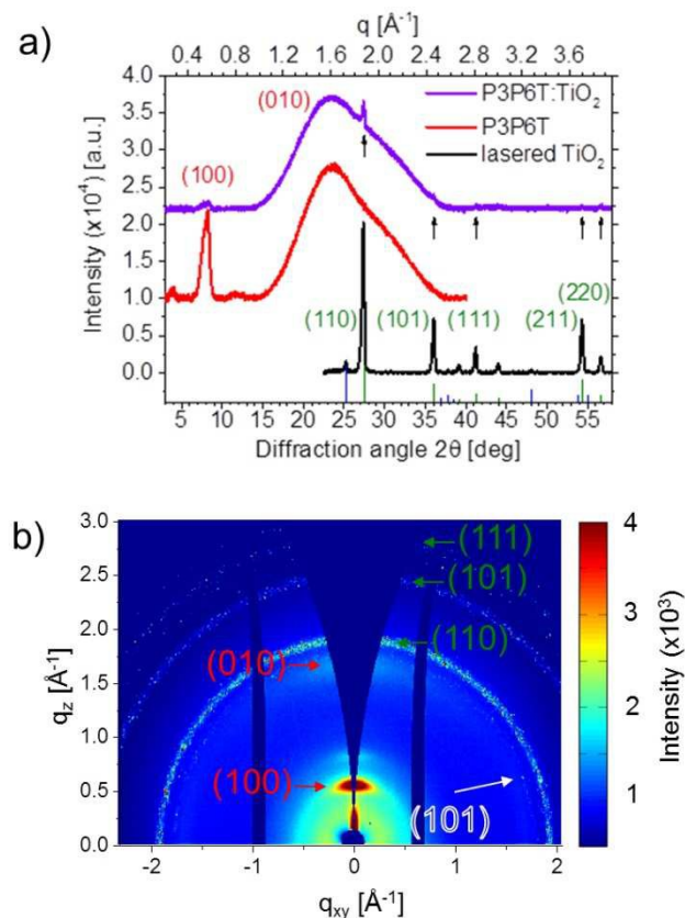
Fig. 4 a) XRD pattern of laser ablated TiO 2 (black curve), P3P6T (red curve) and the P3P6T:TiO 2 compound (purple curve). Theoretical positions of TiO 2 in anatase and rutile phases are plotted in green and blue, respectively. The main rutile peaks, which are observed in the P3P6T:TiO 2 blend are denoted by black arrows. The data are shifted along the y-axis for clarity. b) Two-dimensional GIWAXS pattern of a film of P3P6T:TiO 2 compound. The crystal planes for the polymer are denoted in red letters, whereas the attribution of the observed crystalline phases of TiO 2 is noted by green and white letters for anatase and rutile phase, respectively.
