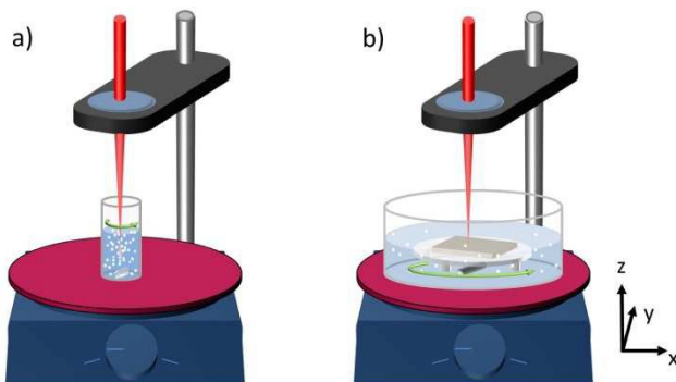
Fig. 1 Basic set-up of laser ablation process for a) aqueous titania powder suspension and b) solid titanium target in water.
