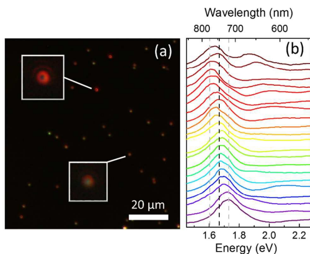
Figure 1. (a) A darkfield microscopy image of gold nanoparticles on a gold film. The insets show a magnified view of two representative particles. (b) Peak-normalized single particle scattering spectra from randomly selected gold nanoparticles.
