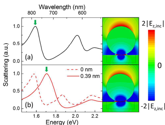
Figure 4. Normalized scattering spectra of a gold nanoparticle (a) on a 4-MBT coated flat gold film and (b) on a corrugated gold surface with d = 0 (dashed line) and d = 0.39 nm (solid line). The field-plots show two-dimensional electric field distributions at the main resonance peak of the spectra as indicated by the green arrows.
