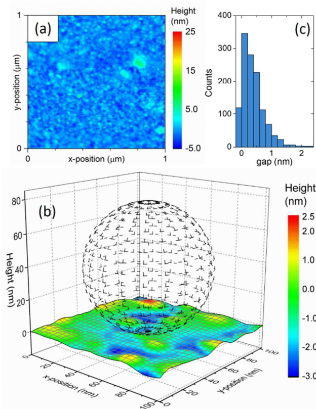
Figure 2. (a) AFM image of a gold film thermally evaporated on glass. (b) Example surface geometry near a liquid-deposited gold nanoparticle deposited on top of the surface shown in (a). (c) Normalized gap size histogram from over 1,200 possible particle locations.
