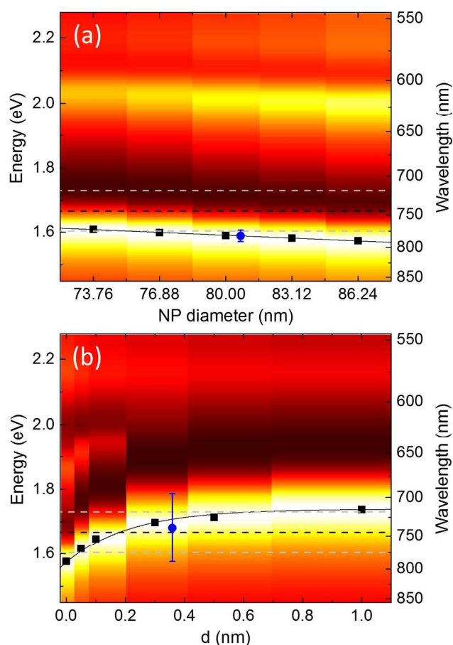
Figure 5. (a) Contour graph of the scattering spectra of gold nanoparticles with different sizes on a flat gold film. (b) Contour graph of the scattering spectra of an 80 nm diameter gold nanoparticle on a rough surface as a function of air gap size d . The black dashed line represents the average resonance energy from the experiment and the two grey dashed lines span 2\sigma on each side. The black squares mark the main peak positions and the solid lines show empirical fits to the peak position. The blue circles represent experimentally expected spectral positions and variations based on numerical simulations.
