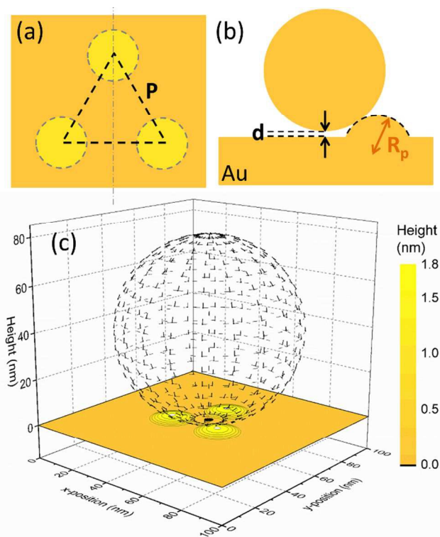
Figure 3. Schematic of a representative simulation geometry and relevant parameters showing (a) a top view without a gold nanoparticle showing three protrusions, (b) a side view along the dashed line in (a) with a deposited gold nanoparticle present, and (c) a perspective view of the final structure.
