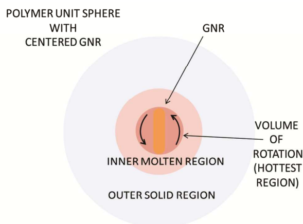
Figure 5. Schematic depiction of the GNR's volume of rotation and the subsequent temperature zones around it based on the polarized perylene spectrum and the inter-particle distances. The volume of rotation registers the hottest temperature as recorded by the rotational spectroscopy, the inner molten region is sampled by the perpendicular perylene emission giving T_{\perp} , and the outer solid region corresponds to the temperature T_{\parallel} , as reported by parallel perylene emission.
