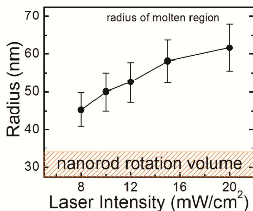
Figure 6. The radius of the inner molten region as a function of the average pulsed laser intensity. The inner molten region is always larger than the sphere corresponding to the length of the GNR (~70 nm), and with increasing photothermal intensity the molten region increases. Although the molten volume grows with increasing intensity, it is still centered on individual GNRs without overlap from adjacent GNRs, thus enabling site-specific processing without influencing the bulk of the sample.
