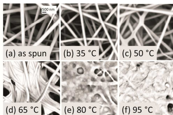
Figure 2. SEM images of PEO nanofibrous composite mats after conventional heating for ten minutes at different temperatures show the clear destruction of the fibrous morphology that occurs under uniform spatial heating, in contrast to the preservation of the nanofiber structure under the heterogeneous temperature distribution created when using photothermal heating. For PEO, T_m = \sim 65 °C.
