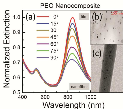
Figure 1. (a) Linearly-polarized extinction spectrum of aligned GNR in PEO nanocomposite. The angle-dependent extinction validates the anisotropic nature of the sample where maximum extinction occurs for parallel polarization and GNR orientation and minimum extinction for the orthogonal configuration. (b) TEM images of aligned GNRs in a PEO film and (c) TEM images of aligned GNRs in PEO nanofibers, both confirming the alignment as depicted in the extinction spectrum. Note: for (c) same scale as (b).
