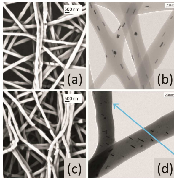
Figure 3. (a) SEM image of randomly oriented PEO nanofibrous mat fabricated by electrospinning. (b) During fiber formation, the gold nanorods align along the fiber axis as revealed by TEM image. (c) After 10 minutes photothermal treatment by the ultrafast laser at an average intensity of 10 mW/cm 2 , the nanofibers retain their fibrous morphology. (d) TEM images reveal photothermal treatment causes localized heating above the melting point of the polymer and the simultaneous application of an external electric field (arrow direction) enables re-orientation of the nanorods without loss of fibrous structure. Under these conditions, from rotational measurements, the average temperature at the nanorod is ~95 °C whereas far from the particle the background temperature is ~32 °C.
