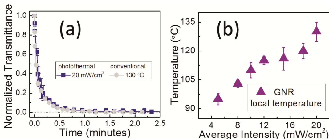
Figure 7. (a) Normalized transmittance through the GNR:PEO nanocomposite sample when photothermally heated with 20 \text{ mW/cm}^2 and conventionally heated at 130 \text{ }^\circ\text{C} . The well-overlapped curves indicate that a good estimate of the steady state temperature of the nanocomposite at the GNRs when irradiated with 20 \text{ mW/cm}^2 is 130 \text{ }^\circ\text{C} . (b) With this approach, estimates of nanocomposite temperatures as determined by comparing rotation rates under pulsed laser intensities. GNR local temperature refers to the average temperature in the volume of rotation of the nanorod.
