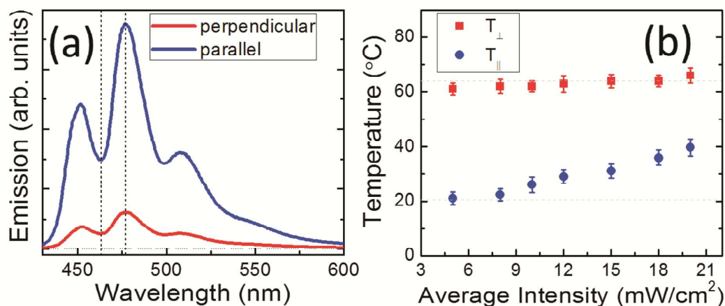
Figure 4. Nanocomposite film samples under ultrafast pulsed excitation. (a) The characteristic perylene spectrum corresponding to parallel (blue) and perpendicular (red) emission detection for a 20mW/cm 2 photothermal excitation of GNRs. The differences in overall amplitude of the spectra depict the difference in populations emitting parallel or perpendicular polarized light. (b) The raw spectrum can be converted to temperature using the calibration system explained in the experimental section, and thus corresponding to different photothermal intensities we obtain two different temperatures, T_{\parallel} and T_{\perp} . The T_{\parallel} ( T_{\perp} ) component reveals the steady-state temperature of the sample far away from (closer to) the GNRs. Dashed horizontal lines indicate room temperature and PEO T_m , respectively.
