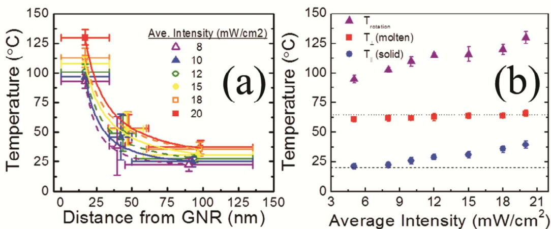
Figure 8. (a) The distribution of temperatures associated with these three spatial regions for varying average intensities of the pulsed irradiation. (b) Summary of the results of the three measurements for temperature in the different spatial regions as the average laser intensity is increased.
