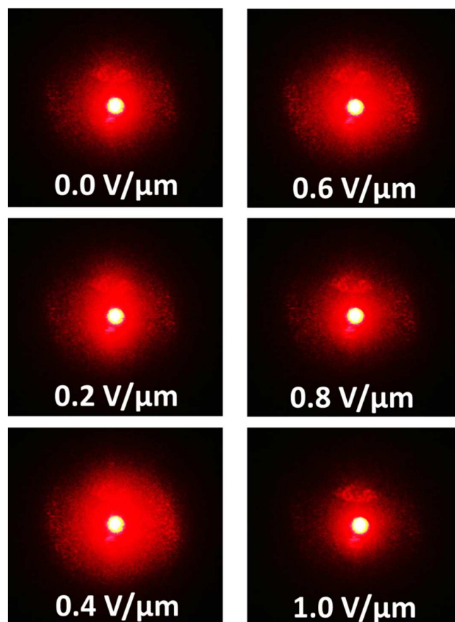
Figure 5: A laser beam passing through the electro-optical device. The voltage applied to the device is increased from 0 to 1 V/μm. The laser beam is most diffused at 0.4 V/μm by the LC molecules.
