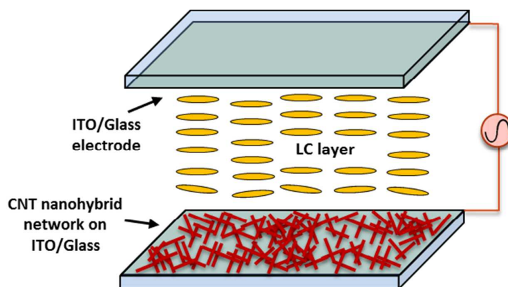
Figure 3: The schematic diagram of the fabricated CNT nanohybrid network and LC based electro-optical device.
