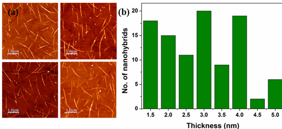
Figure 2: The distribution of nanohybrid thickness in the sample solution used. (a) Represents AFM images of nanohybrids drop cast on Si using a 0.01 \text{ mg ml}^{-1} solution. (b) A histogram representing the nanohybrid count vs. the respective thickness.
