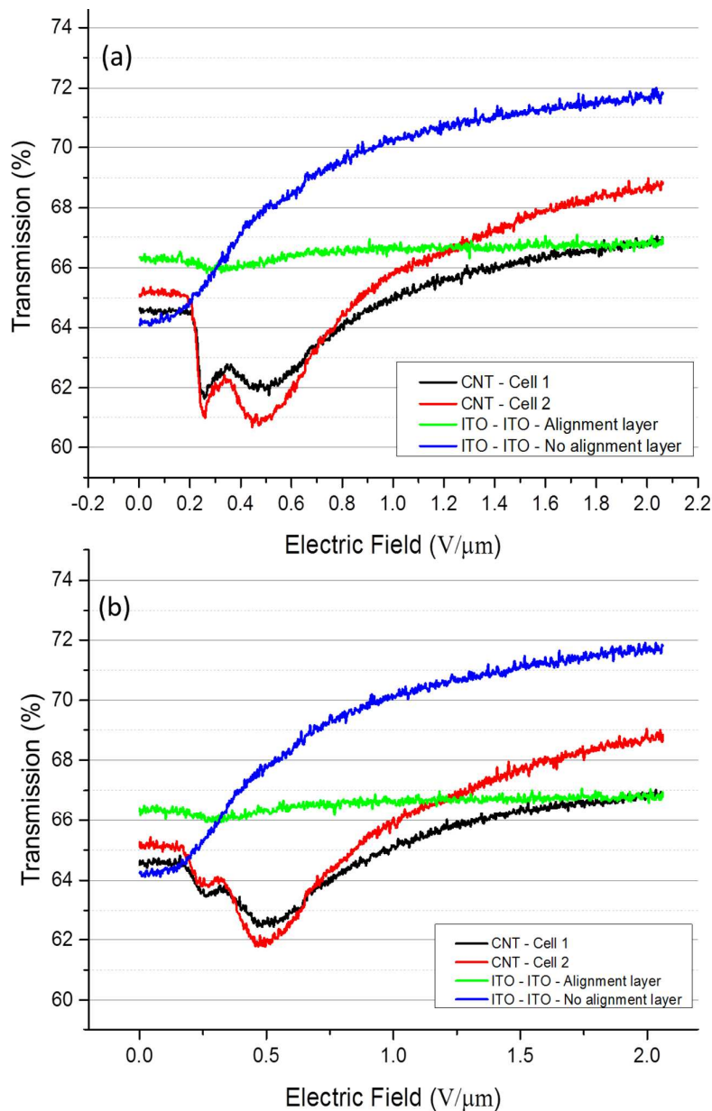
Figure 6: The comparison of cross polarised optical transmission through a ITO-ITO LC cell without alignment layers, ITO-ITO LC cell with alignment layers, nanohybrid network/LC cells with nanohybrid network thickness of 2nm (Cell 1) and 5nm (Cell 2). All cells had 10 μm spacing filled BL006 LC and the applied field frequency was 1 KHz. Field applied in (a) forwards and in the (b) reverse direction.
