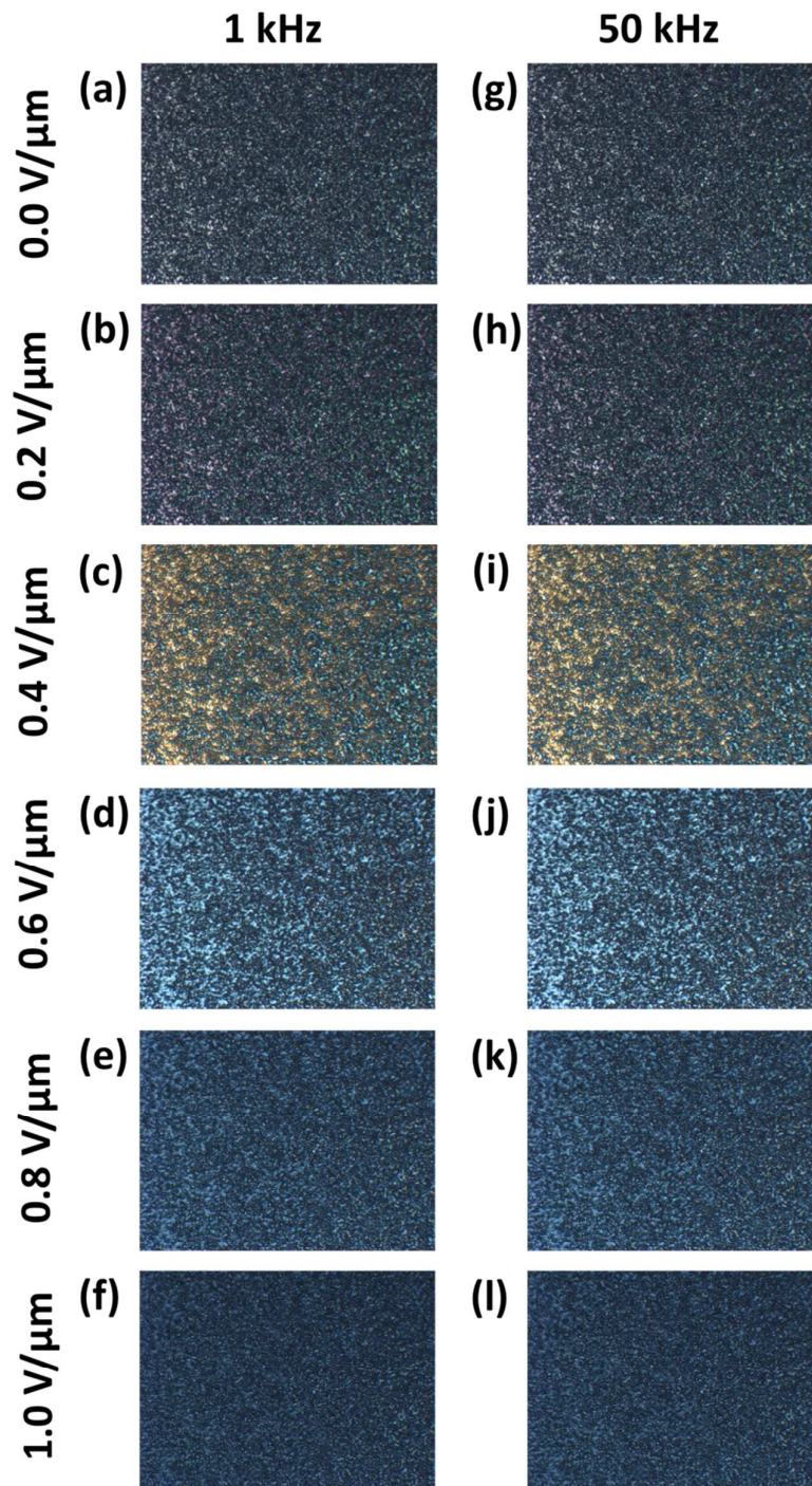
Figure 4: (a-f) Nanohybrids and LC based device viewed under a cross polarised microscope with 1 kHz voltage signal. (g-l) The same measurement repeated at 50 kHz voltage signal. The voltage values are in rms.
