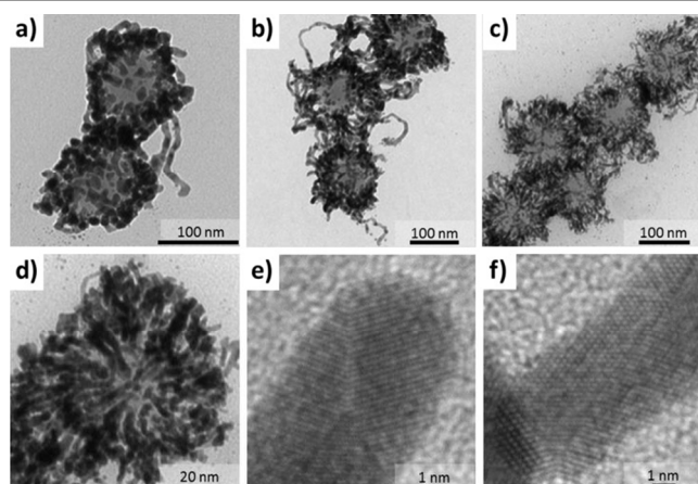
Figure 4. TEM characterization of SGNUs synthesized in flow microreactor system in continuous manner. Residence time in the reactor was 12 min. a–c) Flow rate ratio of \text{NaBH}_4 solution and gold precursor was varied to control the structure: a) 50:50, b) 20:50 and c) 1:50 ( \text{NaBH}_4 :gold precursor solution, \mu\text{L}/\text{min.} ). d) Magnified TEM image of SGNU at 1:50 ratio (see Fig. S7 for images of other conditions). e) High resolution TEM image showing the tip of a polycrystalline gold nanobranches. f) Root of a gold nanobranch on the silica particle surface.
