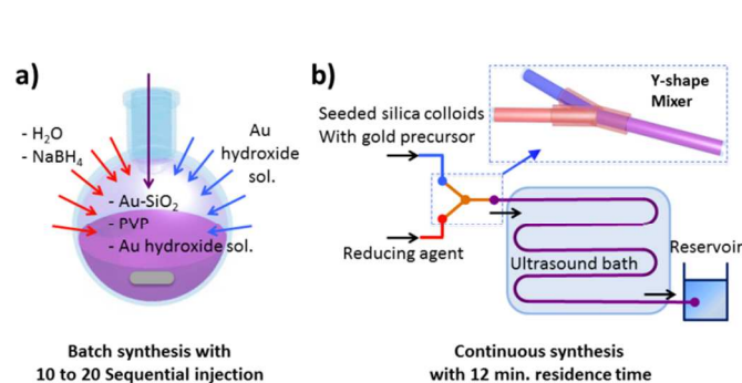
Figure 1. Synthesis procedures to produce SGNU nanoparticles. a) Batch production with sequential addition of reagents. Gold hydroxide solution and \text{NaBH}_4 solutions were added under a 2 minutes frequency. b) Microfluidic approach injecting the reagents in continuous mode. The residence time was kept constant at 12 minutes.
