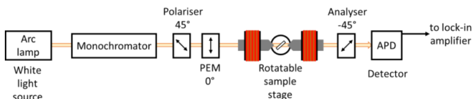
Figure 3) Schematic of experimental setup for ellipsometric measurements with a magnetic field
