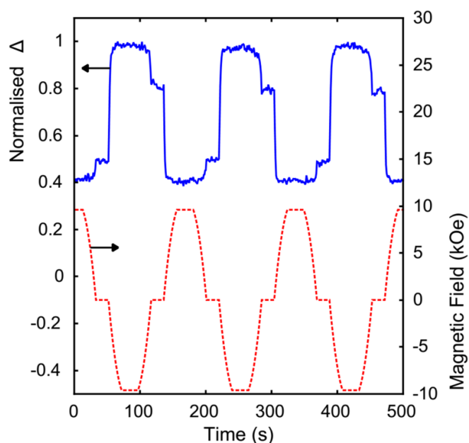
Figure 5) Normalised \Delta at 540 nm wavelength and 15 degrees AOI against time varying magnetic field.
