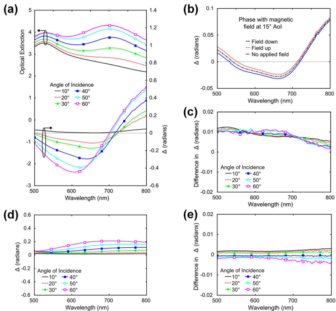
Figure 4 a) Optical extinction spectra and \Delta at varying AOI of Au Core – Co Shell sample with no field applied. b) Measurements of \Delta across the wavelength range, showing the difference for oppositely oriented magnetic fields and the two resonance conditions present at 15 degrees AOI. c) Difference in measured value of \Delta when the direction of magnetic field is reversed for Au Core – Co Shell sample. d) & e) \Delta with no field applied, and the difference in \Delta for opposite fields at varying AOI's for hollow cobalt nanotubes.
