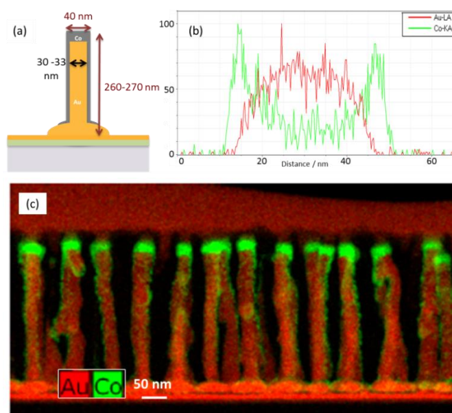
Figure 1 a) Core-Shell nanowire schematic b) EDX line scan profile across one wire c) STEM cross-section
