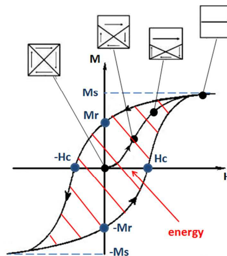
Fig. 1 Hysteresis loop of a ferromagnet (squares show domain wall displacement with increasing field strength). The area of the hysteresis loop represents the energy dissipated during a magnetisation cycle.
