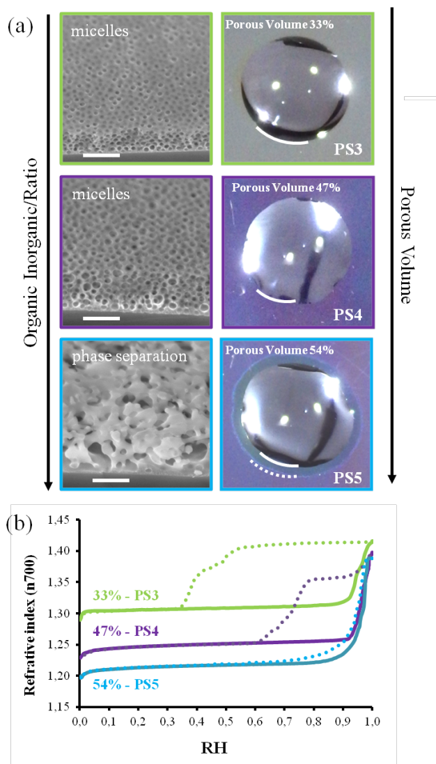
Figure 3. a) SEM images (scale bar 300 nm) and corresponding images of a water drop deposited onto the surface of PS3, PS4 and PS5 films. Only sample PS5, which has a higher porosity vol%, shows a capillary ring. b) EEP adsorption/desorption isotherms (film refractive index at wavelength 700nm versus relative humidity) of PS3, PS4 and PS5 samples.
