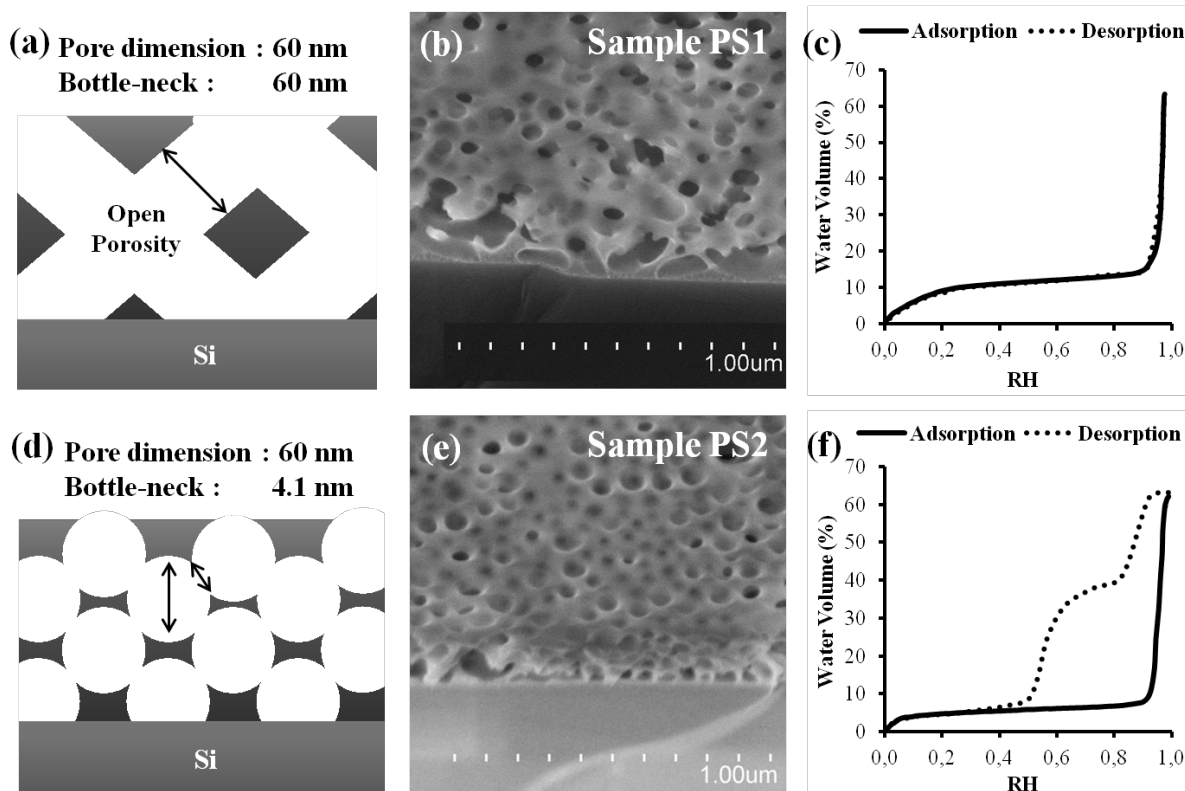
Figure 1. (a), (d) Simplified schemes (b), (e) SEM images (c), (f) EEP adsorption/desorption isotherms (water volume versus relative humidity) of the PS1 and PS2 samples respectively. The lack of hysteresis in (c) suggests an internal structure of the thin film with large bottlenecks.
