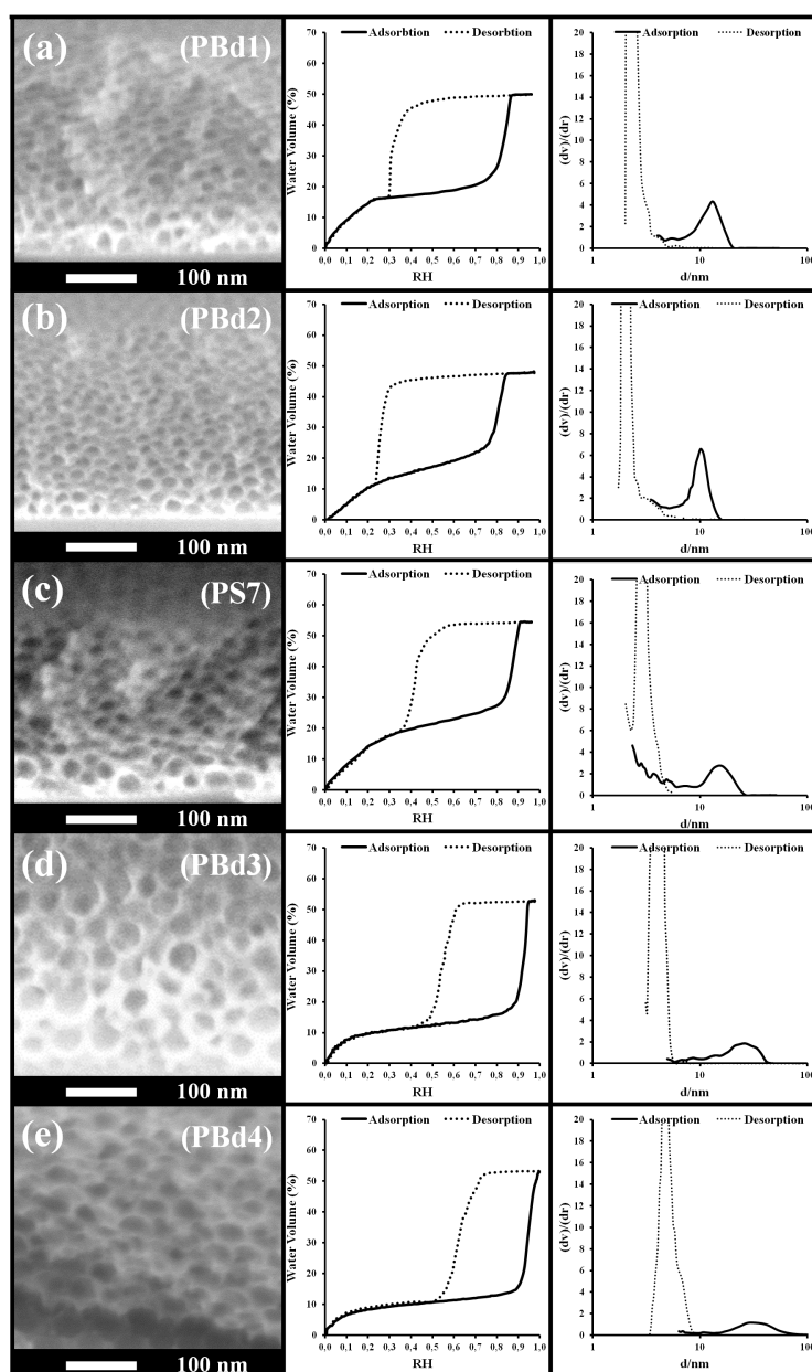
Figure 7. left) SEM images, center) EEP adsorption/desorption isotherms (water volume versus relative humidity) and right) pore size distribution of the PBd1, PBd2, PS7, PBd3 and PBd4 samples of the intermediate section of Table 2. The samples are reported in decreasing order of the water filling speed.
