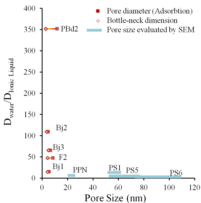
Figure 10. D_{\text{water}}/D_{\text{IL}} values for samples reported in Table 2. The same code of Figure 9 has been used to express the pore and constriction sizes.
