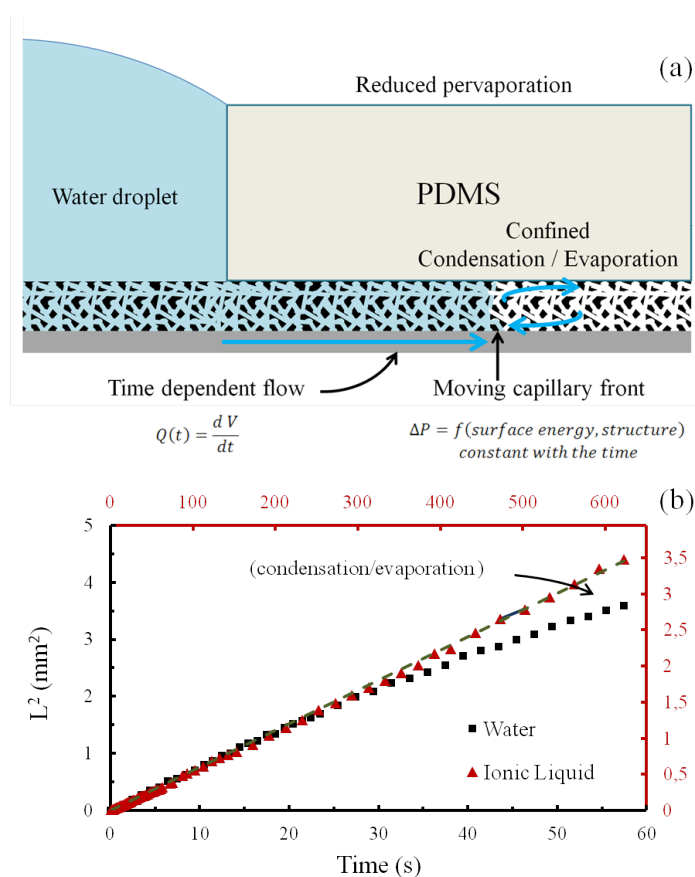
Figure 4. a) Scheme of the phenomena taking place when a water drop stands at the edge of PDMS top cover (stamp) on a thin film that allows wicking. b) Graphic displaying the diffusion limited capillary filling of the PS1 porous film with water and with (1-Ethyl-3-methylimidazolium dicyanamide) ionic liquid, in the configuration illustrated in a). Black (points and axes) corresponds to water, while red (points and axes) correspond to the ionic liquid. The initial position of the fluid corresponds to the edge of the PDMS stamp. Dots are experimental points and plain lines are linear fits of the first 20 points of both curves.
