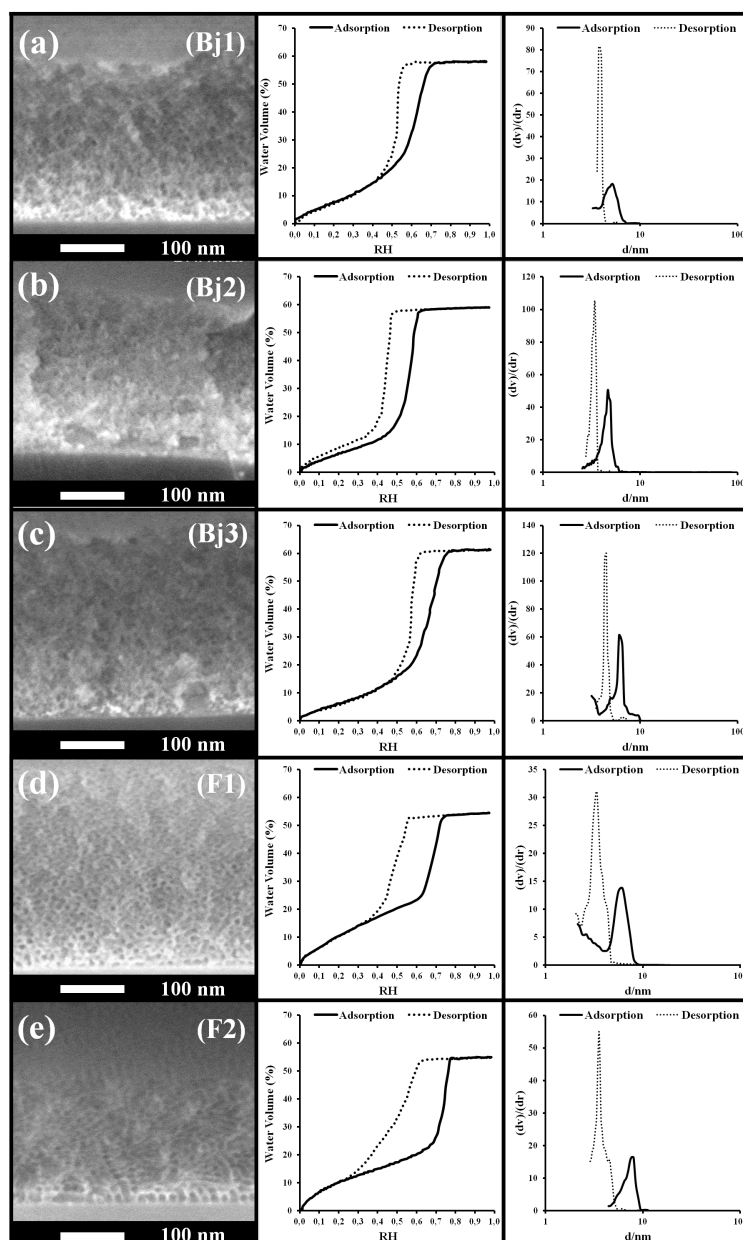
Figure 6. left) SEM images, center) EEP adsorption/desorption isotherms (water volume versus relative humidity) and right) pore size distribution of the Bj1, Bj2, Bj3, F1 and F2 samples of the intermediate section of Table 2. The samples are reported in decreasing order of the water filling speed.
