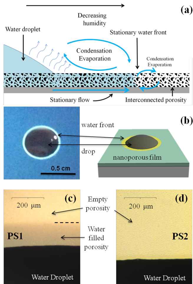
Figure 2. a) Scheme of the phenomena taking place when a water drop stands free on a thin film that allows wicking; b) picture and corresponding scheme representing a sessile water drop deposited onto the surface of PS1 and surrounded by its capillary ring. c) and d) zoomed optical images of the triple line showing the presence of the capillary ring in PS1 and no capillary ring in PS2.
