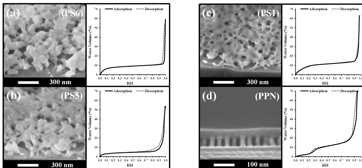
Figure 5. SEM images and corresponding EEP adsorption/desorption isotherms (water volume versus relative humidity) of the PS5, PS6, PS1 and PPN samples (top section of Table 2).
