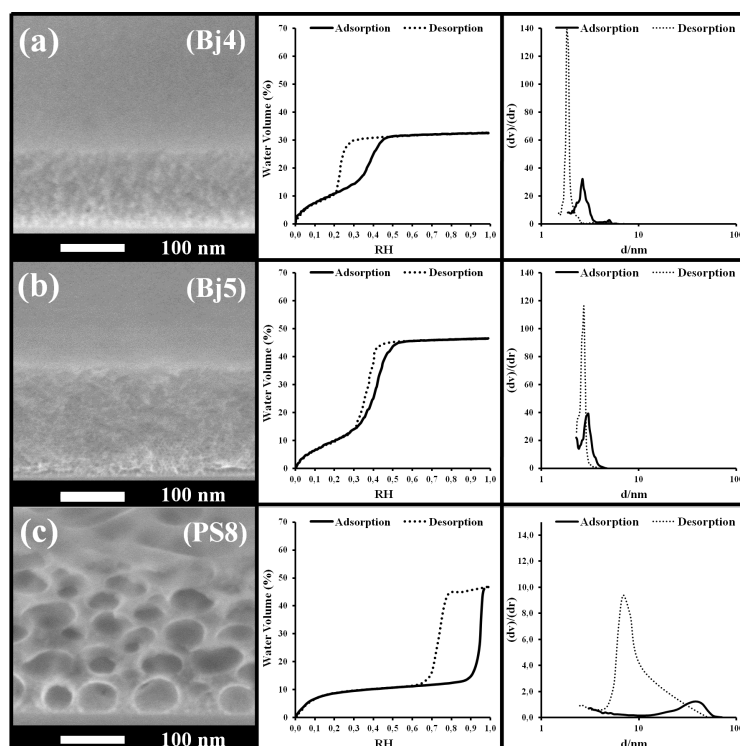
Figure 8. left) SEM images, center) EEP adsorption/desorption isotherms (water volume versus relative humidity) and right) pore size distribution of the B j 4, B j 5, PS8 samples of the third section of Table 2.
