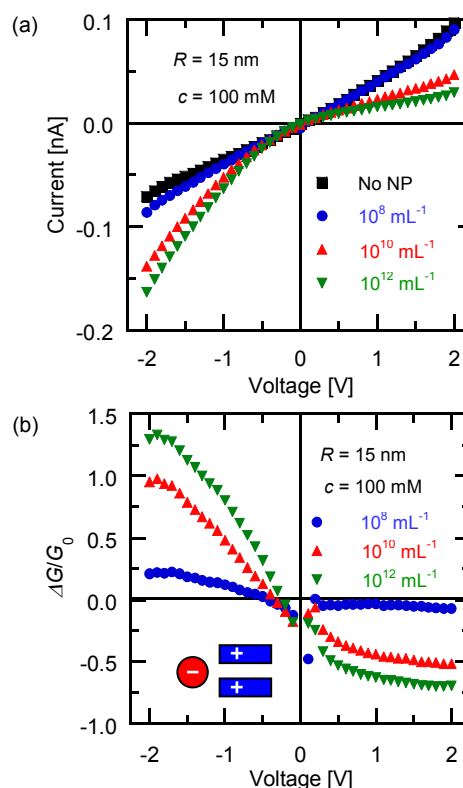
Fig. 5 I-V curves for the negative particle and the positive pore parametrically in the NP concentration (a). The relative change in the conductance, \Delta G/G_0 , is obtained from the I-V curves of Fig. 5(a). The inset shows the experimental conditions and the relative sizes of the pore and particle.
