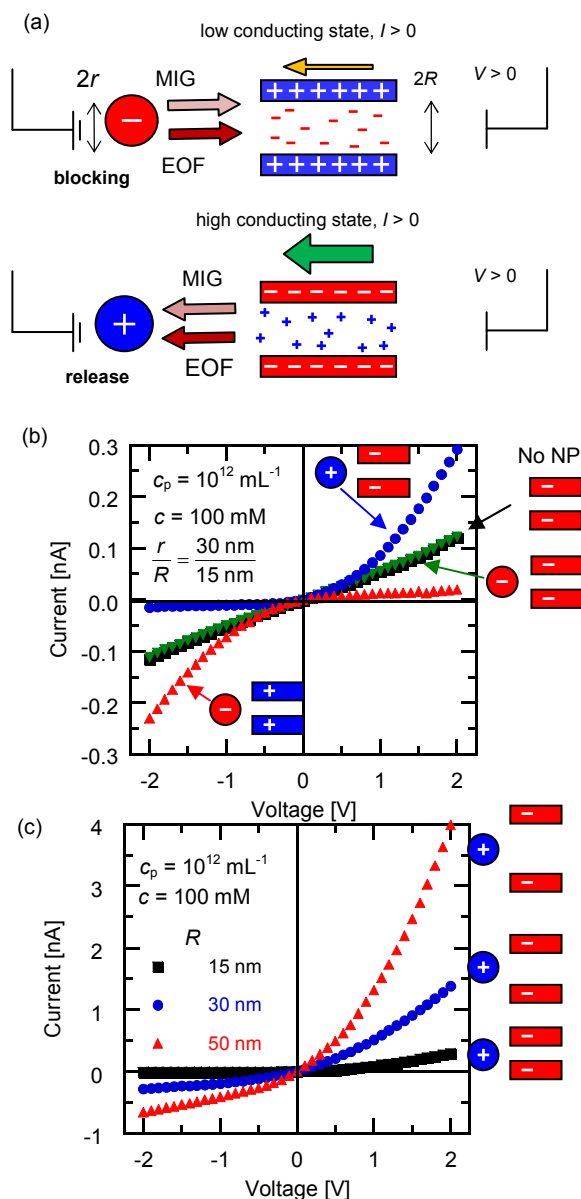
Fig. 2 The charged NP and the nanopore with the mobile charges compensating for the opposite charges fixed to the pore walls (a). We consider three experimental cases ( r > R , r \approx R , and r < R ) although only the case r \approx R is shown in the figure for simplicity. The radii combinations r = 30 \text{ nm} > R = 15 \text{ nm} and r \approx R = 30 \text{ nm} allow significant pore blocking while the case r < R = 50 \text{ nm} permits particle translocation. The current I > 0 and its relative value (arrow) are shown for voltage V > 0 (the ground electrode is placed on the left side of the pore). Electro-osmotic (EOF) and migration (MIG) flows at the pore entrance are drawn out of the pore for the sake of clarity and should be reversed for V < 0 . I - V curves for the negative (PS-COO - ) and positive (PS-NH 3 + ) NPs and the oppositely charged pores. The curves for the negatively charged pore in absence of NPs and in presence of negatively charged NPs are also included (b). I - V curves for the positive NP and the oppositely charged pore parametrically in the pore radii R (c). The insets show the experimental conditions.
