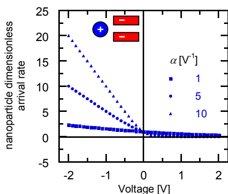
Fig. 3 NP arrival rate scaled to the purely diffusional rate, \dot{N}_p/\dot{N}_0 , as a function of V . The different values of \alpha are dictated by the relative signs and magnitudes of the migration and electro-osmotic terms in Eq. (1). Note the inverse correspondence between the positive NP arrival to (and blocking of) the pore mouth in this figure and the low ionic current I in Fig. 2(b) for V < 0 .
