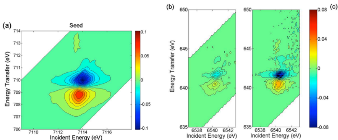
Figure 3. (a) RIXS-MCD spectrum measured at room temperature at the Fe K pre-edge for the seed. RIXS-MCD spectra measured at room temperature at the Mn K pre-edge for (b) CS particles and (c) \text{Mn}_{0.5}\text{Zn}_{0.5}\text{Fe}_2\text{O}_4 particles.
