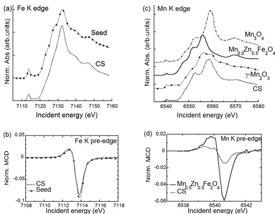
Figure 2. (a) HERFD-XAS spectra measured at the Fe K -edge using the maxima of K\alpha_1 emission lines for the CS nanoparticles (dashed line) and the seeds (dashed line with triangles- Note that symbols are plotted every twenty experimental points). (b) K\alpha_1 -detected HERFD-XMCD spectra measured at the Fe K edge for the CS particles and the seeds. The spectra are normalized to the HERFD-XAS pre-edge maximum. (c) HERFD-XAS spectra
