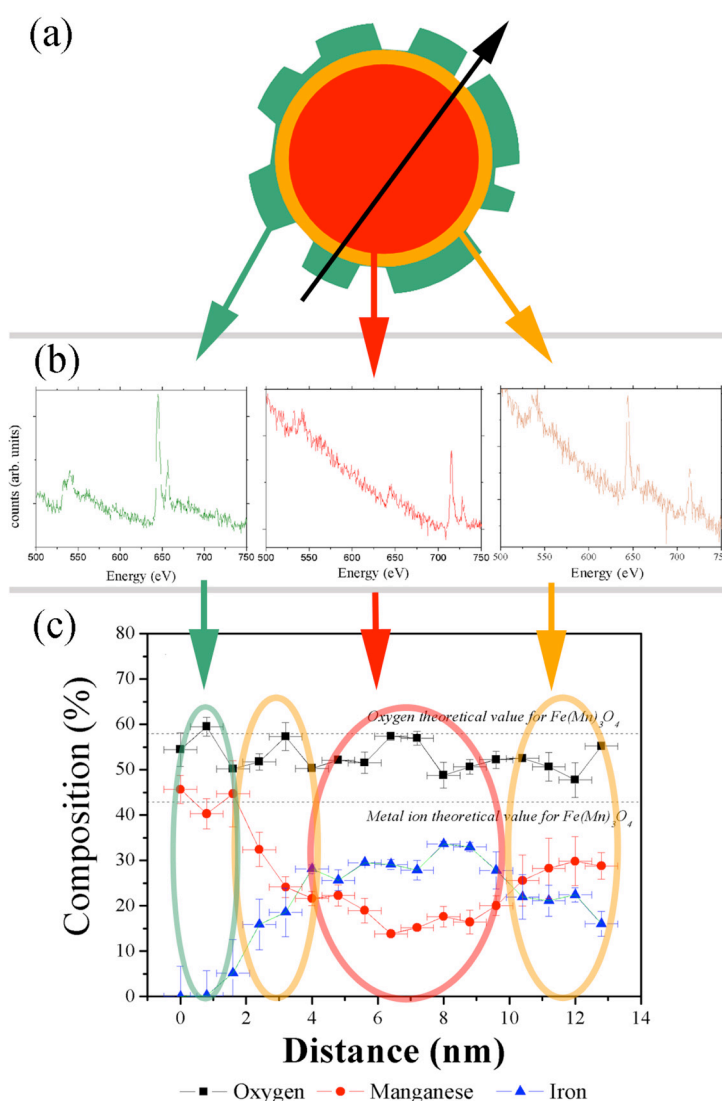
Figure 1. (a) Schematic representation of the irregular shape of a CS nanoparticle (the arrow indicates the direction of the EELS measurements); (b) EELS spectra at three different positions of the particle: core, inner and outer shells; (c) elemental quantification along the particle diameter: Fe (triangles), Mn (circles) and O (squares).
