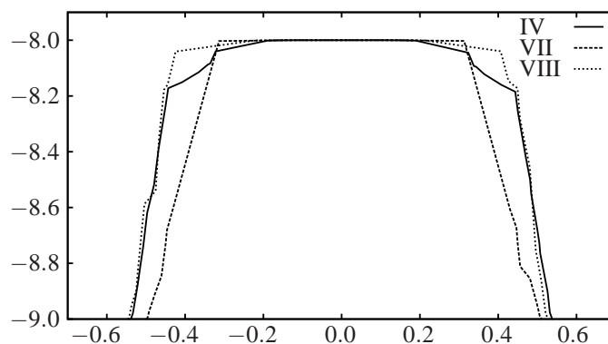
Fig. 5 The variation of energy along the integrated path length for the paths including transition states IV, VII and VIII in the six-particle cluster.
