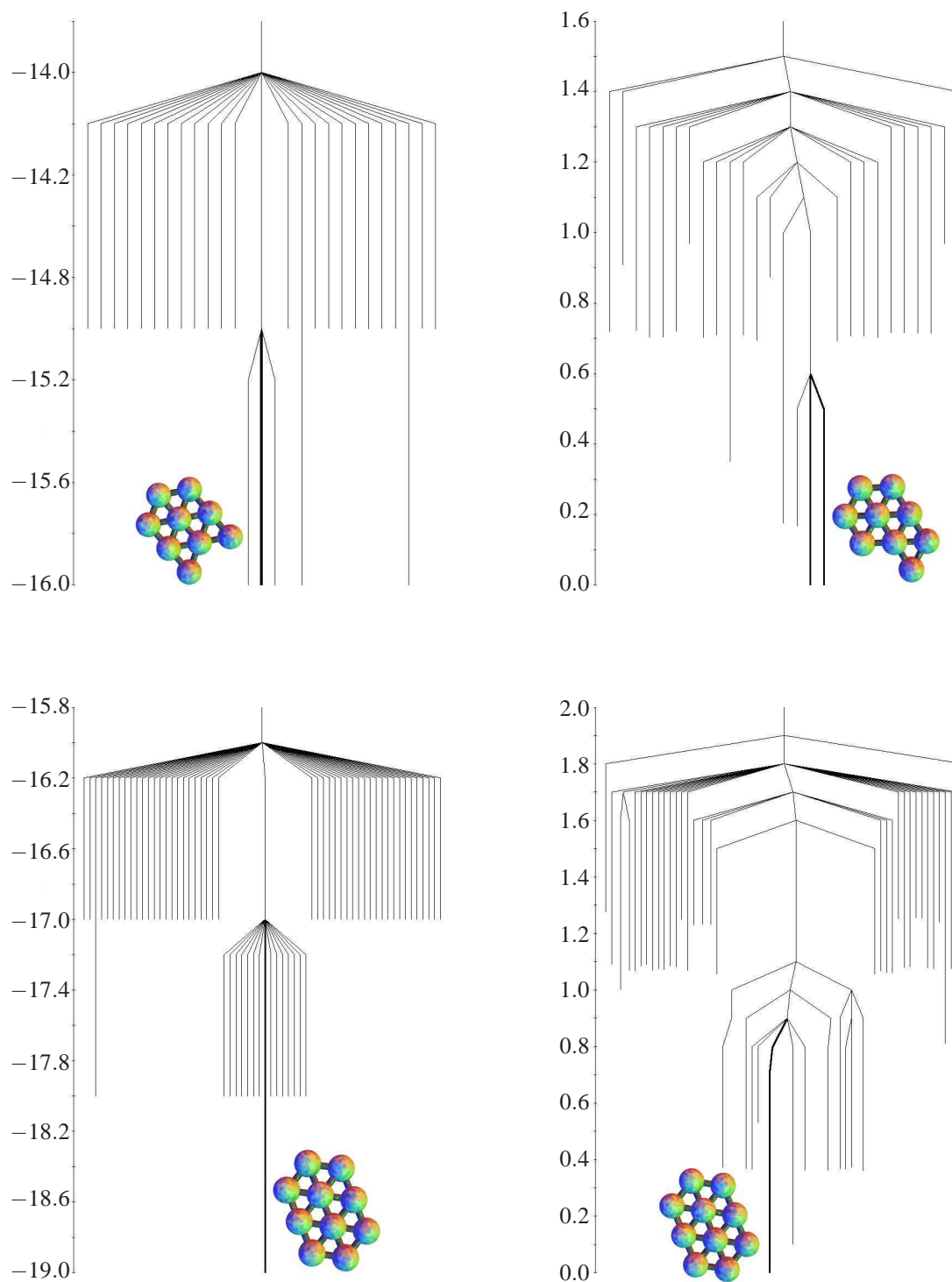
Fig. 8 The potential energy (left) and free energy (right) disconnection graphs for the nine-particle (top) and ten-particle (bottom) clusters. The branch corresponding to the global minimum is highlighted in bold along with the structure.
