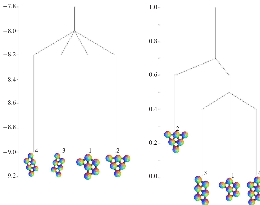
Fig. 6 Potential energy (left) and free energy (right) disconnectivity graphs ( k_B T / \varepsilon = 0.25 ) for the six-particle cluster.
