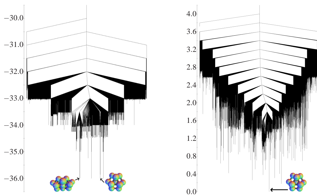
Fig. 10 Potential energy (left) and free energy ( k_B T / \epsilon = 0.25 ) (right) disconnectivity graphs for the 13-particle three-dimensional cluster. On the potential energy graph, the global minimum D_{3h} structure and the quasi-degenerate C_{2v} are shown. On the free energy graph, the global minimum D_{3h} structure is shown.
