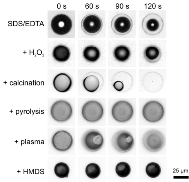
Figure 2 Wetting behavior of S. turris valves as a function of time. First row: SDS/EDTA-treated valve slowly filling up with water (note: the air bubble inside the cell wall appears dark in the images, the white spot in the center of the cell wall is an artifact). Second row: The H 2 O 2 -treated sample shows a similar behaviour. The air bubble is stable for about 1 minute. Third row: Calcination leads to an immediate collapse of the air bubble. Fourth row: The pyrolyzed valve shows the best results, the air bubble stays intact for at least 2 minutes. Fifth row: After additional air plasma cleaning (2 min), the air bubble collapses already after 1 minute. Sixth row: As hydrophilised reference sample, biosilica was treated with hexamethyldisilazane (HMDS). The air bubble remained then intact for at least 5 minutes.
