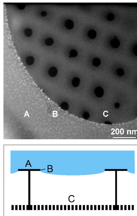
Figure 6 High resolution He-ion microscopic image (top) of pyrolyzed biosilica with regioselectively assembled Au-NPs (layer-by-layer method). Corresponding wetting scheme (bottom): wetted outer surface (A), the three phase contact line (B) and cribrum (C).
