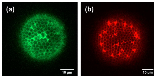
Figure 3 Comparison of CLSM images of CdTe NPs regioselectively attached to a diatom valve using covalent coupling (a) and the layer-by-layer approach (b). Note that the color encoding can be chosen arbitrarily. Green symbolizes covalent coupling, red the layer-by-layer approach. Note that the tubular extensions (cf. Figure 1(a)) are visible as strongly fluorescent spots especially in (b).
