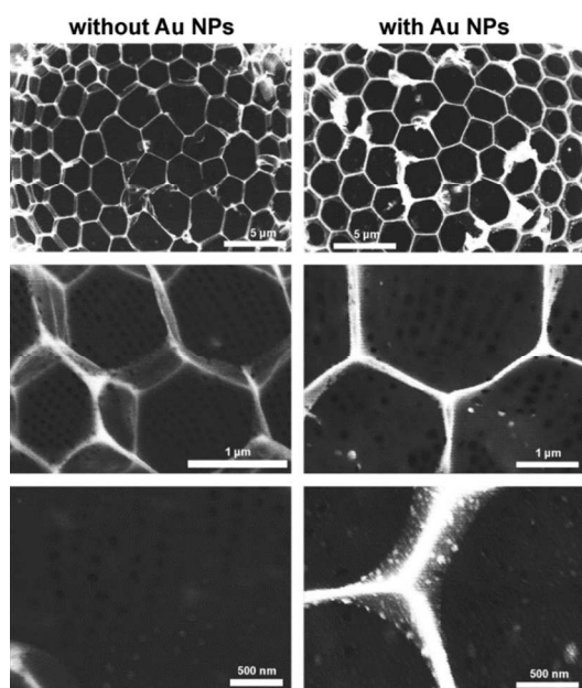
Figure 5 Backscatter electron microscopic images of pyrolyzed biosilica without (left) and with (right) regioselectively assembled Au-NPs (layer-by-layer method). The images were measured under identical conditions. Note the tendency of noble metal nanoparticles to aggregate.
