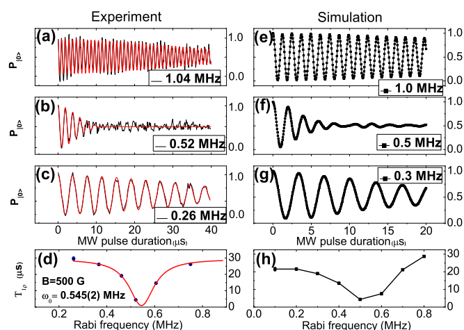
Fig. 2 (Colour online) Hartman-Hahn resonance between electron spin and nearby ^{13}\text{C} nuclear spins. (a-c) Rabi oscillation of centre electron spin driven by different MW power under B=500 Gauss. (d) Dependence of the envelope decay time ( T_{1\rho} time) on the Rabi frequency. A dramatic decay was observed at the Hartman Hahn condition ( \Omega_R = \gamma_c B = 545 kHz), which indicates that the spin polarization transfer channel was built under such condition. (e-h) Numerical simulation results of a-d.
