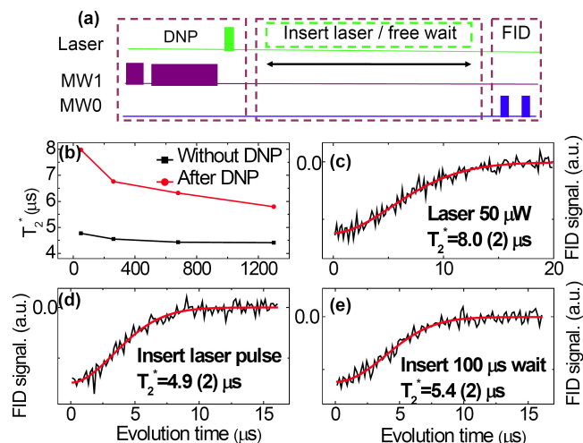
Fig. 4 (Colour online) Influence of laser pulse. (a) Pulse sequence used to investigate laser depolarizing effect. (b) Laser power Dependence. The red (black) scatters are the measured T_2^* times after (without) DNP pumping process under 4 different laser power. Lower laser power gives stronger enhancement of centre spin coherence time. (c) The FID result with DNP pumping at the optimized laser power ( 50\ \mu\text{W} ). The T_2^* time of electron spin is \sim 2 times longer than the case without DNP pumping. (d) FID after adding depolarizing laser pulse. The insertion of laser pulses will depolarize the bath spin polarization built by DNP process, resulting in a dephasing time close to the case without DNP. (e) FID after adding free waiting segment. The extra waiting time decreases the effective number of DNP cycles, so an in-between dephasing time is observed.
