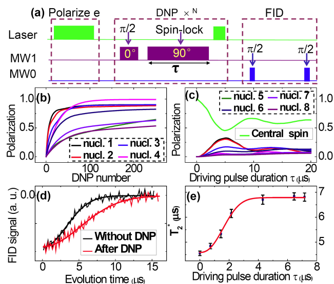
Fig. 3 (Colour online) Polarization transfer process and enhancement of centre spin coherence ( T_2^* ) time. (a) The pulse sequence used to generate (the DNP sequence) and to examine (the FID sequence) nuclear spin bath polarization. (b-c) Numerical simulations of the polarization transfer process. For 8 random located ^{13}\text{C} nuclear spins around an NV centre, the dependence of spin polarization on (b) DNP number and (c) spin-lock driving duration are monitored. (d) Experimental measured FID signals without (black line) and after (red line) DNP, the prolongation of the dephasing time (from 4.6 μs to 7.4 μs) indicates that the bath spin is polarized during the DNP process. (e) Dependence of the T_2^* time on the DNP pumping duration, with N=10 . The magnetic field is 660 Gauss for these measurements.
