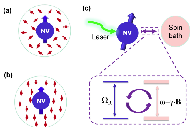
Fig. 1 (Colour online) General Schematic. (a) Spin bath in thermal equilibrium, red arrows represent 13 C nuclear spins around centre electron spins. The thermal fluctuations of the unpolarized spin bath usually causes fast decoherence of the centre spin. (b) After DNP, the 13 C nuclear spins close to the NV centre are polarized, and centre spin coherence can be well protected by the polarized bath. (c) Polarization transformation around an NV centre in diamond. Inset, the Hartman-Hahn condition (see equation 2).
