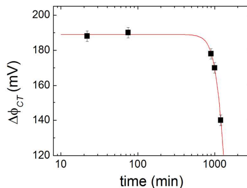
Fig. 6 Work function difference between trans and cis SAMs on Au as measured by macroscopic KP.
