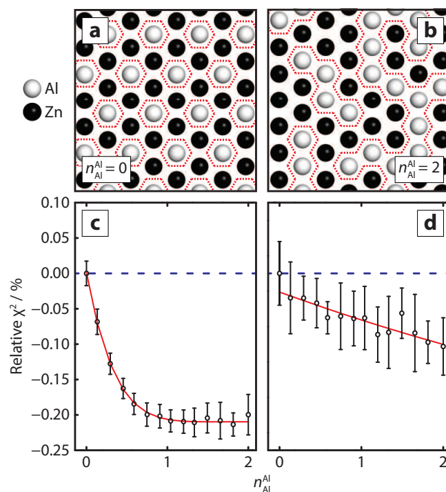
Fig. 4 Cross-sections of ordered (a) and disordered (b) cation arrangements. Oxygen and hydrogen atoms are omitted for clarity. The dotted red lines in a and b indicate Al/Zn boundaries. \chi^2 values, expressed as the percentage difference from the first data point (blue dotted line), are shown for the F(Q) (c) and D(r) (d) data. The error bars represent the corrected sample standard deviations, each derived from six RMC refinements. The red lines show error-weighted three-parameter polynomial fits of the form \chi_{\text{rel}}^2 = \chi_0^2 + \alpha(n_{\text{Al}}^{\text{Al}} - n_0)^6 , chosen to capture the particular nonlinearity of the dependency observed in (c).
