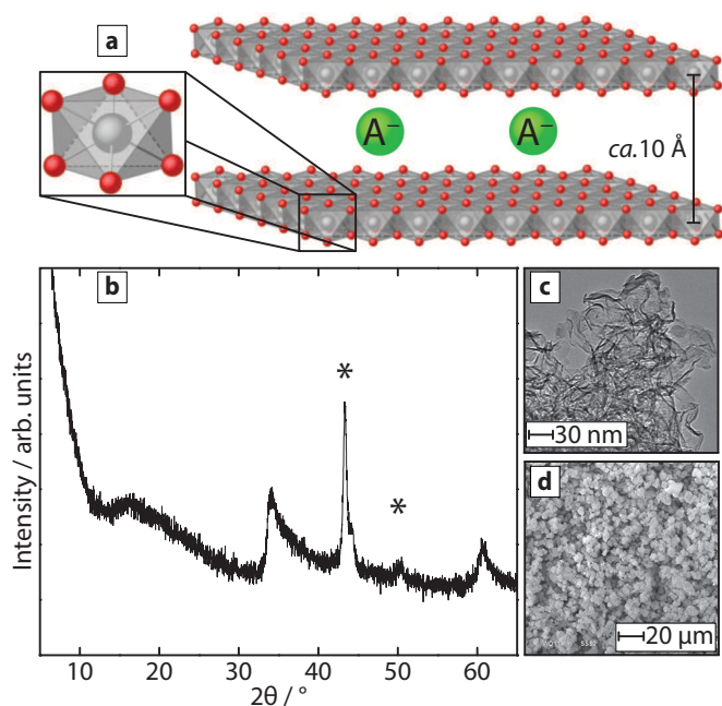
Fig. 1 (a) schematic of a typical crystalline LDH structure; edge-linked metal octahedra form sheets, spaced by interlayer anions ( A^- ; here, predominantly borate). (b) PXRD pattern of the AMOST-prepared Zn_2Al -borate LDH. In the crystalline parent compound, (00l) peaks are evident in PXRD patterns typically between ca. 10–25°. Asterisks denote scattering from the sample container. TEM and SEM images of the sample are shown in c and d. Panels b, c and d are adapted from Ref 11.
