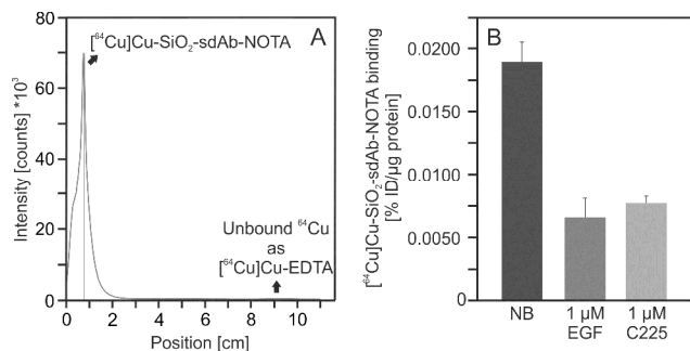
Figure 7 Radiolabelling and cellular binding of SiO 2 -sdAb-NOTA. After modification with 1,4,7-triazacyclononane-triacetic acid (NOTA), sdAb-functionalised silica nanoparticles were labelled with 64 Cu until a radiochemical purity of >98 % was obtained as analysed by radio-TLC (A). A 1 μM excess of human epidermal growth factor (EGF) or of the EGFR-inhibitory antibody Cetuximab (C225), respectively, blocks binding of radiolabelled sdAb-functionalised silica nanoparticles to EGFR-presenting FaDu cells. Binding data are expressed as % of injected dose per μg protein (% ID/μg protein). Each point represents the mean ± SD of three samples.
