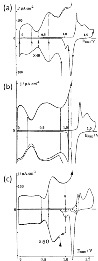
Figure 2: Cyclic voltammograms recorded for high index planes of gold single crystals in perchloric acid (a) (311), (b) (310) and (c) (554). Adapted from figures 4, 9 and 11 ref 54 with permission of Elsevier.
