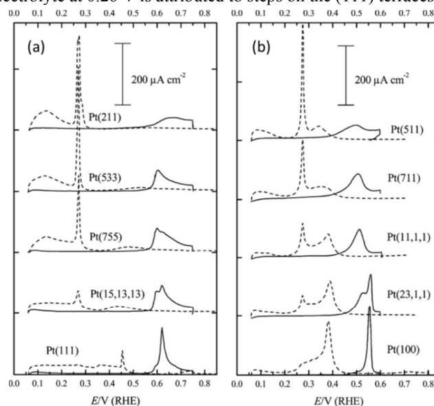
Figure 3: Voltammetric profiles of Pt single crystal electrodes with irreversible adsorbed (a) bismuth and (b) germanium recorded in 0.5 M \text{H}_2\text{SO}_4 . Adapted from Figures 1 and 3 in ref 58 with permission of the Royal Society of Chemistry.
