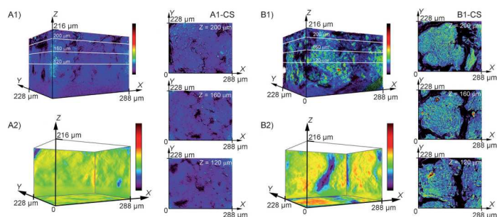
Figure 9: The distribution of Pt catalysts in the cathode catalyst layers of A) fresh and B) degraded MEA as observed by 3D-laminography–XANES. The change in colour intensity reflects the quantity of Pt. Cross sectional images of the MEA are also shown in the X–Y plane. A2) and B2) are 2D projections of the summation of the change of intensity onto the X–Y, Y–Z, and Z–X planes of (A1) and (B1). Reprinted from ref 109 with permission of Wiley.
