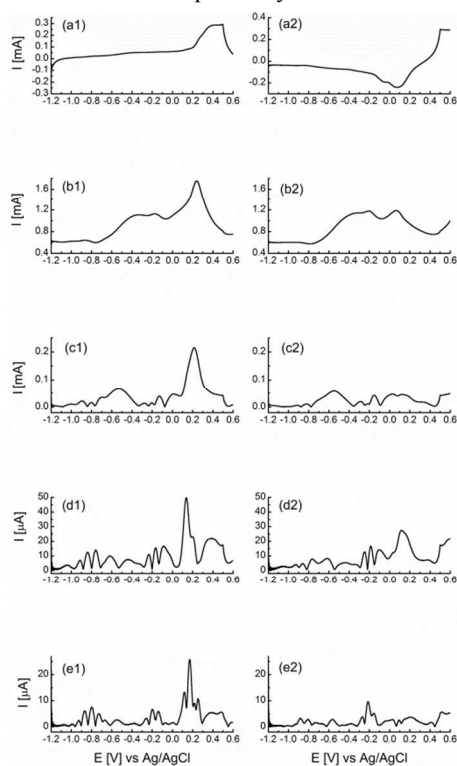
Figure 6: Large amplitude Fourier transformed ac voltammograms recorded at an electrodeposited porous Au surface in 1 M NaOH showing the fundamental to fifth ac harmonic responses. The voltammograms have been split into the forward (a1-e1) and reverse (a2-e2) sweeps for clarity. Reprinted from ref 77 with permission of the Royal Society of Chemistry.
