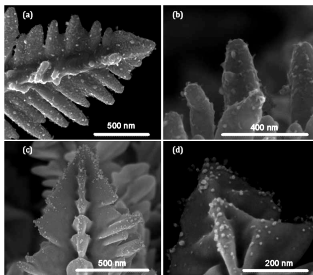
Figure 8: SEM images of electrodeposited porous Au decorated with (a, b) Ag and (c, d) Pd via a spontaneous electroless deposition approach. Adapted from figure 11 in ref 77 with permission of the Royal Society of Chemistry.
