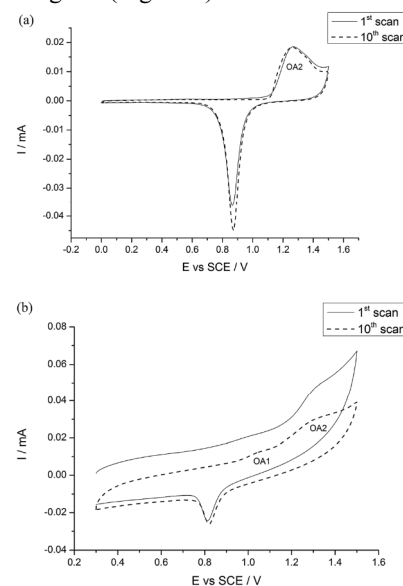
Figure 5: Cyclic voltammograms recorded in 0.5 M H 2 SO 4 at (a) macro Au electrode and (b) Au nanoparticles demonstrating the prominence and stability of the OA1 peak at the Au nanoparticles. Reprinted from ref 80 with permission of the Royal Society of Chemistry.
