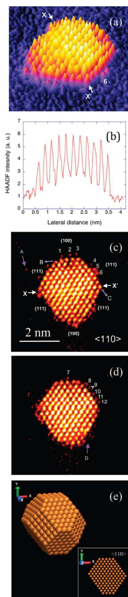
Figure 12: (a) 3D intensity plot of the HAADF-STEM image of one \text{Au}_{923} cluster, (b) intensity profile along the X-X' line, (c) profile view of (a) and (d) is after a further 6 frames have been taken, (e) an atomic model of a truncated-octahedral \text{Au}_{923} cluster. Reprinted with permission from ref 121. Copyright (2011) American Chemical Society.
