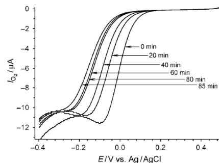
Figure 7: Cyclic voltammograms illustrating the reduction in activity for the ORR in 0.1 M H 2 SO 4 at a Au electrode treated with Fenton’s reagent for various times. Reprinted from ref 96 with permission of Wiley.
