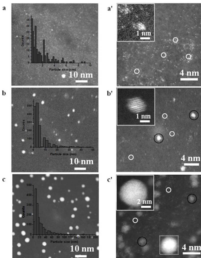
Figure 15: HAADF-STEM images of Pt/GNS samples with increasing number of atomic layer deposition cycles. Reprinted from ref 138 with permission of Nature Publishing Group.
