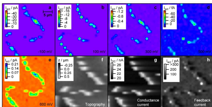
Figure 10: SECCM images of Pt nanoparticles on an individual carbon nanotube biased at different potentials illustrating reactivity maps and the corresponding topography of the sample. Also shown is the conductance recorded between the two barrels of the SECCM probe and the ac component of the conductance current (feedback current). Reprinted with permission from ref 113. Copyright (2011) American Chemical Society.
