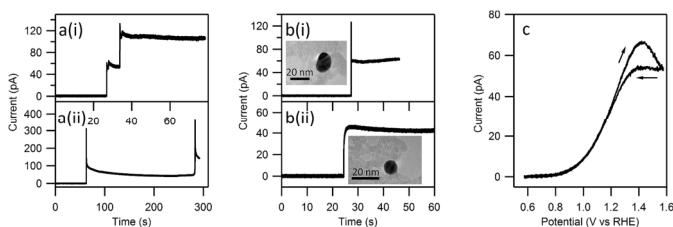
Figure 11: Illustration of the landing of multiple and single Au NPs on a carbon coated TEM grid. After detection of a single landing event (b) the same nanoparticle could be imaged in the TEM and its electrocatalytic behaviour for the oxidation of hydrazine could be investigated (c). Reprinted with permission from ref 120. Copyright (2012) American Chemical Society.
