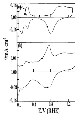
Figure 4: Cyclic voltammograms recorded in 1 M H 2 SO 4 at a Pt wire before (a) and after (b) thermal activation via resistive heating in a N 2 /H 2 atmosphere followed by quenching. The temperature of the wire was ~ 1310 °C. Reprinted from ref 63 with permission of Springer.
