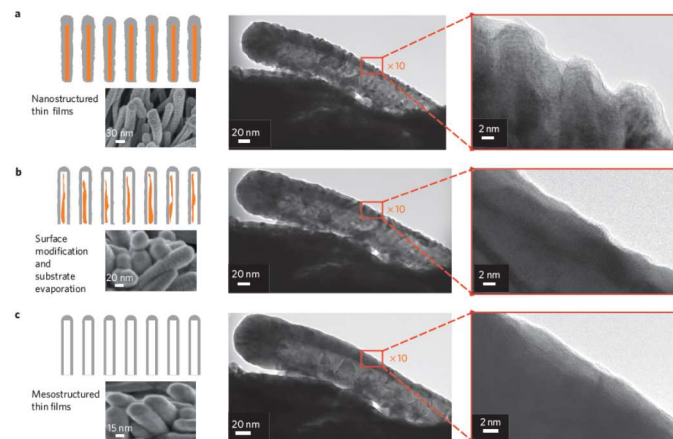
Figure 14: In situ transformation from a nanostructured into mesostructured PtNi thin film during annealing from RT to 400°C. HRTEM images shows this process occurring at a single nanowhisker. Reprinted from ref 135 with permission of Nature Publishing Group.
