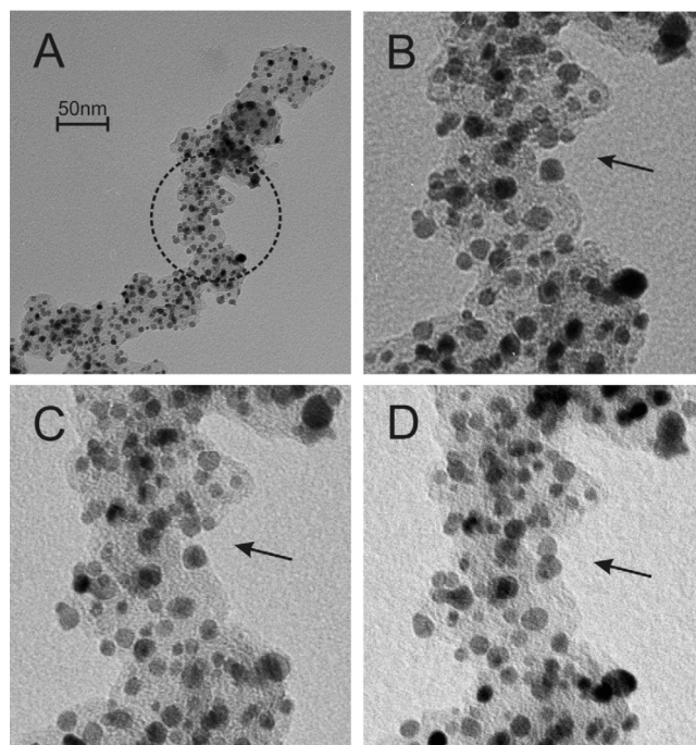
Figure 13: IL-TEM images of a commercial Pt/C catalyst before (A+B) and after (C+D) electrochemical cycling showing the movement and agglomeration of Pt catalyst particles. Reprinted from ref 122 with permission of Elsevier.
