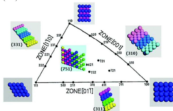
Figure 1: Unit stereographical triangle of fcc single-crystal surfaces and the corresponding models of surface atomic arrangements. Reprinted from ref 52 with permission of the Royal Society of Chemistry.
