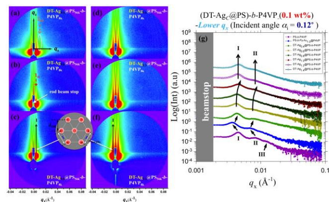
Fig. 5 (a–f) 2D GISAXS patterns and (g) in-plane GISAXS profiles of the (DT-Ag c @PS)- b -P4VP composites incorporating DT-Ag NPs with weight ratios of the latter ( c ) of (a) 0.4, (b) 0.6, (c) 0.8, (d) 1.0, (e) 1.2, and (f) 1.4. In (a), q_x and q_z are the in-plane and out-of-plane components of the momentum transfer vector q , respectively. The peaks of the structure factor, denoted I , II , and III , arose from the micelle-to-micelle distance, d_{\text{micelle}} . The arrows in the in-plane profiles indicate scattering peaks from the hexagonally ordered copolymer micelle cores in the lower- q_x region.
