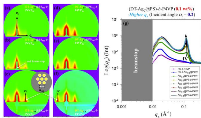
Fig. 7 (a–f) 2D GISAXS patterns and (g) in-plane GISAXS profiles for thin films of the (DT-Ag c @PS)- b -P4VP composites incorporating DT-Ag NPs, with concentrations of the latter ( c ) of (a) 0.4, (b) 0.6, (c) 0.8, (d) 1.0, (e) 1.2, and (f) 1.4. In (a), q_x and q_z are the in-plane and out-of-plane components of the momentum transfer vector q , respectively. The intensity scale is logarithmic. The peaks of the structure factor, denoted IV, arose from the mean interparticle distance, d_{np} , in the higher- q_x region.
