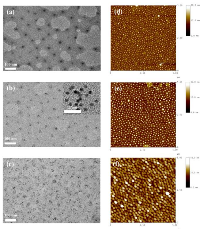
Fig. 3 (a–c) TEM images of the (a) \text{PS}_{56k}\text{-}b\text{-P4VP}_{8k} , (b) \text{PS-}b\text{-}(\text{Py-Au}_{1.0}\text{@P4VP}) , and (c) (\text{DT-Ag}_{1.0}\text{@PS})\text{-}b\text{-}(\text{Py-Au}_{1.0}\text{@P4VP}) composites. The dark spots in (a) and the light spots in (b) and (c) represent P4VP cores, in the absence and presence of the Py-Au NPs; the dark spots in (b) and (c) represent the Py-Au NPs. Inset to (b): Detailed view of single Py-Au/P4VP cores and their surroundings. (d–f) Representative AFM patterns of (d) the neat \text{PS}_{56k}\text{-}b\text{-P4VP}_{8k} thin film and (e) the \text{PS-}b\text{-}(\text{Py-Au}_{1.0}\text{@P4VP}) and (f) (\text{DT-Ag}_{1.0}\text{@PS})\text{-}b\text{-}(\text{Py-Au}_{1.0}\text{@P4VP}) BCP/metal NP composite thin films. Bright spots (local high lands) in (d) and (e) represent P4VP and Py-Au/P4VP cores, respectively. Bright zones (local high lands) and bright spots (2D hexagonal packing) in (f) represent Py-Au NPs and Py-Au/P4VP cores, respectively.
