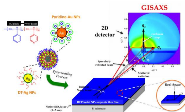
Fig. 1 Schematic representation of the experimental GISAXS setup for analyzing the BCP/metal NP composite thin films featuring micelle structures. The incident beam impinged on the sample surface at a grazing angle \alpha_i ; \alpha_f and 2\theta_f are the exit angles of the X-ray beam with respect to the film surface and to the plane of incidence, respectively; k_i and k_f are the wave vectors of the incident and exit X-ray beams, respectively; q_x , q_y , and q_z are the components of the scattering vector \mathbf{q} ; a strip-shaped beam stop was used to block the strong specular reflection of the X-ray beam and diffuse scattering along the \alpha_f axis. The intensity was monitored by a 2D detector in the x - z plane.
