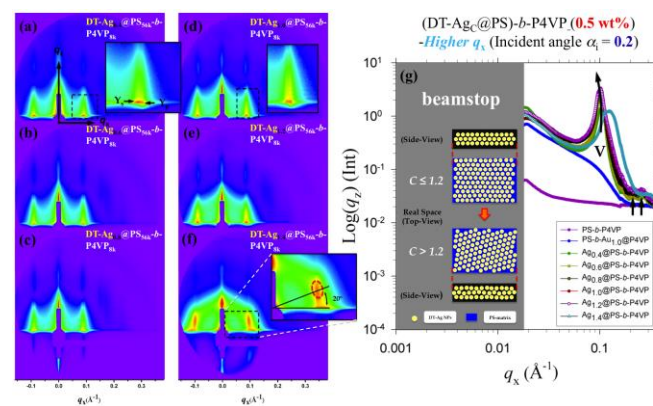
Fig. 9 (a–f) 2D GISAXS patterns and (g) in-plane GISAXS profiles for thin films of the (DT-Ag c @PS)- b -P4VP composites spun from toluene solutions at a concentration of 0.5 wt%, with concentrations of the DT-Ag NPs ( c ) of (a) 0.4, (b) 0.6, (c) 0.8, (d) 1.0, (e) 1.2, and (f) 1.4. In (a), q_x and q_z are the in-plane and
