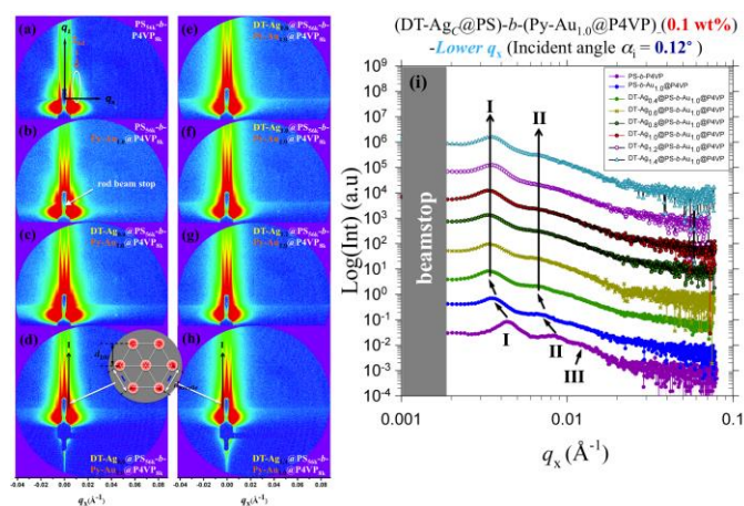
Fig. 4 (a–h) 2D GISAXS patterns and (i) in-plane GISAXS profiles of the (a) neat PS 56k - b -P4VP 8k thin film and of (b–h) thin films of the (DT-Ag c @PS)- b -(Py-Au 1.0 @P4VP) composites incorporating Py-Au and DT-Ag NPs, with weight ratios of the latter ( c ) of (b) 0, (c) 0.4, (d) 0.6, (e) 0.8, (f) 1.0, (g) 1.2, and (h) 1.4. In (a), q_x and q_z are the in-plane and out-of-plane components of the momentum transfer vector q , respectively. The peaks of the structure factor, denoted I , II , and III , arose from the micelle-to-micelle distance, d_{\text{micelle}} . The arrows in the in-plane profiles indicate scattering peaks from the hexagonally ordered copolymer micelle cores in the lower- q_x region. Insets to (d) and (h): Curves analyzed using a 2D hexagonal lattice function.
