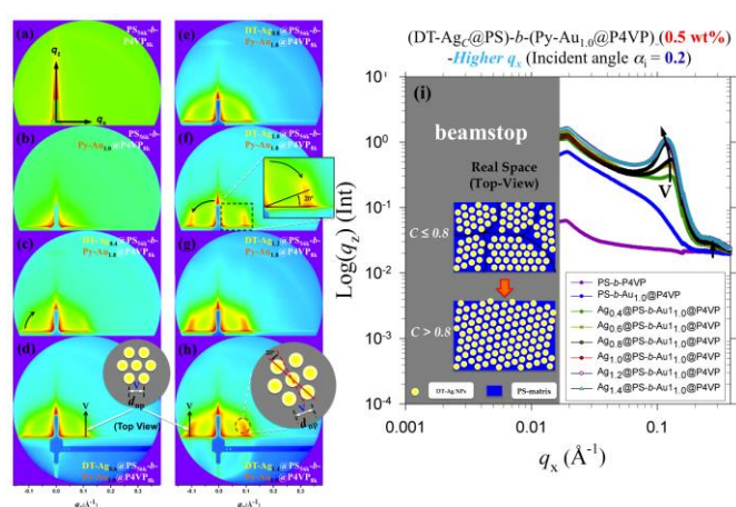
Fig. 8 (a–h) 2D GISAXS patterns and (i) in-plane GISAXS profiles for (a) the neat PS 56k - b -P4VP 8k thin film and (b–h) thin films of the (DT-Ag c @PS)- b -(Py-Au 1.0 @P4VP) composites
