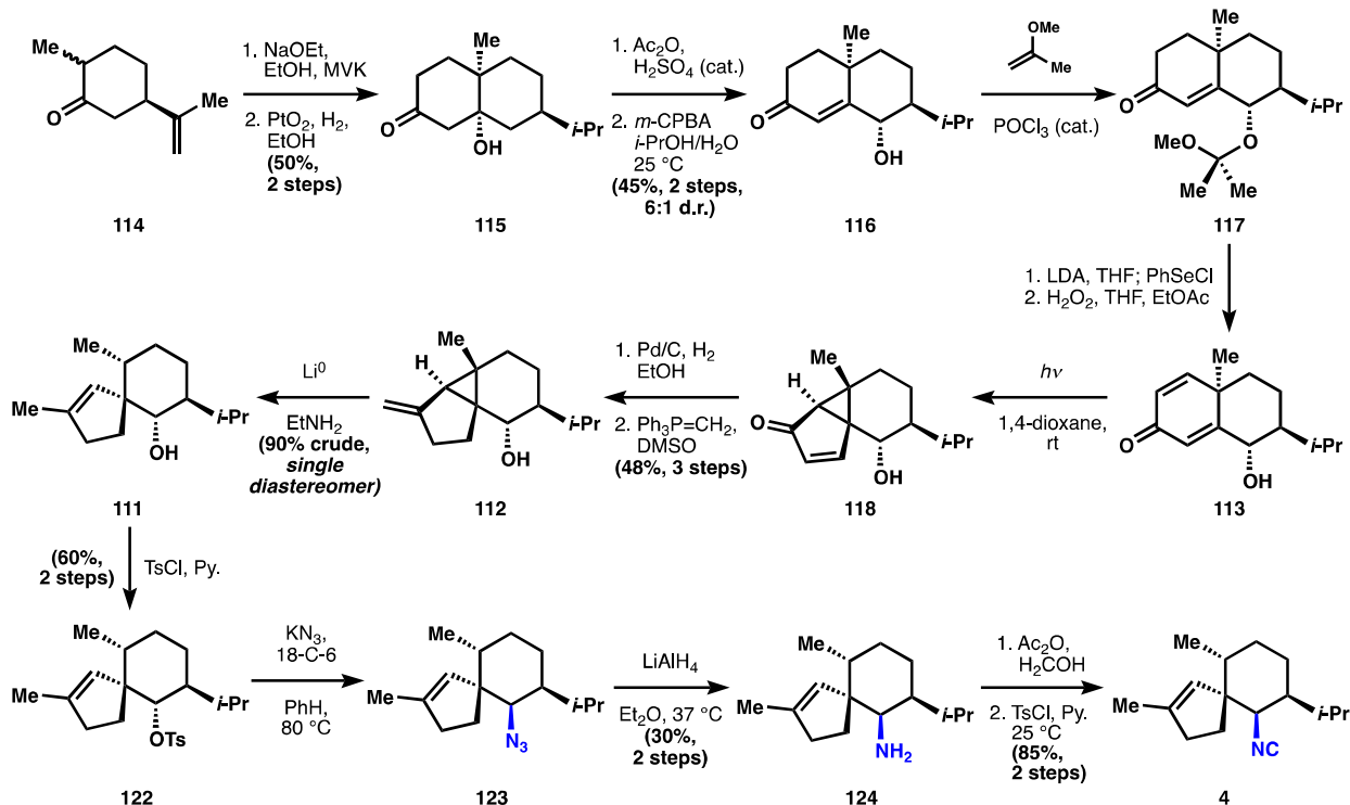
Figure 9. Caine's synthesis of (-)-axisonitrile-3.
