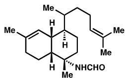
51: caverene C
