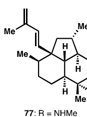
77: R = NHMe 78: R = NCHO
