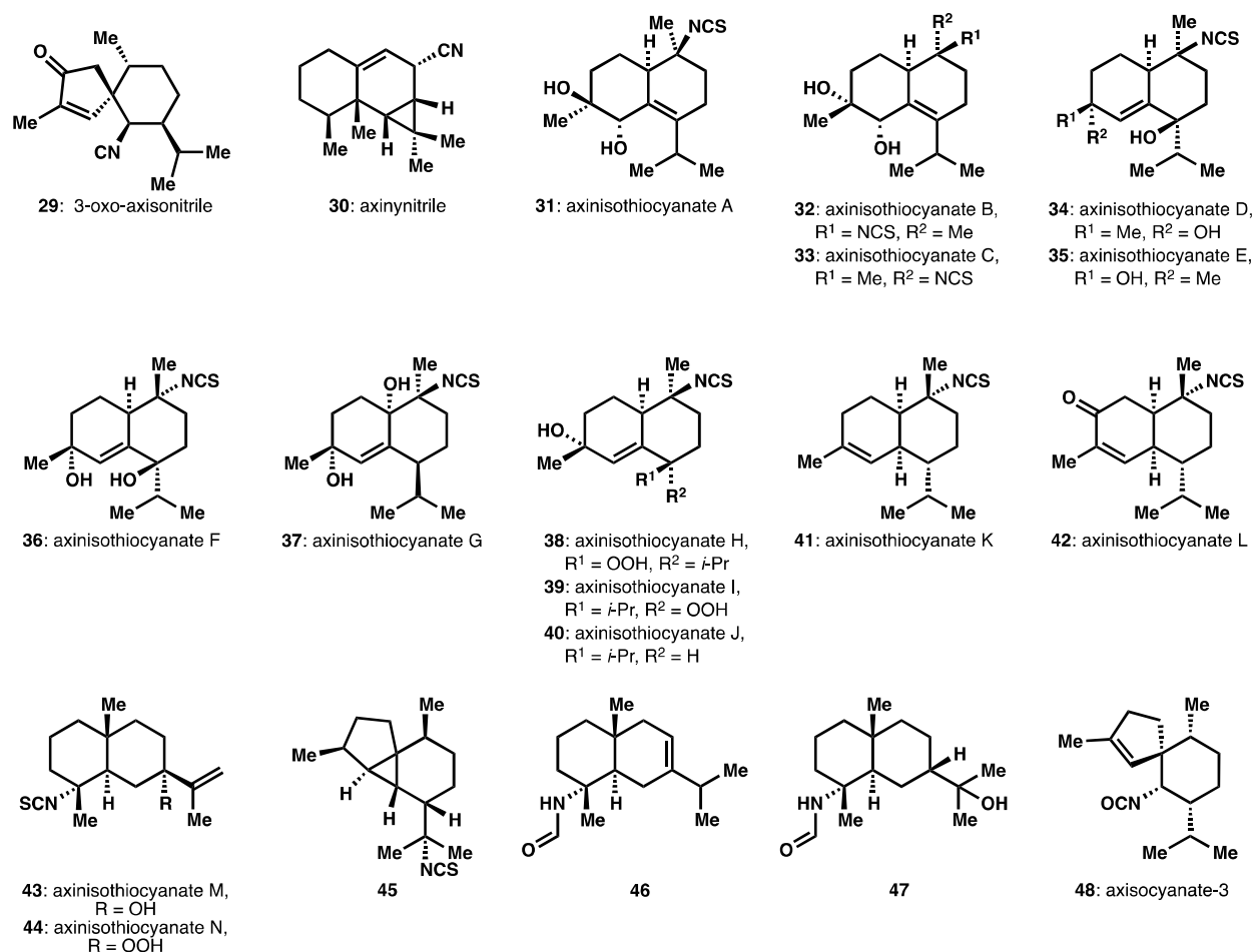
Figure 3: Sesquiterpenes isolated from 2004-2014.
