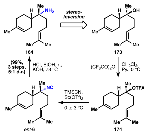
Figure 18. Shenvi's route to (-)- 164 via stereoinversion of 173 .
