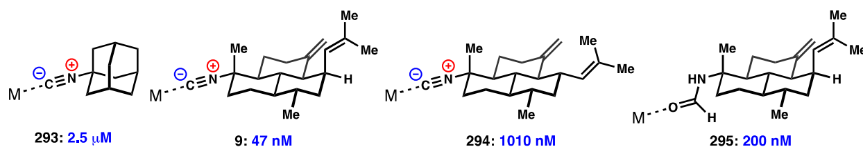
Figure 36. Metal binding alone does not explain SAR.
