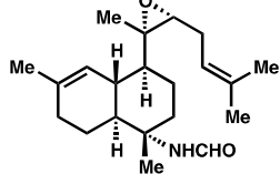
52: caverene D
