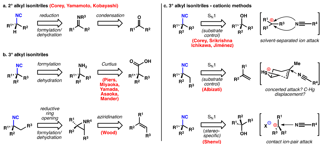
Figure 6. Retrosynthetic strategies to generate stereogenic sec - and tert -alkyl isonitriles.
