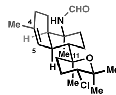
11: Kalihinene X
