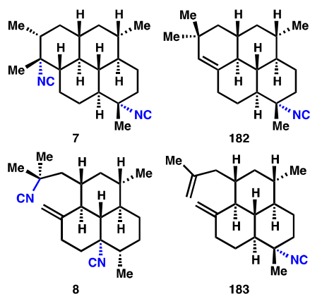
Figure 20. Amphilectenes and adocianes.
