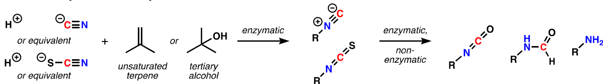
5: 10-Isocyano-4-cadinene
