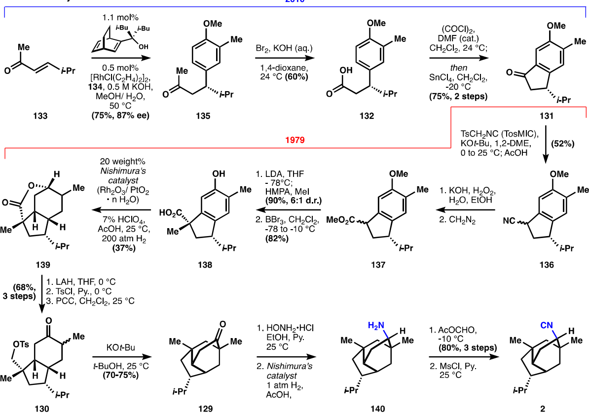
Figure 12a. Corey's analysis of 2 ; b. Corey's chemical synthesis of 2 .
