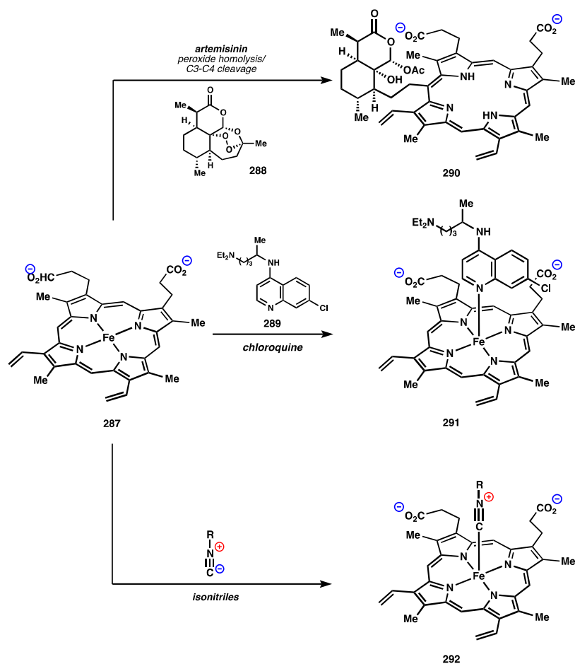
Figure 34: Small molecule/heme interactions.
