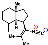
4: Axisonitrile-4
