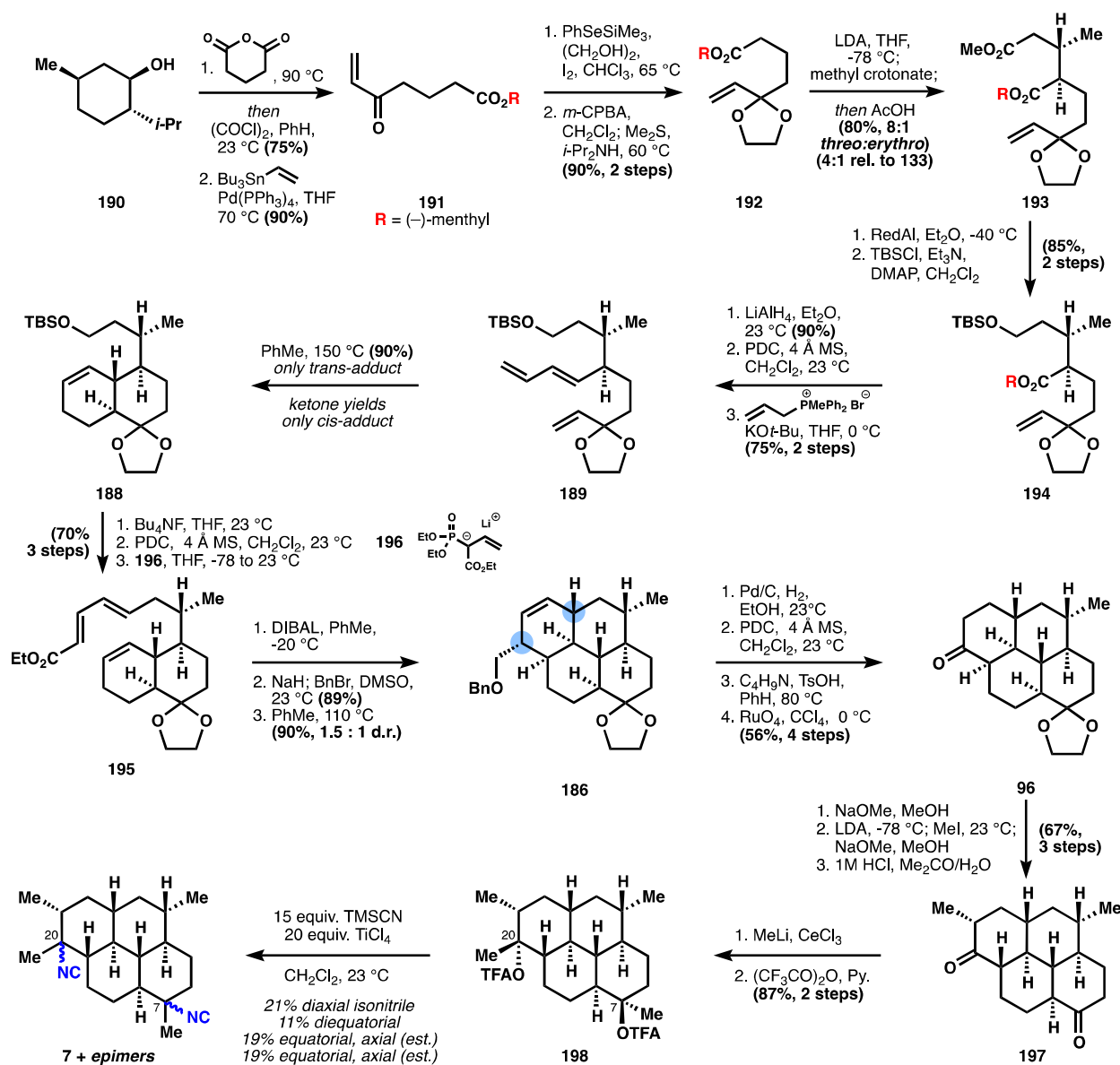
Figure 22. Corey's chemical synthesis of 7 .
