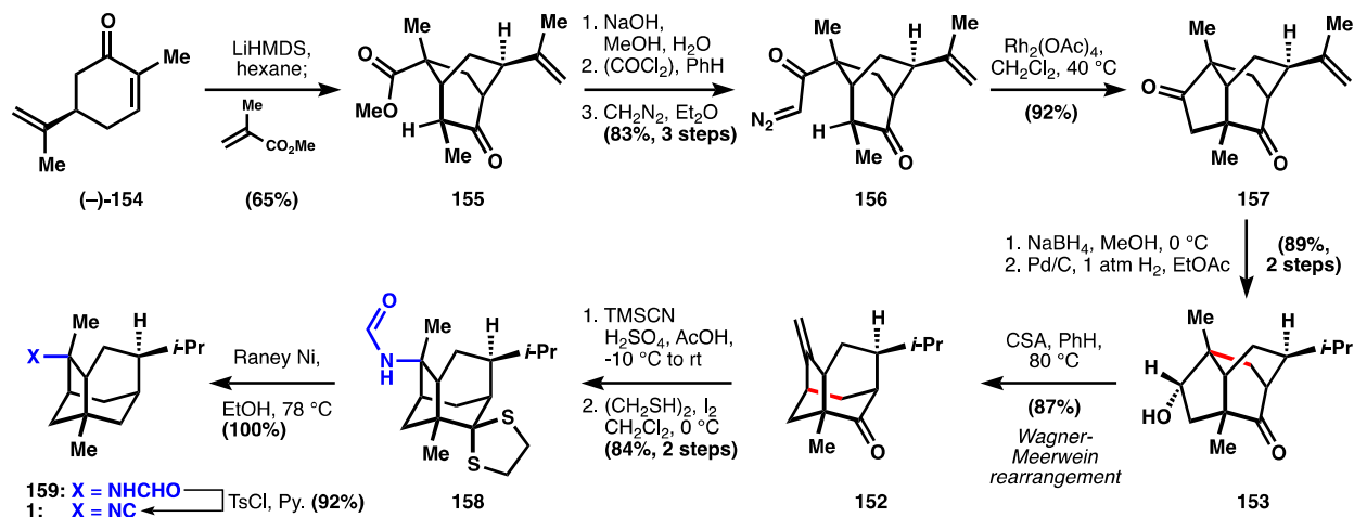
Figure 14a. Srikrishna's analysis of 1 ; b. Srikrishna's chemical synthesis of 1 .
