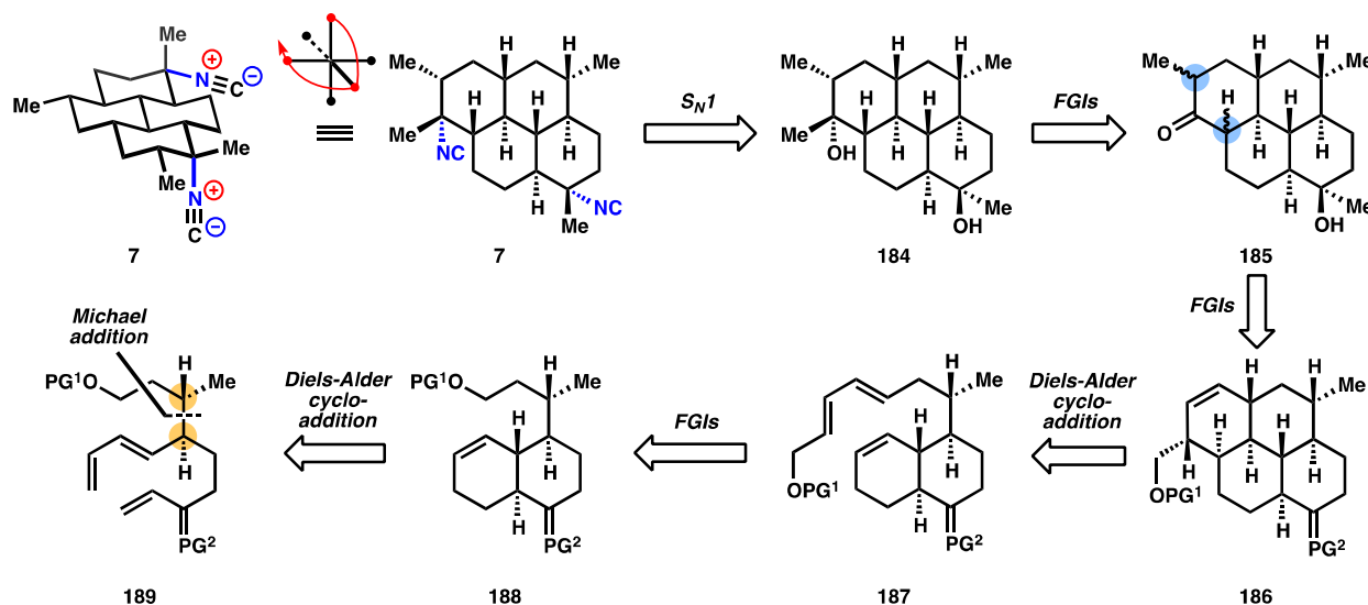
Figure 21. Corey's retrosynthetic analysis of (+)-7,20-diisocyanoadociane ( 7 ).
