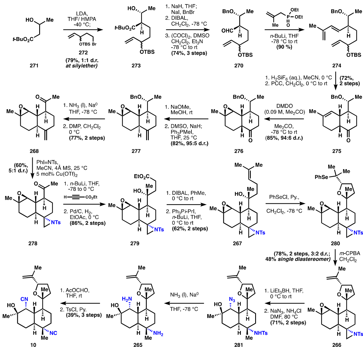
Figure 31. Wood's synthesis of kalihinol C ( 10 ).
