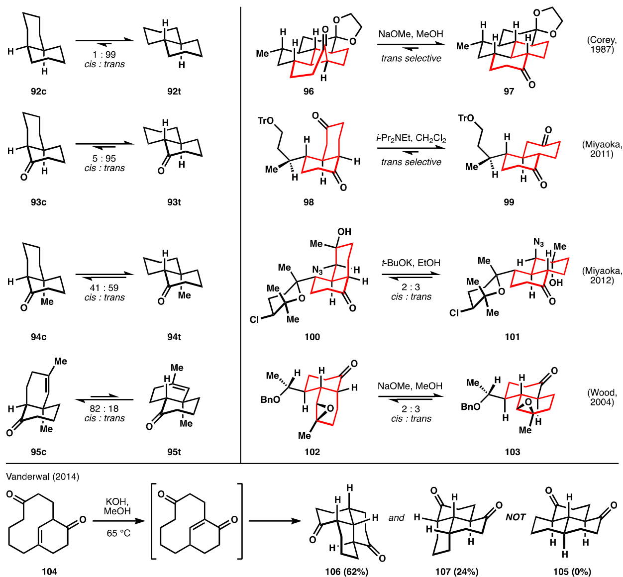
Figure 7. Cis -/ trans -isomerism of substituted decalins.
