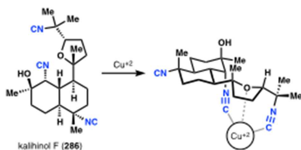
Figure 33. Kalihinol F copper chelation model.
