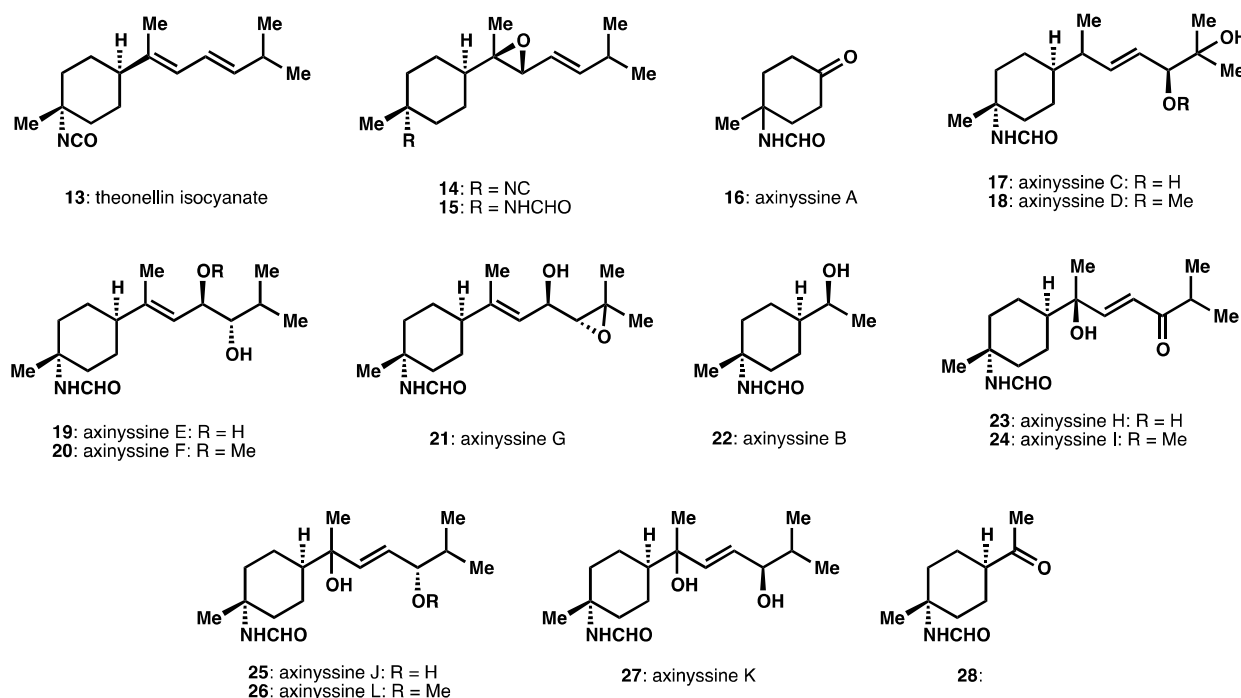
Figure 2: Bisabolene sesquiterpenes isolated from 2004-2014.
