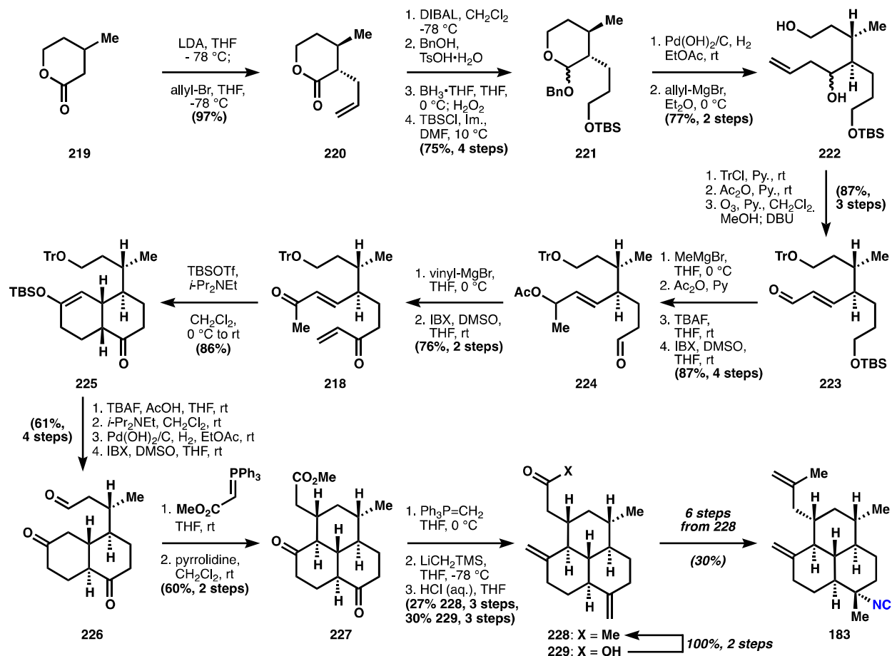
Figure 25a. Miyaoka's analysis and b. synthesis of amphilectene 183 .
