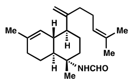
49: caverene A
