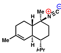
5: 10-Isocyano-4-cadinene
