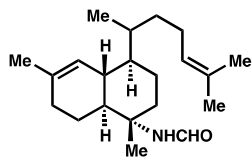
50: caverene B
