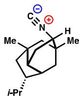
2: 9-Isocyanopupukeanane
