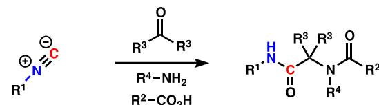
Figure 1: (A) Isonitrile-Containing Natural Products (B) General Biosynthetic Scheme (C) Representative Isonitrile Reactivity.
