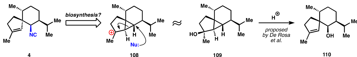
Figure 8. A hypothetical biosynthesis of 4 based on related terpene relationships.
