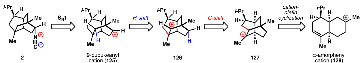
Figure 11. Hypothesized biosynthesis of 2 .
