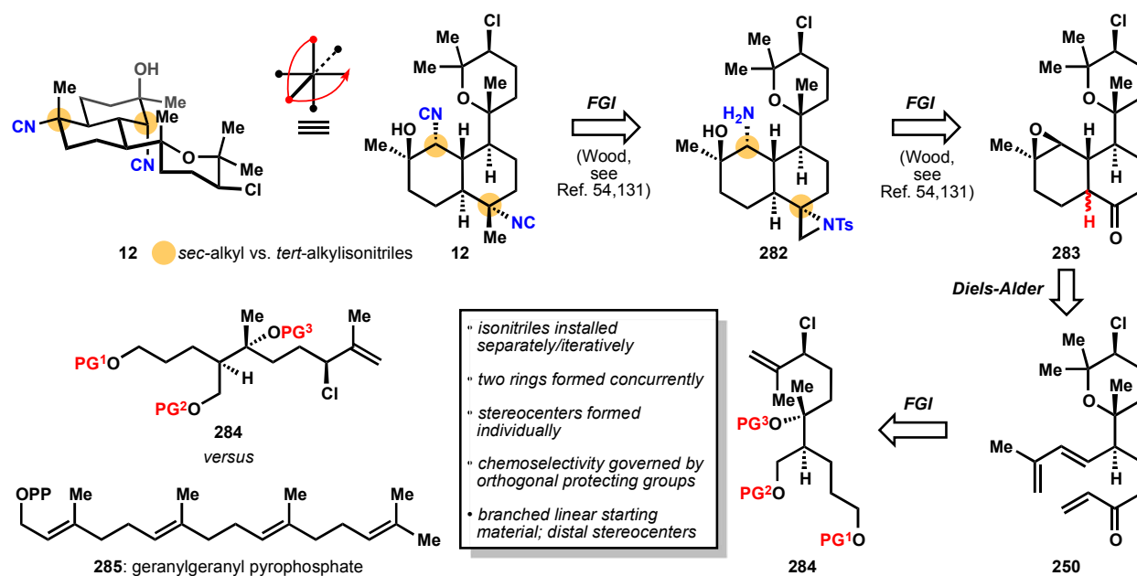
Figure 32. Miyaoka's analysis of 12 relies on preinstalled stereocenters (e.g. 284 ) prior to ring building, in contrast to the hypothesized biosynthesis of 12 from 285 .
