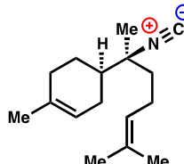
6: Isocyanobisabolene
