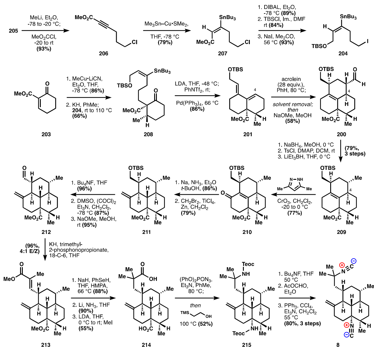
Figure 24. Piers' synthesis of 8 .
