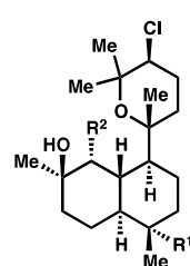
64: kalihinol P: R 1 = NC, R 2 = NCS 65: kalihinol S: R 1 = NCS, R 2 = NHCHO
