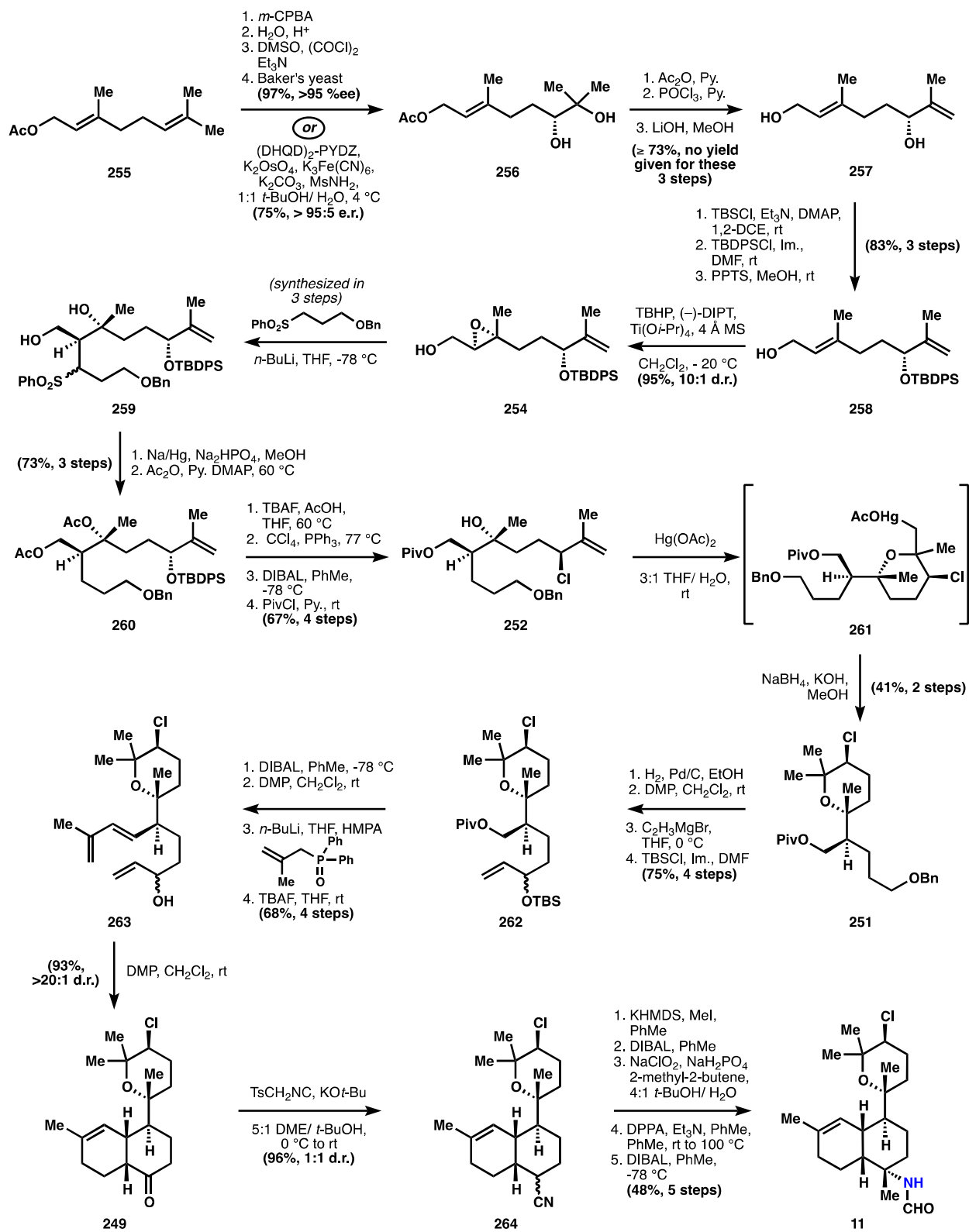
Figure 29. Miyaoka's and Yamada's synthesis of 11.
