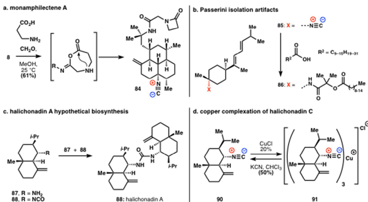
Figure 5a. Semisynthesis of monamphilectine A. b. Passerini isolation artifacts. c. Proposed biosynthesis of urea-linked sesquiterpenes. d. Copper complexation and decomplexation of isocyanoterpenes.
