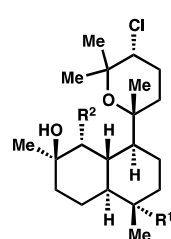
61: kalihinol O: R 1 = NCS, R 2 = NC 62: kalihinol Q: R 1 = NC, R 2 = NCS 63: kalihinol R: R 1 = NCS, R 2 = NCS
