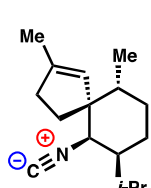
3: Axisonitrile-3
