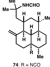
74: R = NCO 75: R = NCS
