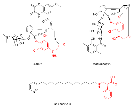
Fig. 2.3. Structures of C-1027 chromophore, maduropeptin, and nakinadine B. \beta -Amino acid moiety in red.
