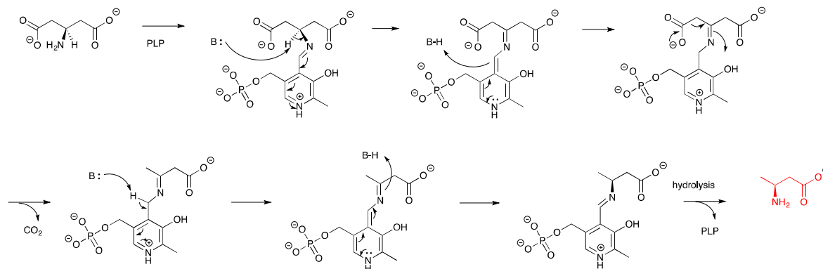
Fig. 3.4. Reaction mechanism of pyruvoyl-dependent and PLP-dependent decarboxylases to produce \beta -amino acids, such as \beta -aminoisobutyrate and \beta -aminobutyrate.
