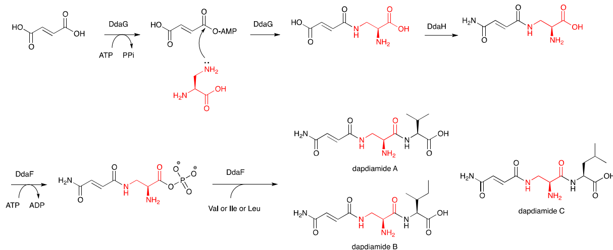
Fig. 4.4. Biosynthesis of dapdiamides.
