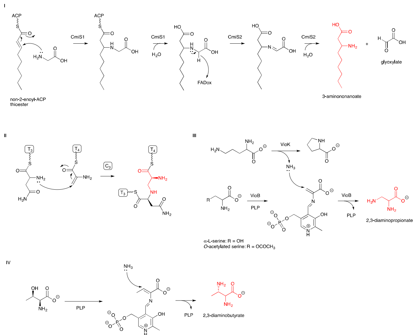
Fig. 3.5. Mechanism of Michael addition of ammonia or amino acid amino group to \alpha,\beta -
