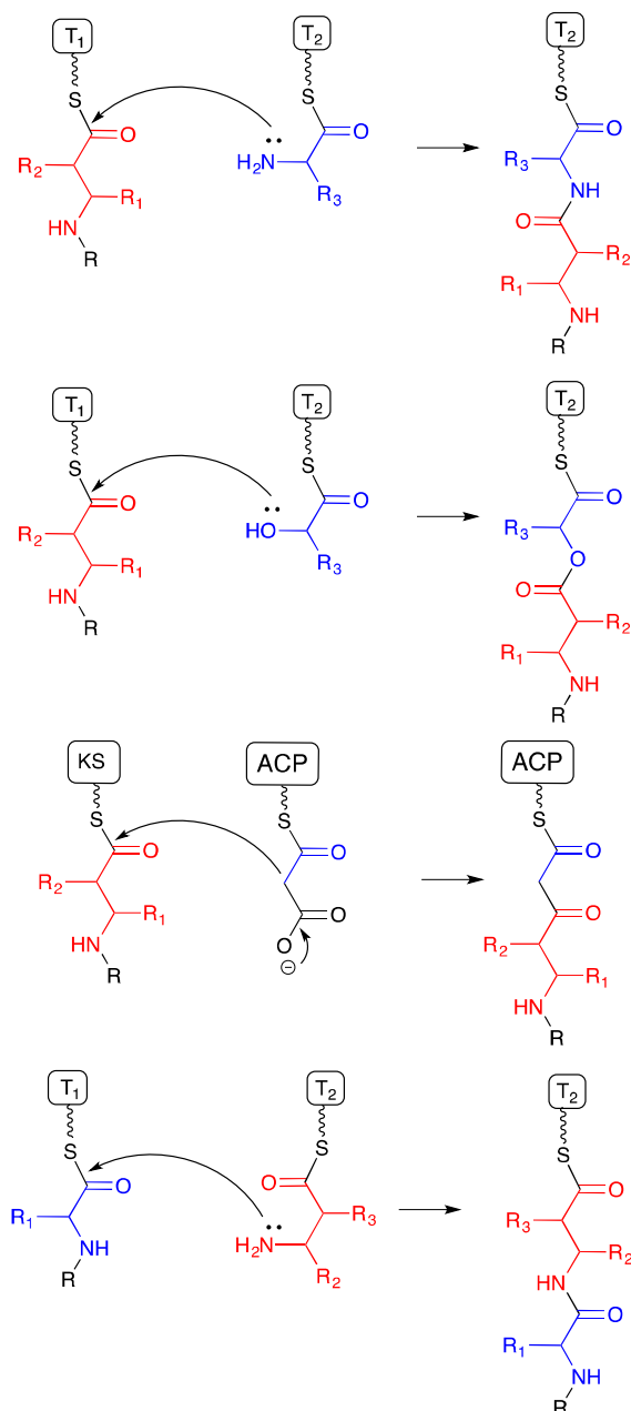
Fig. 1. Condensation mechanism of \beta -amino acid between carboxylates and other nucleophiles (Upper three schemes), and \beta -amino group and carboxylates (Bottom). \beta -Amino acids and counter substrates in red and blue, respectively.
