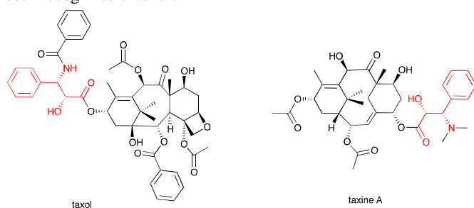
Fig. 2.4. Structures of taxol and taxine A. \beta -Amino acid moiety in red.
