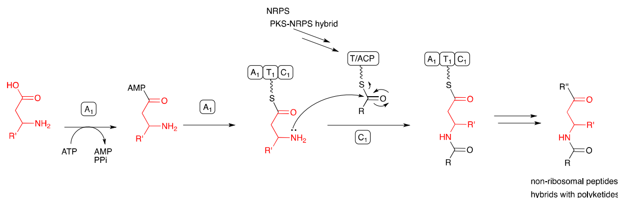
Fig. 4.3. Biosynthesis of \beta -amino acid-containing nonribosomal peptides and nonribosomal peptide-polyketide hybrids.
