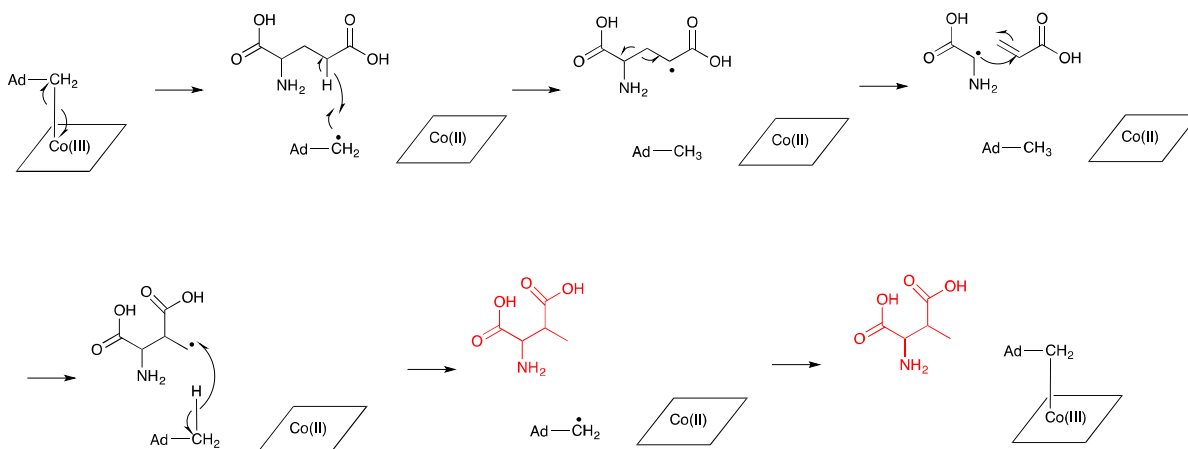
Fig. 3.3. Reaction mechanism of adenosylcobalamin-dependent glutamate mutase.
