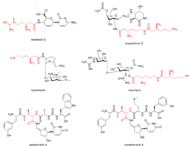
Fig. 2.5. Structures of sugar- \beta -amino acid hybrid compounds. \beta -Amino acid moiety in red.
