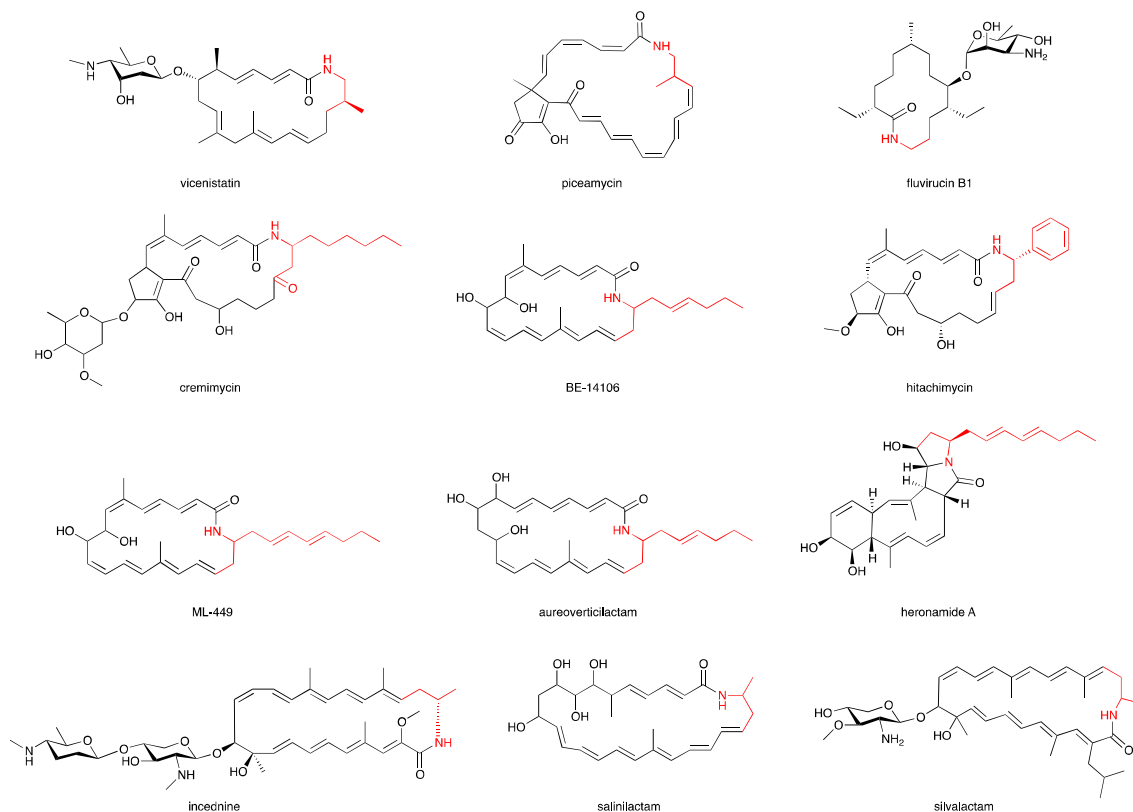
Fig. 2.2. Structures of macrolactam antibiotics. \beta -Amino acid moiety in red.
