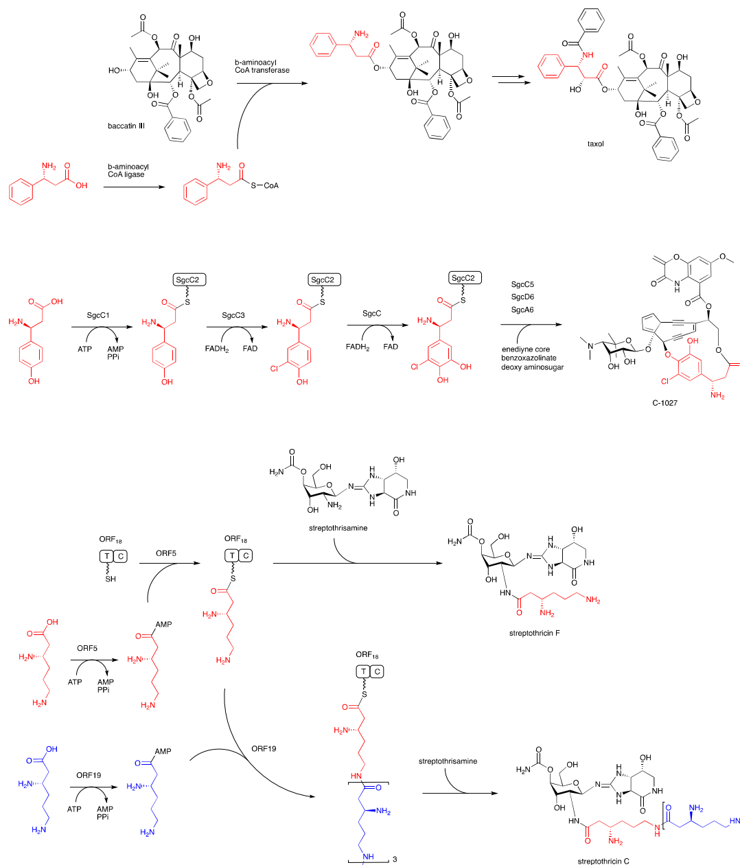
Fig. 4.1. Acyl transfer reactions of \beta -amino acids to hydroxyl or amino group acceptors. (I) Installation of \beta -phenylalanine into taxol. (II) Installation of (S)-3-chloro-4,5-dihydroxy- \beta -phenylalanine into C-1027. (III) Installation of poly- \beta -lysine into streptothricin. \beta -Lysine (in red) activated by ORF 5 is initially loaded on the T (PCP) domain of ORF 18. \beta -Lysine molecules (in blue) activated by ORF 19 are then used as extender units for elongation reactions of \beta -lysine oligopeptide.
