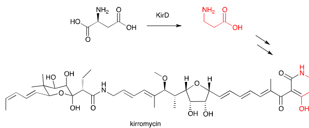
Fig. 3.1. Biosynthesis of kirromycin. \beta -Alanine moiety in red.
