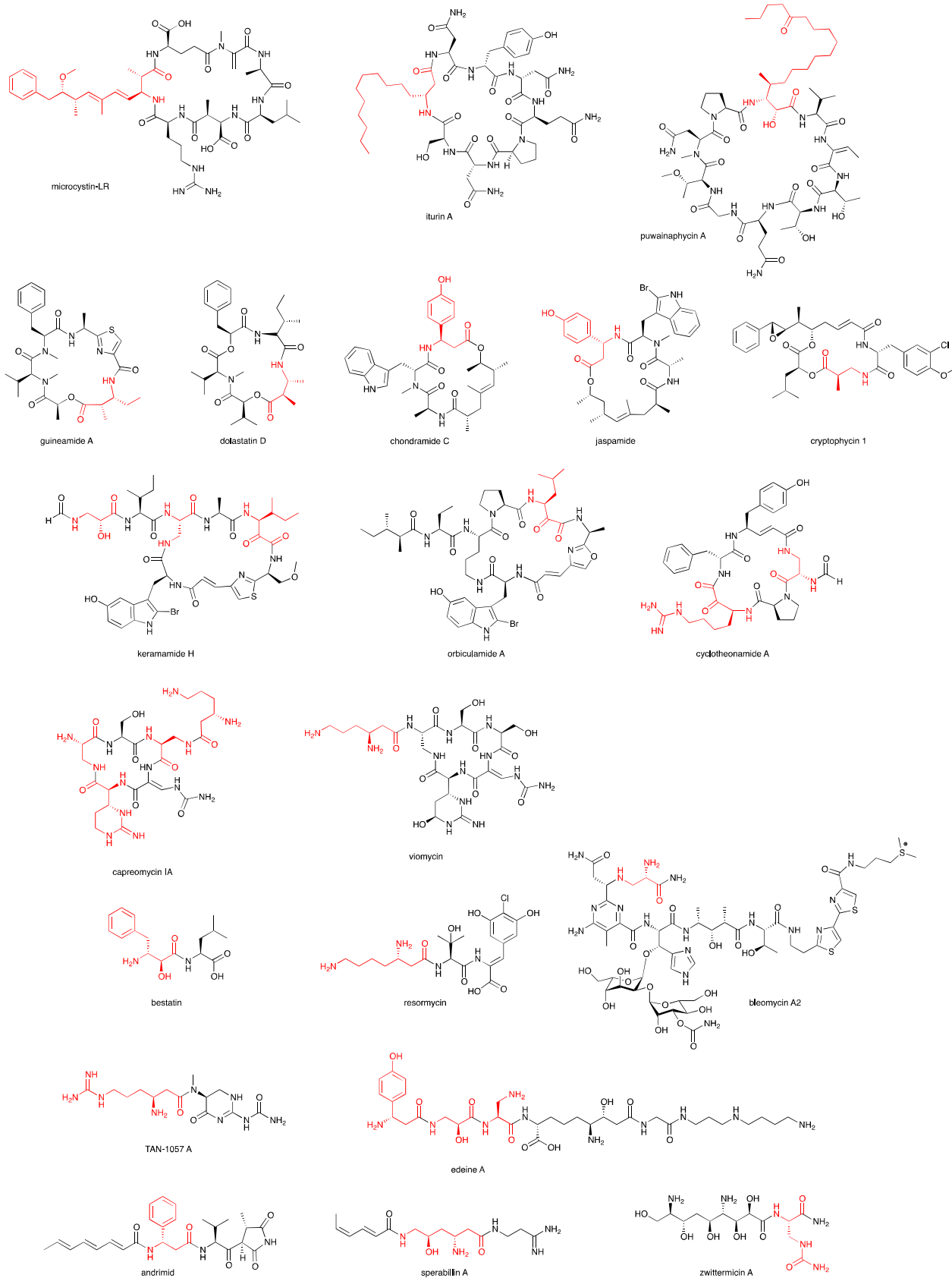
Fig. 2.1. Structures of \beta -amino acid-containing nonribosomal peptides and nonribosomal peptide-polyketide hybrids. \beta -Amino acid moiety in red.
