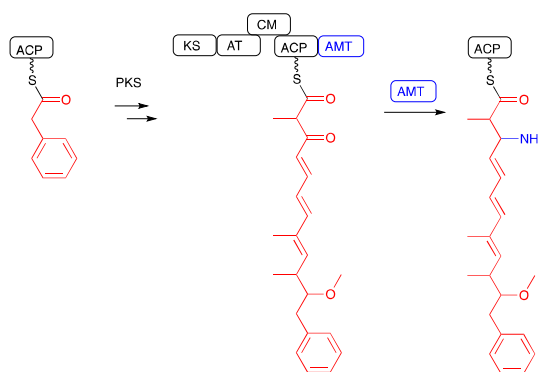
Fig. 3.6. Biosynthesis of microcystin-LR. \beta -Ketocarboxylate is transaminated by PLP-
