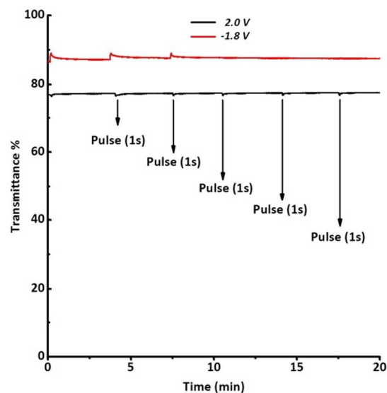
25 Fig.7 Open circuit memory of PTPTFlo/PEDOT ECD recorded at 580 nm, +2.0 V and -1.8 V pulse were applied for 1 s every 200 s
