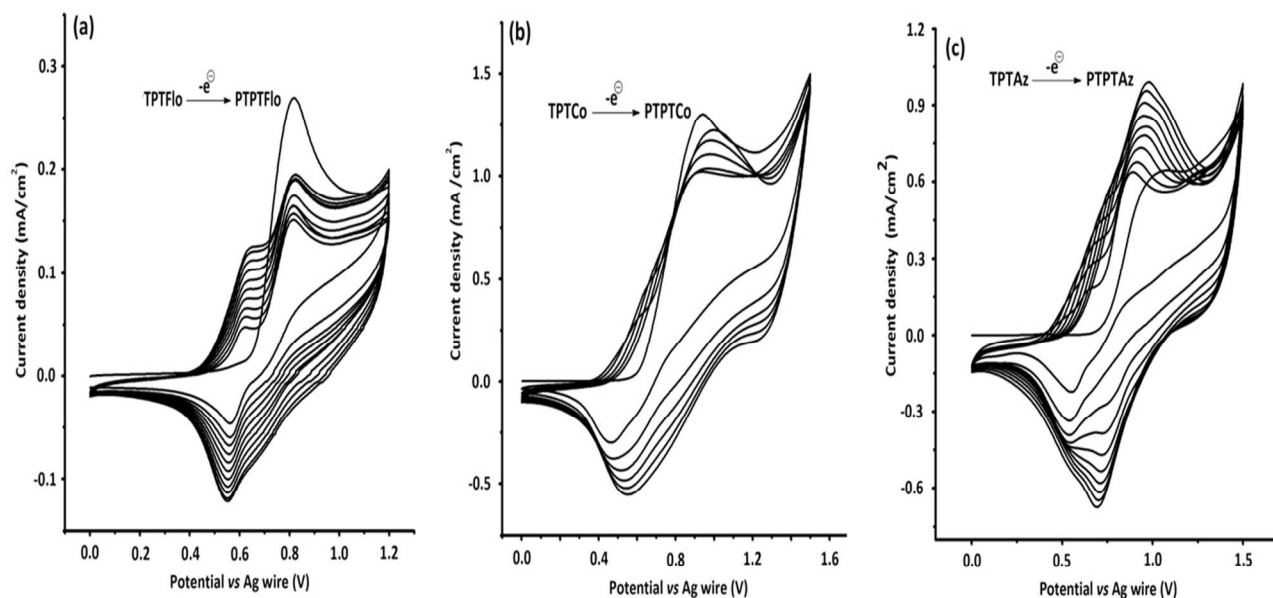
Fig.2 Repeated potential scan polymerization of (a) TPTFlo (b) TPTCo and (c) TPTAz in 0.1 M LiClO 4 / NaClO 4 /DCM/ACN (5:95,v:v) solution at 100 mV s -1 scan rate
