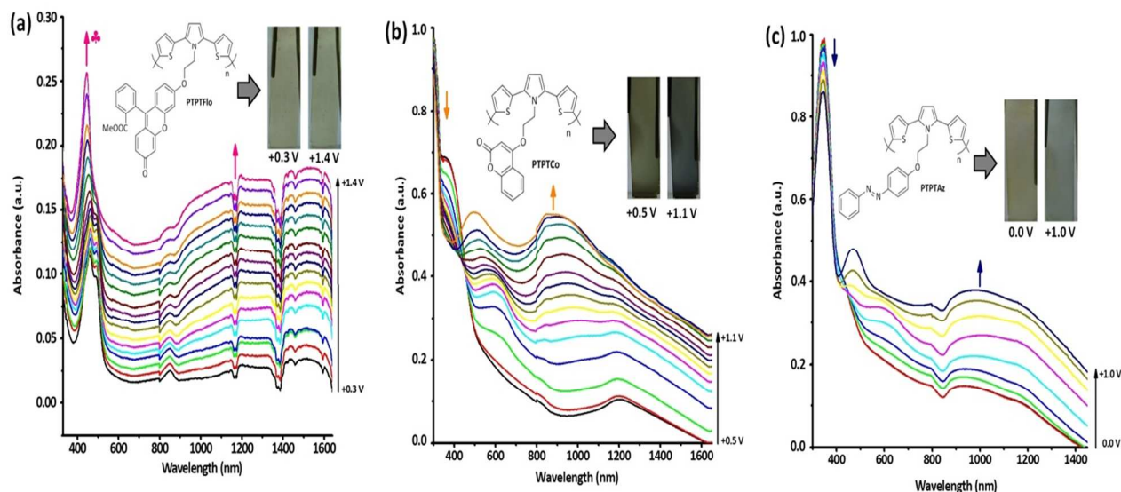
Fig. 4 Electronic absorption spectra of (a) PTPTFlo (b) PTPTCo (c) PTPTAz in 0.1 M NaClO 4 -LiClO 4 /ACN electrolyte solution between +0.3 V and +1.4 V for PTPTFlo , +0.5 V and +1.1 V for PTPTCo and 0.0 V and +1.0 V for PTPTAz
