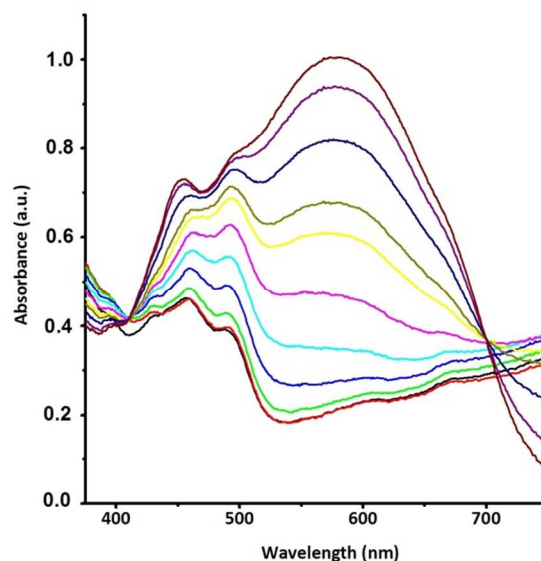
20 Fig.6 Electronic absorption spectra of PTPTFlo/PEDOT ECD at various applied potentials (between -1.8 V and +1.8 V)
