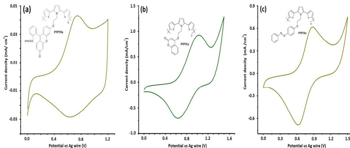
5 Fig.3 Single scan cyclic voltammograms for (a) PTPTFlo (b) PTPTCo and (c) PTPTAz in a monomer free, 0.1 M NaClO 4 /LiClO 4 /ACN solution
