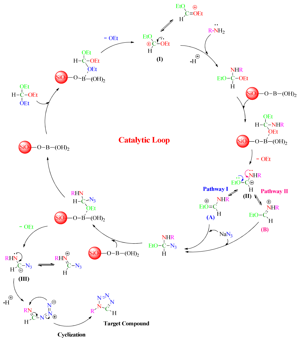
Scheme: 3 Plausible mechanistic catalytic loop for the synthesis of compounds 4 (a-o)
