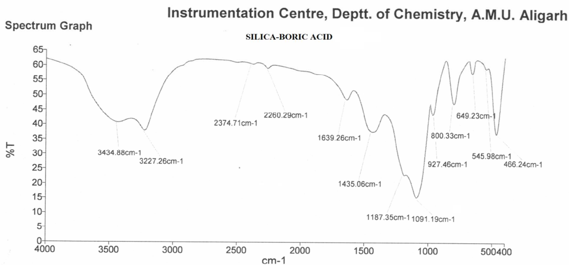
Fig. 2 FT-IR spectrum of catalyst \text{SiO}_2\text{-H}_3\text{BO}_3
