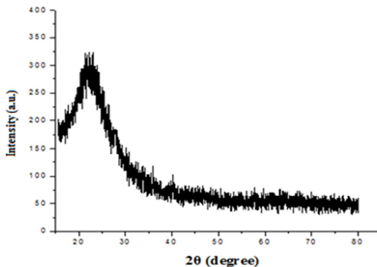
Fig. 3 Powder XRD analysis of catalyst \text{SiO}_2\text{-H}_3\text{BO}_3
