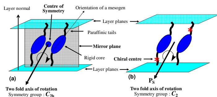
Figure 1. Symmetry in the smectic C (a) and chiral smectic C (b) phases.
