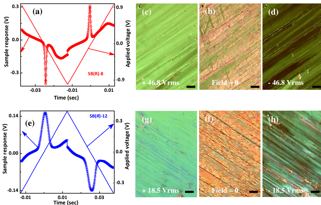
Figure 7. Switching current response peaks obtained upon applying a triangular-wave field for the SmC* phase of mesogens SB(R)-8 (90 °C; 46.8 Vrms, 20 Hz; 09 kΩ; P_s = 108 \text{ nC cm}^{-2} ) (a) and SB(R)-12 , (70 °C; 18.5 Vrms, 20 Hz; 09 kΩ; P_s = 123.8 \text{ nC cm}^{-2} ) (e). Microphotographs of the microscopic textural changes observed under the applied electric field (c,d & g,h) and in the absence of field (b & f) (Bar: 100 μm).
