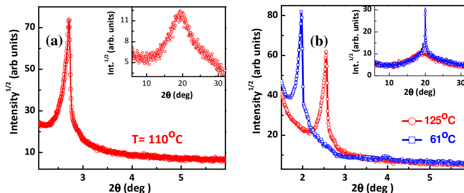
Figure 4. The low-angle and wide-angle (inset) regions of the XRD patterns obtained for the smectic phases of mesogens: (a) the intensity vs 2\theta profile obtained in the SmC* phase of SB(R)-8 ; (b) the intensity vs 2\theta profiles of the SmC* phase (red traces) and SmX phase (blue traces) belonging to SB(R)-12
