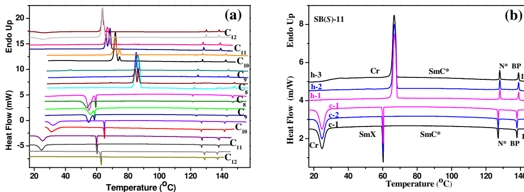
Figure 3. (a) DSC traces obtained during the first heating-cooling cycles at a rate of 5 °C for all the five pairs of enantiomers; (b) DSC traces recorded for the three successive heating (h-1, h-2 & h-3)-cooling (c-1, c-2 & c-3) cycles at a rate of 5 °C for the mesogen SB(S)-11 ; note that the peak positions of all the traces match.
