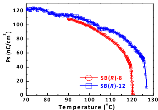
Figure 8. A profile showing the temperature dependence of the P_s in the SmC* phase of compounds SB(R)-8 (red-trace) and SB(R)-12 (blue-trace).
