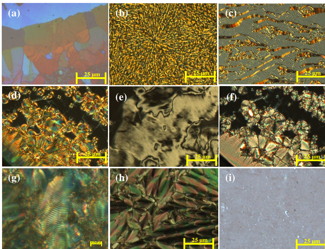
Figure 2. Microphotographs of the optical textural patterns of the mesophases of SB(R)-10 held between two untreated slides (a-f) and treated glass substrates (g-i): (a) The platelet texture of the BP-I/II occurring just below the isotropic phase (141.8 °C); (b) the vague texture obtained for the N* phase at 135 °C; (c) the typical oily streak texture of the N* phase formed at 130 °C when the pattern-(b) was sheared gently; (d) planarly, and homeotropically aligned SmC* phase showing the banded concentric circles as well as banded broken focal-conic texture, and the intense dark-greyish pattern (115 °C), respectively; (e) the schlieren-like pattern found at the edge of the slide for the SmC* phase (115 °C); (f) the distorted circular domains as well as broken focal-conic fan pattern and the pseudo -isotropic texture respectively, observed for the homogeneously and homeotropically oriented SmX phase at 58 °C; (g) the occurrence of a classical fan-shaped texture, featuring equidistant lines on top of it, when the SmC* phase was subjected to planar boundary conditions; (h) the textural pattern seen at 58 °C for the planarly aligned SmX phase where focal-conics, fan-shaped pattern and polygonal domains can be seen; (i) the cloudy texture seen for the homeotropically oriented SmC* phase at 121 °C.
