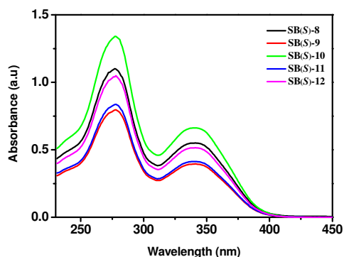
Figure 9. UV-Vis spectrum recorded for the dilute (dichloromethane) solutions of the ( S )-enantiomers
