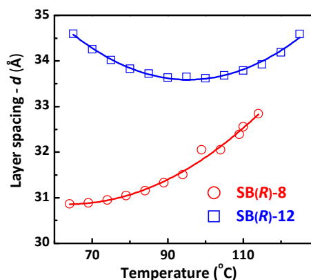
Figure 5. The layer spacing ( d / \text{Å} ) recorded as a function of temperature in the \text{SmC}^* phase of the mesogens SB(R)-8 and SB(R)-12 , as representative cases.
