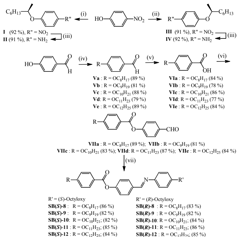
Scheme -I : Synthesis of chiral, three-ring rod-like LCs. Reagents & conditions: (i) ( S )-(+)-2-Octanol, Ph 3 P, DIAD, THF, rt, 18 h; (ii) ( R )-(-)-2-Octanol, Ph 3 P, DIAD, THF, rt, 18 h; (iii) H 2 , (1 atm, balloon), 10 % Pd-C, THF, rt, 4 h; (iv) n -Bromoalkane, anhydrous K 2 CO 3 , DMF, 80 °C, 12 h. (v) Jones reagent, acetone, rt, 1 h; (vi) 4-Hydroxybenzaldehyde, DCC, DMAP, THF, rt, 4 h. (vii) II & IV , EtOH, AcOH, reflux, 5 h
