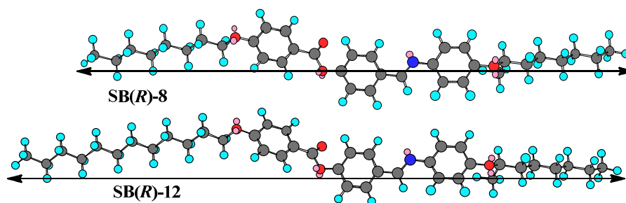
Figure 6. Energy-minimized ball-and-stick models of the most extended form with an all-trans conformation of the alkoxy chains (derived from MM2 of the ChemBioDraw Ultra 12.0) of the SB(R)-8 and SB(R)-12 with respective theoretical molecular lengths of 37.5 Å and 42.5 Å.
