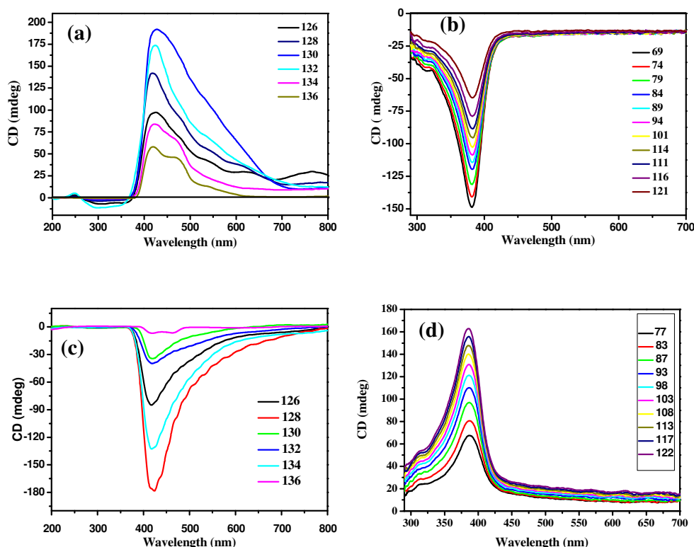
Figure 10. CD spectra recorded as a function of temperature in the N^* (a and c) and SmC^* (b and d) phases exhibited by the enantiomer SB(R)-9 and SB(S)-9
