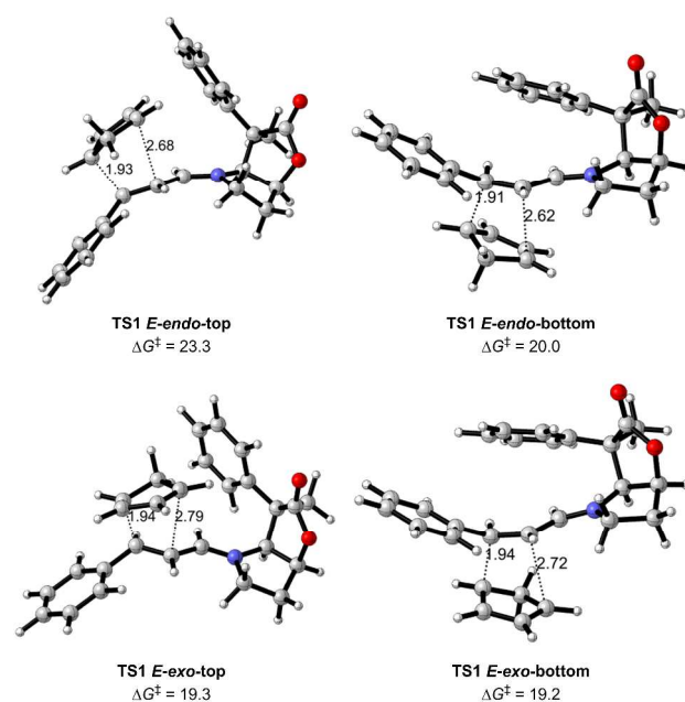
Fig. 4 Transition states for the reaction between CP and iminium ion 1-E with Gibbs energies of activation in kcal/mol and relevant distances in Å.
