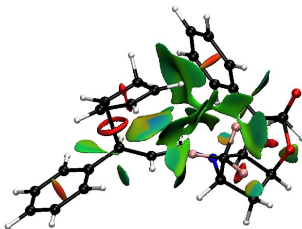
Fig. 7 Color-coded noncovalent interactions (NCI) surfaces (attractive decreasing from blue to green, repulsive increasing from yellow to red) for TS8- E-exo-top .
