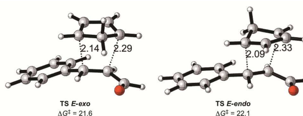
Fig. 2 Transition states for the uncatalyzed Diels-Alder reaction with Gibbs energies of activation in kcal/mol relative to the adduct formed by cyclopentadiene and cinnamaldehyde, and selected distances in Å.
