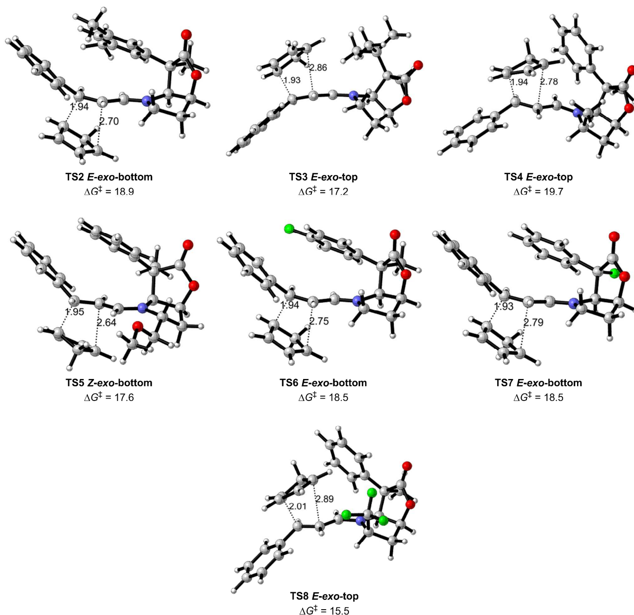
Fig. 6 The preferred transition states (TS2 to TS8) for entries 2 to 8 (Table 1) with Gibbs energies of activation in kcal/mol, and selected distances in Å.
