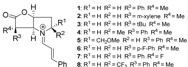
Fig. 5 An overview of investigated catalysts 1-8.
