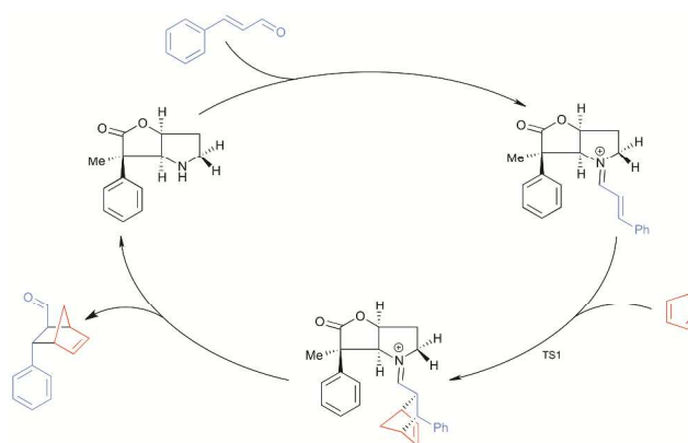
Scheme 3 The catalytic cycle of the organocatalysed Diels-Alder reaction between CP and the E -isomer of the iminium ion formed from cinnamaldehyde and BL.
