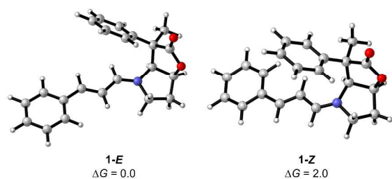
Fig. 3 E/Z iminium ions formed by the condensation of 1 and cinnamaldehyde with relative Gibbs energies in kcal/mol.
