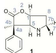
Fig. 1 Bicyclic lactone (BL) used as organocatalyst.
