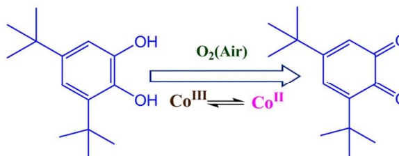
Scheme 1 A schematic representation of catechol oxidation
