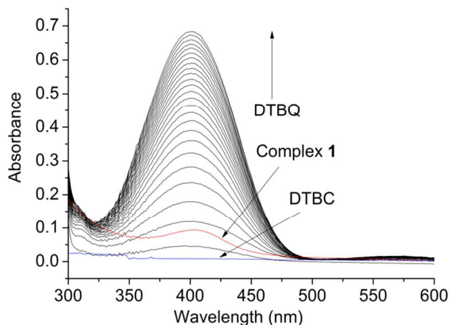
Fig. 4 Increase in absorbance around 400 nm, after addition of 600 equivalents of DTBC dissolved in acetonitrile to a 10^{-5} M solution of 1 in DMF. Spectra were recorded every 5 min.
