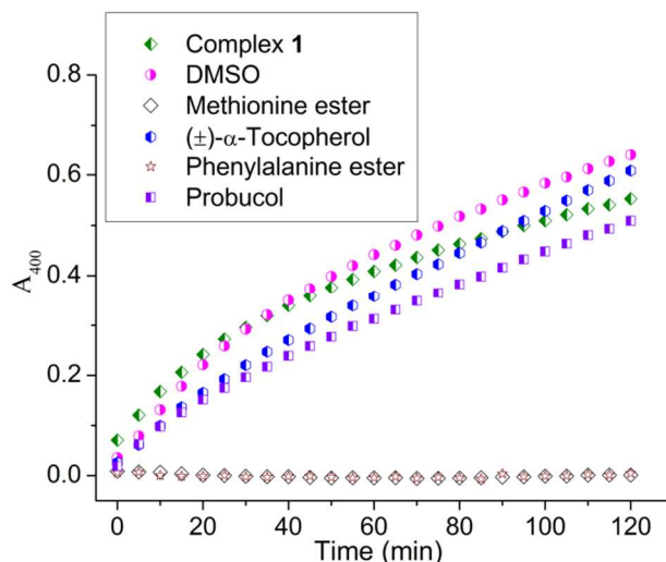
Fig. 6 Inhibition study of catechol oxidation probed by monitoring the change in absorbance at 400 nm. Reaction condition: 500 molar equivalent of DTBC and 0.1 μM catalyst ( 1 ) in air; 100 molar equivalent DMSO, 10 molar equivalent (±)-α-tocopherol, 10 molar equivalent probucol, 10 molar equivalent of methyl ester of methionine and 10 molar equivalent of methyl ester of p -chlorophenylalanine with respect to catalyst. Spectra were recorded every 5 min interval and the respective legends are provided in the figure.
