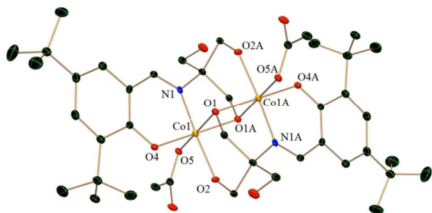
Fig. 1 Crystal structure of complex 1 with thermal ellipsoids at the 30% probability level. Hydrogen atoms and solvent molecules are omitted for clarity. Symmetry transformation: A = -x+1, -y, -z+1
