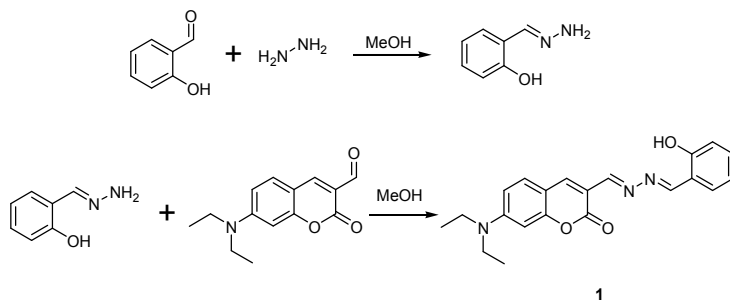
Scheme 1. Synthesis of chemosensor 1
