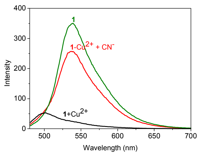
Fig. 9. Reversibility of the interaction between 1 and Cu 2+ by the introduction of CN - to the system.
