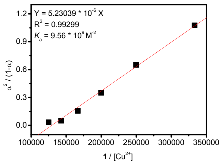
Fig. 5. The plot of chemosensor 1 with Cu 2+ in methanol/water v/v = 1:1, 10 mM hepes, pH 7.0) solution. The excitation wavelength was 467 nm and the observed wavelength was 537 nm.
