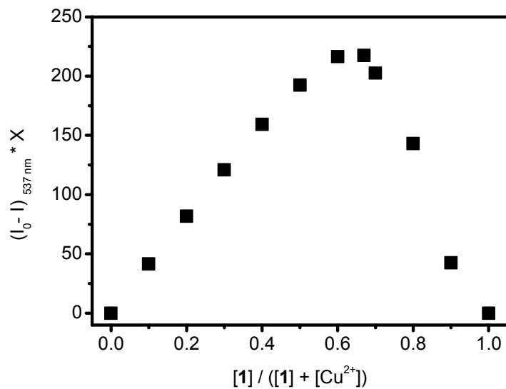
Fig. 4. Job plot of 1 -Cu 2+ complexes, where the emission intensity at 537 nm is plotted against mole fraction of 1 , at a constant total concentration of 2.0*10 -5 M in a methanol-water (v/v = 1:1, 10 mM hepes, pH 7.0) solutions.
