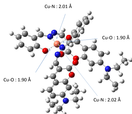
Fig. 7. DFT-optimized structures of \text{Cu}^{2+}\text{-1}_2 complexes calculated using the B3LYP/LanL2DZ method. (Red atom, O; blue atom, N; Orange atom, Cu).
