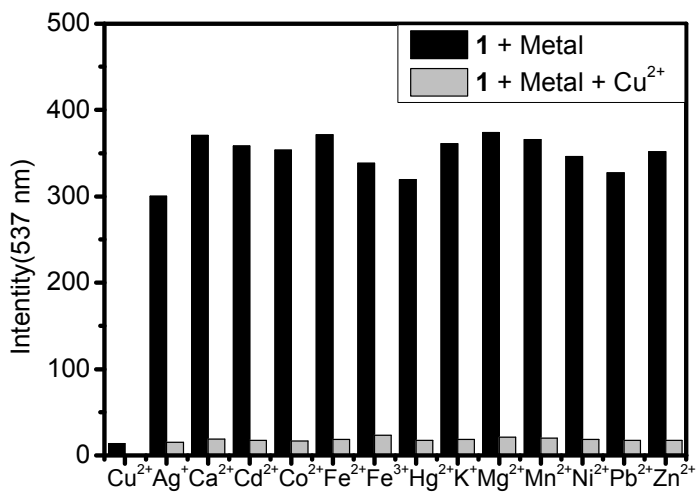
Fig. 3. Fluorescence response of 1 (10 μM) to Cu 2+ (20 μM) or 20 μM of other metal ions (the black bar) and to the mixture of other metal ions (20 μM) with 20 μM of Cu 2+ (the gray bar) in methanol-water (v/v = 1:1, 10 mM hepes, pH 7.0) solutions.
