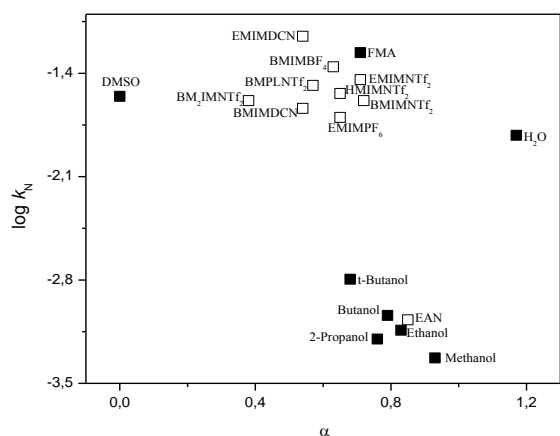
Figure 4. Plots of \log k_N for the reactions of DNBSCl with piperidine in a series of COS and RTILs against \alpha .
