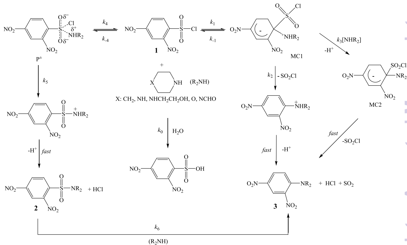
5 Scheme 1. Possible nucleophilic substitution reactions for DNBSCl towards Secondary Alicyclic amines.
