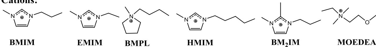
10 Scheme 2. Structures and acronyms of the RTILs used in this study.
