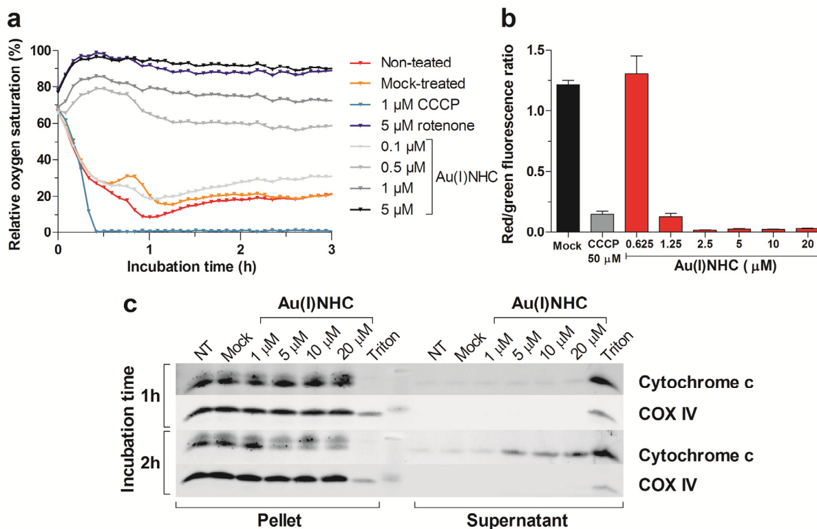
Figure 3 Effects of Au(I)NHC treatment on mitochondria. (a) Respiration of isolated mouse liver mitochondria depicted as a decrease of oxygen saturation over time. Mock-treated samples contained 0.1 % (v/v) DMF. CCCP (1 \mu M) was used as a positive control of the maximal oxygen consumption (0 % oxygen in the respiration buffer). The respiratory chain complex I inhibitor rotenone was used as a positive control of respiration inhibition (oxygen concentration close to 100%). (b) Mitochondrial membrane potential in Jurkat cells presented as JC-1 aggregated /JC-1 monomeric fluorescence ratio. Mock stands for mock-treated cells (0.1 % (v/v) DMF). The proton uncoupling reagent CCCP (50 \mu M) was used as a positive control. (c) Cytochrome c release from isolated mouse liver mitochondria. Mock-treated samples contained 0.1 % (v/v) DMF. Triton X-100 (1% (v/v)) was used as a positive control for outer membrane permeabilization. Cytochrome c oxidase subunit IV (COX IV) detection was used as a control of protein loading and as an indicator for the intactness of the inner mitochondrial membrane.
