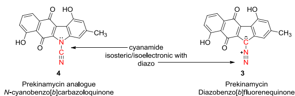
Figure 3: Prekinamycin 3 and the corresponding cyanamide analogue of prekinamycin 4 .
