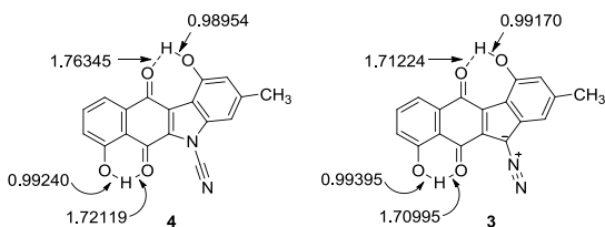
Figure 6: Bond lengths (Å) as observed in the minimized structures of 4 and 3 obtained at the DFT B3LYP 6-31 G(d) level of theory.
