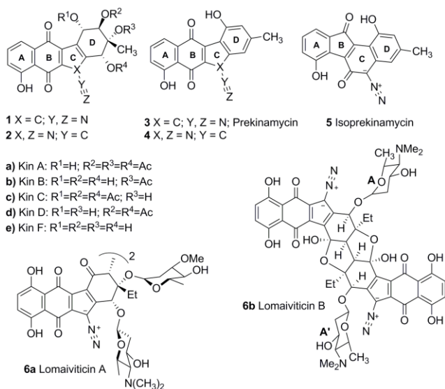
Figure 1: Representative members of the kinamycins and lomaiviticins.
