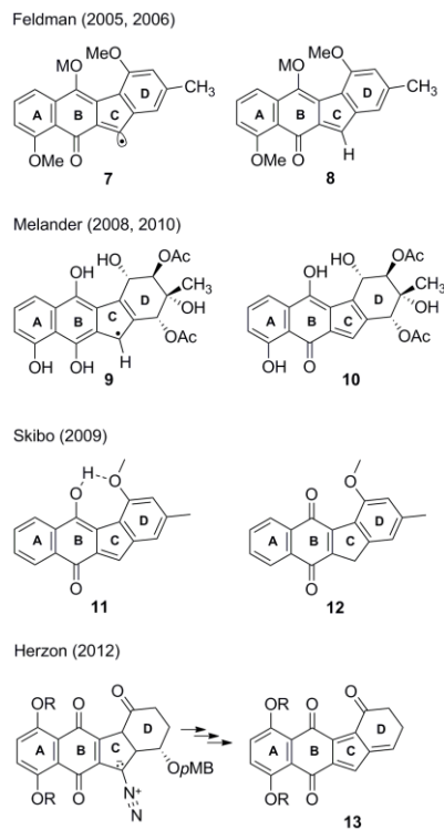
Figure 2: Possible reactive intermediates.
