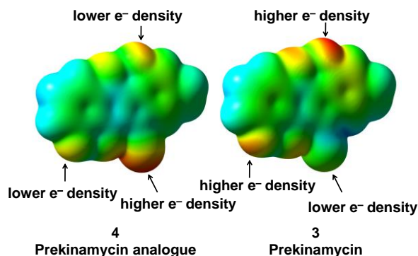
Figure 5: The electrostatic potential energy (ESP) surfaces of 4 and 3 generated at the DFT B3LYP 6-31 G(d) level of theory (isoval 0.0004) and range from ±30.8 kcal·mol -1 for 4 and ±26.3 kcal·mol -1 for 3 . Regions coloured red indicate negative ESP values and regions coloured blue indicate positive values of the ESP with green being zero ESP.
