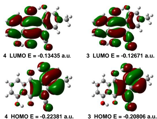
Figure 4: The HOMO, LUMO and their corresponding energy levels (eigenvalues) of cyanamide 4 and prekinamycin 3 generated at the DFT B3LYP 6-31 G(d) level of theory (1 a.u. = 627.5095 kcal mol -1 ).
