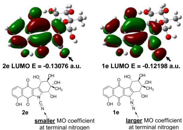
Figure 7: The LUMO and their corresponding energy levels (eigenvalues) of kinamycin F 1e and its hypothetical cyanamide analogue 2e generated at the DFT B3LYP 6-31 G(d) level (1 a.u. = 627.5095 kcal·mol -1 ).
