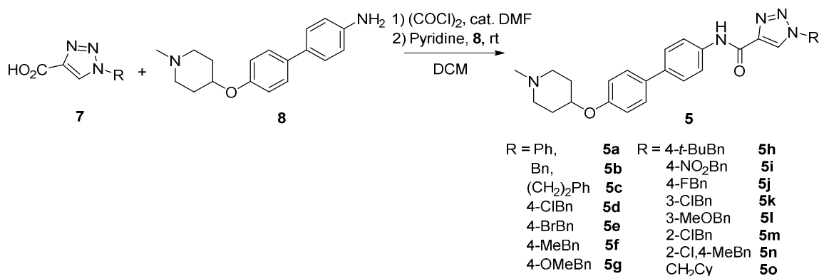
Scheme 3. Synthesis of biphenyl triazole derivatives 5 .
