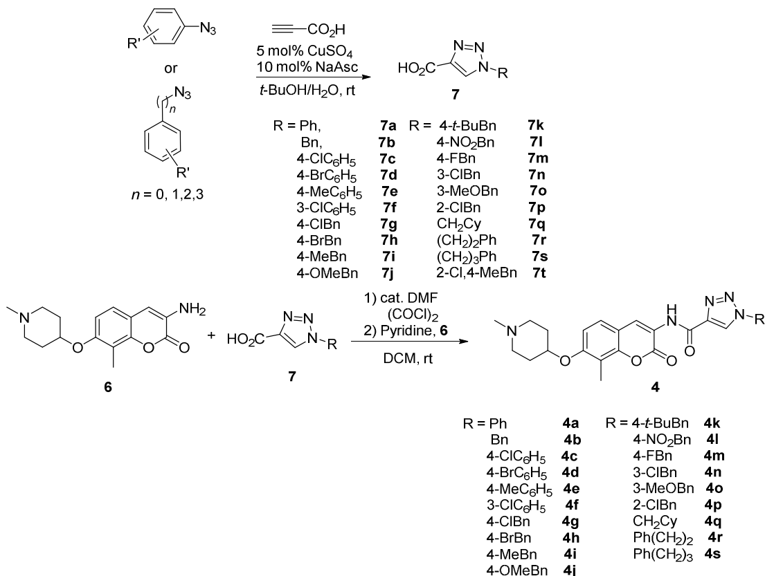
Scheme 2. Synthesis of triazole containing coumarin derivatives.
