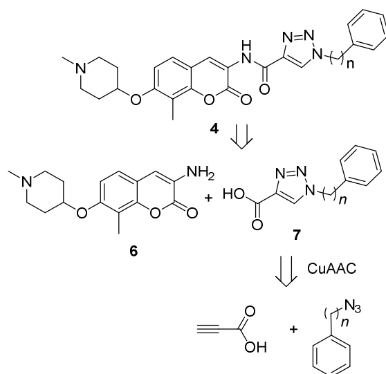
Scheme 1. Retrosynthetic analysis of the triazole 4 .
