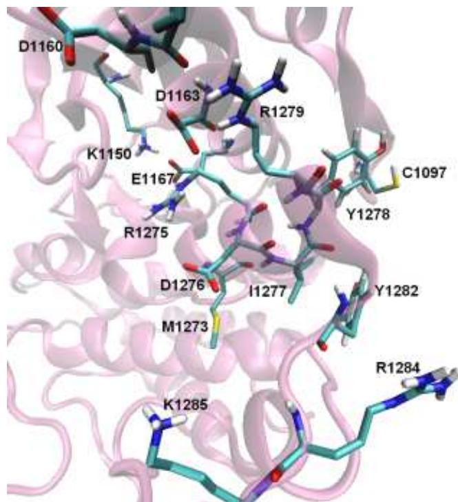
Figure 4 Interactions between the aminoacid residues in the \alpha C- and \alpha A-helices.
