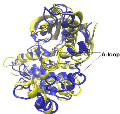
Figure 5 Superimposed MD-averaged and crystal structures of ALK. The MD structure is in blue and the crystal structure is in yellow.
