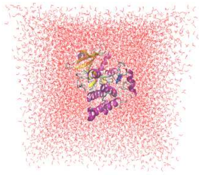
Figure 2. Solvated and neutralized system for MD simulations
