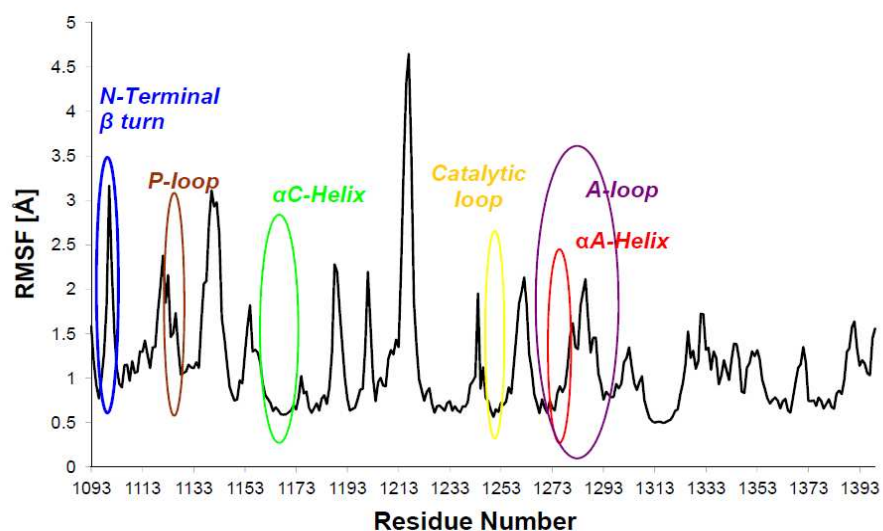
Figure 3. RMSF Values of the wild type free enzyme
