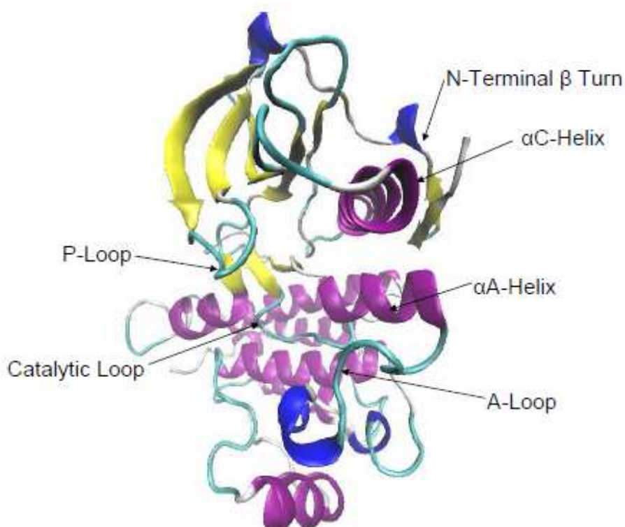
Figure 1 Structure of ALK (3L9P.pdb 7 ). The \alpha -helices are shown in purple, the \beta -sheets are shown in yellow, and the 3-10 helices are shown in blue, the loops are shown in cyan and the coils in white shown in red.
