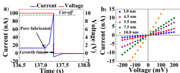
Fig. 2 (a) Leakage current through the \text{SiN}_x membrane a few seconds before nanopore fabrication by CBD at 10 V. The instant of nanopore fabrication is characterized by a sudden increase in current. (b) Current-voltage (I-V) curves used to infer nanopore diameter using a conductance-based model for 5 independently fabricated nanopores on a single five-channel device.
