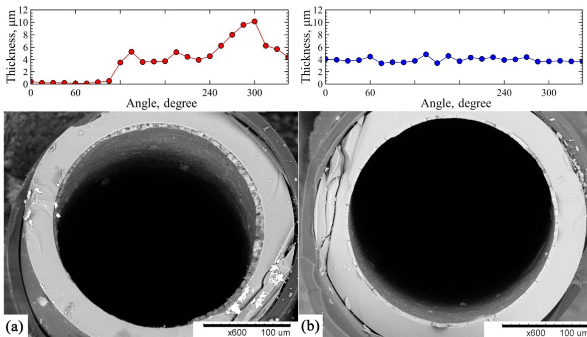
Fig. 5. Cross-sectional SEM images of the capillaries coated at (a) 0.2 mm/s, (b) 5 mm/s and the coating thickness as a function of angular position.
