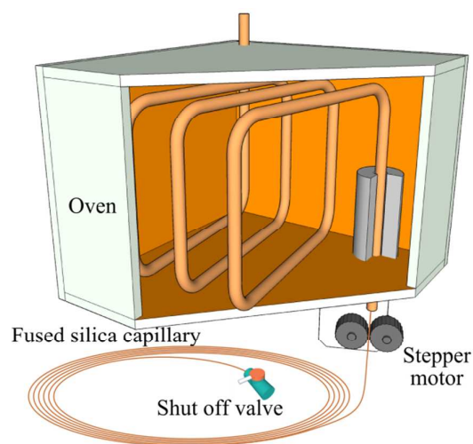
Fig. 2. Schematic view of the coating apparatus.
