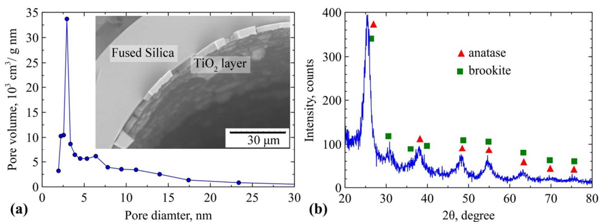
Fig. 4. (a) PSD of the \text{TiO}_2 coatings, (insert) SEM image of the cross-section of the titania coated 250 \mu\text{m} capillary, and (b) the PXRD pattern of the coating.
