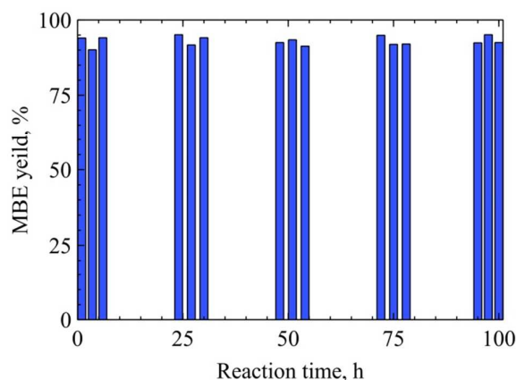
Fig. 9. Long-term stability of the capillary microreactor with Pd-Bi/TiO 2 in MBY semihydrogenation (1200 mol/m 3 MBY in hexane flow 42.5 \mu\text{L}/\text{min} , 10 mL/min (STP) H 2 flow, 335K).
