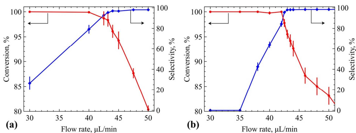
Fig. 8. Summary of the performance of the capillary microreactor with Pd-Bi/TiO 2 in MBY semihydrogenation ( 1200 \text{ mol}/\text{m}^3 MBY in hexane, 10 mL/min (STP) H 2 flow, (a) 310 K and (b) 335 K). Selectivity is calculated towards MBE.
