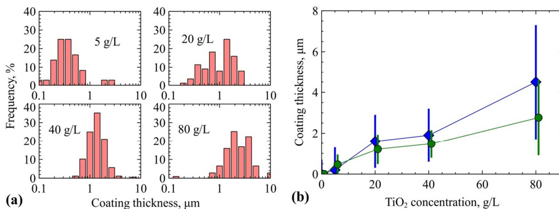
Fig. 6. (a) Distribution of the \text{TiO}_2 coating thickness obtained in the 250\ \mu\text{m} fused silica capillaries using different precursor sol concentrations. Displacement speed: 0.2\ \text{mm/s} . Oven temperature: 450\ \text{K} . (b) The comparison of the average coating thickness determined by (●) SEM and (◆) hydrodynamic study.
