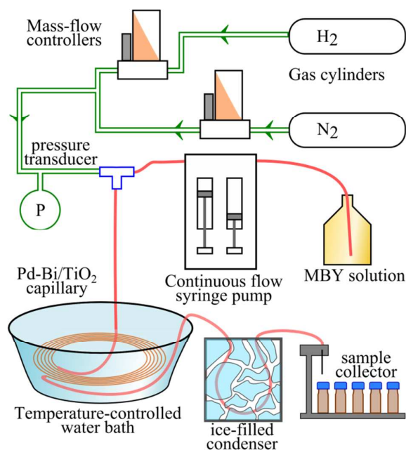
Fig. 3. Scheme of the hydrogenation apparatus
