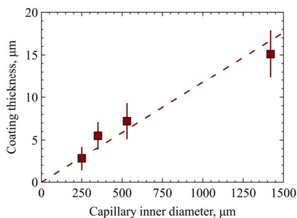
Fig. 7. Effect of the capillary inner diameter on the coating thickness (SEM data) using a 80\ \text{g/L} \text{TiO}_2 sol.
