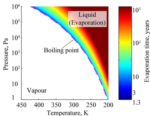
Fig. 1. Effect of temperature and pressure on the evaporation time of the 5-m long reactor filled with ethanol, estimated using Stefan's equation. 33
