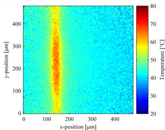
Figure 2: FLIM thermograph of the microwire array with 2 W of electrical power applied to the two left vertical wires (frame similar to Figure 1c).
