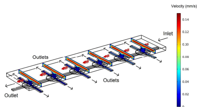
Figure 2 An overview of the velocity contours for a part of the VIA device obtained from 3D CFD simulations.
