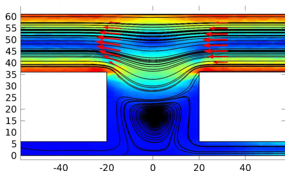
Figure 3 shows the CFD generated flow profiles across the device (in cross-section), demonstrating that cells within 5-10 \mu\text{m} of the bottom surface experience little shear-stress. Dimensions in microns, shear stress colour scale from 0 Pa (blue) to 0.04 Pa (orange).
