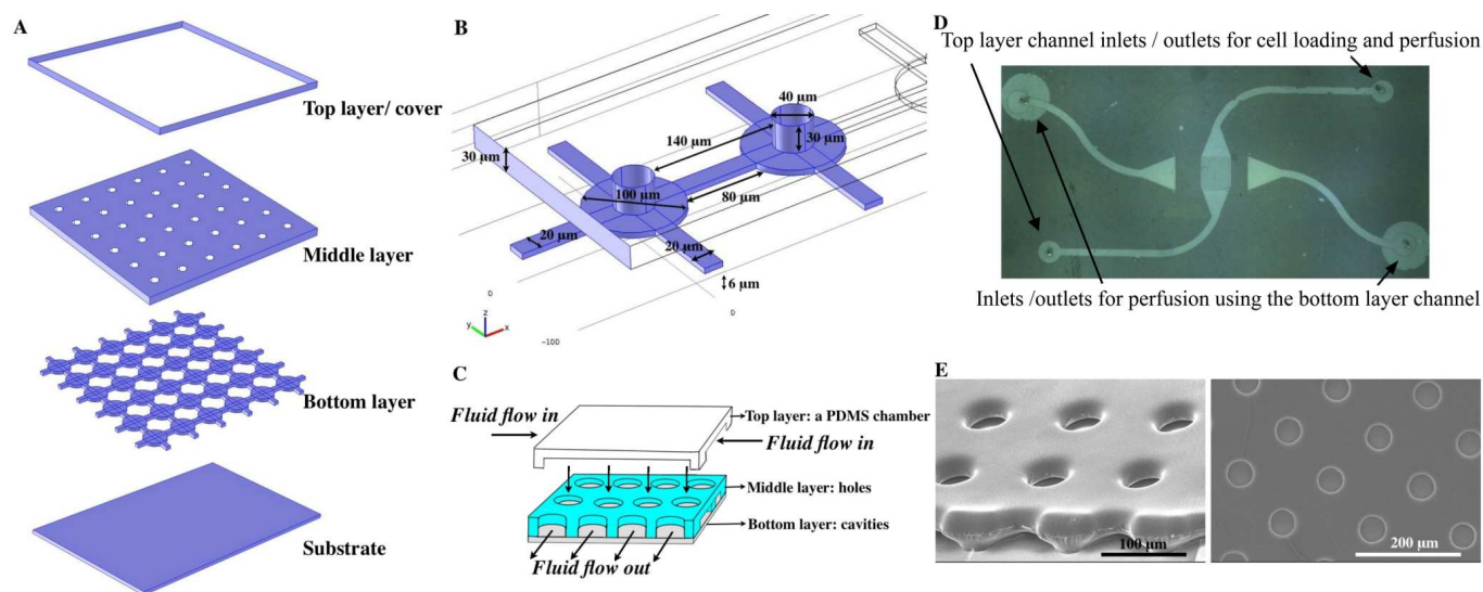
Figure 1 Illustration of the multi-layered VIA device (A) composed of three layers (the upper layer comprises a PDMS chamber, the middle layer has an array of circular holes and the bottom layer has 100 \mu\text{m} circular cavities, linked together by 20 \times 80 \times 6 \mu\text{m} channels). The substrate is typically a glass microscope slide or coverslip (the latter for ease of cell observation). (B) The detail of the geometry of the VIA devices. (C) The cartoon shows composition of the devices and flow direction. (D) Top view of the VIA array comprising fluid inlets and outlets and an observation area (centre) with an array of holes. (E) SEM images of the VIA devices (viewed from the side (left) and from the top view (right)).
