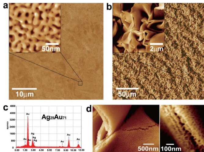
Fig. 8 Shrinkage of nanoporous thin films result in nanostructures for SERS effects. 101 SEM images of a) flat nanoporous films and b) features arising from shrinking nanoporous thin films. c) Chemical composition of the thin films. d) SEM image showing nanogaps hot spots for SERS effects. Adapted from H. W. Liu, L. Zhang, X. Y. Lang, Y. Yamaguchi, H. S. Iwasaki, Y. S. Inouye, Q. K. Xue and M. W. Chen, Sci Rep-Uk , 2011, 1 with permission from Nature Publishing Group.
